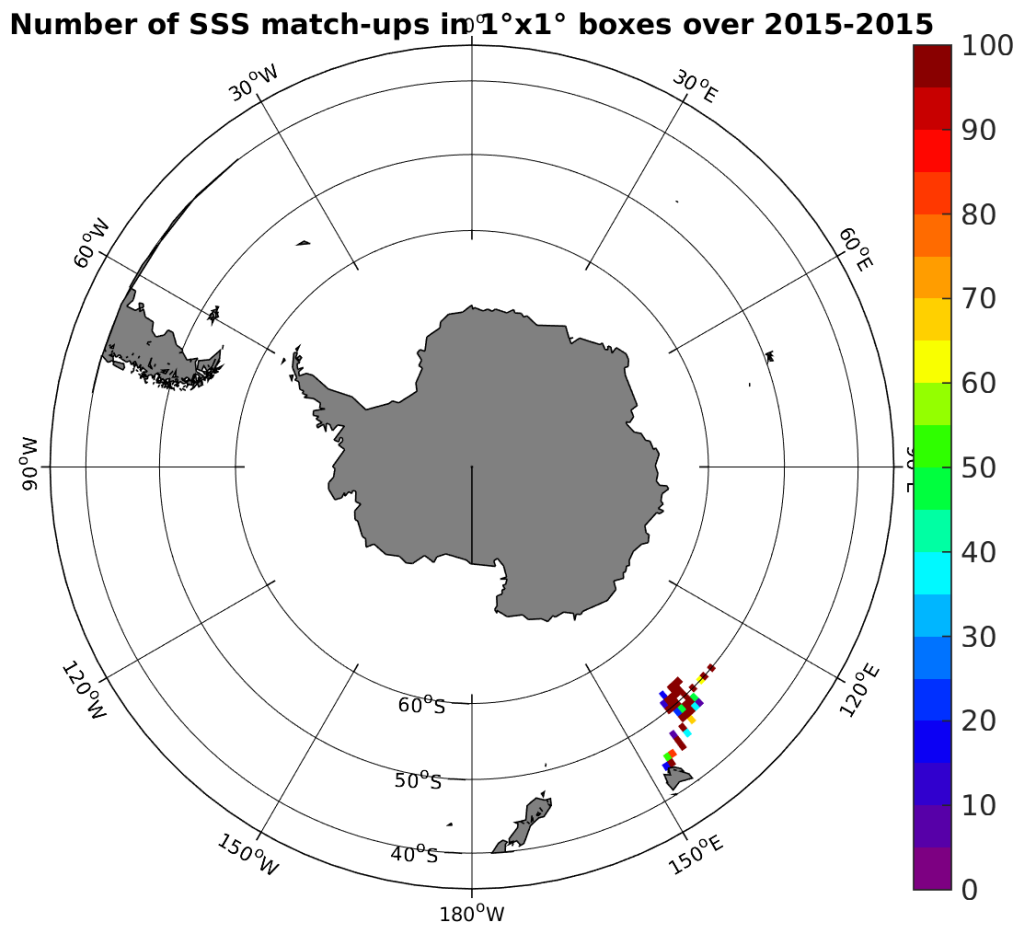
Figure 4: Number of SSS match-ups between TSG-GOSUD-Research-vessel SSS and the AQUARIUS-L2-JPL-V4 SSS product for the Roaring Forties and Furious Fifties Pi-MEP region over 1^\circ \times 1^\circ boxes and for the full satellite product period.
