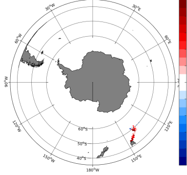
(e) MEAN( \Delta SSS) (Satellite - TSG-GOSUD-Research-vessel)
