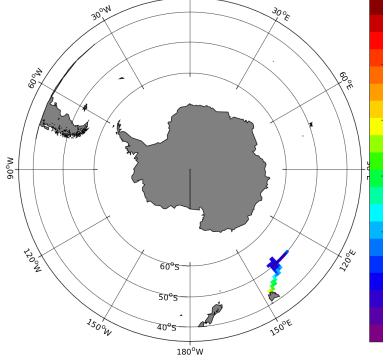
(c) MEAN(TSG-GOSUD-Research-vessel SSS)
