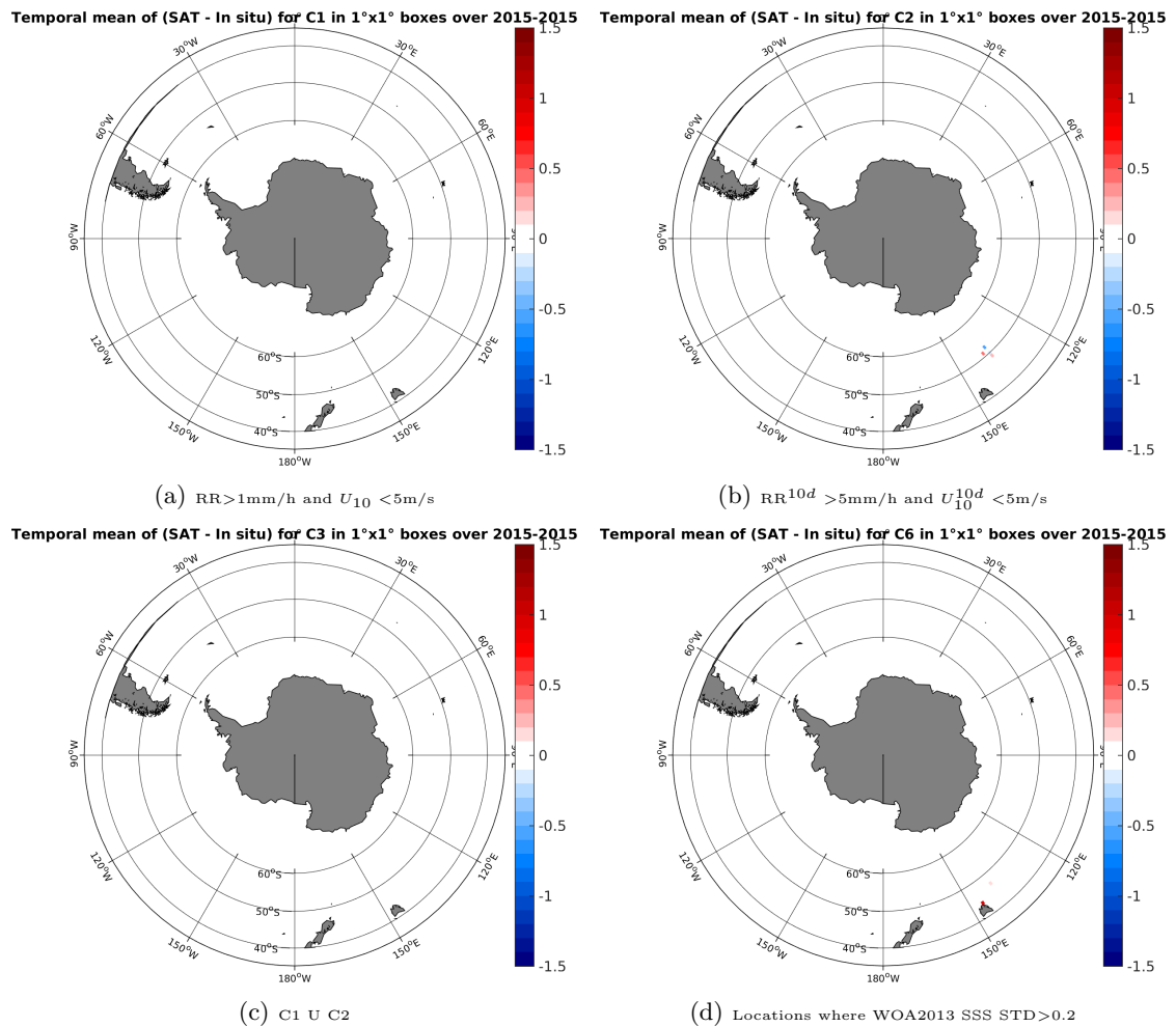
Figure 12: Temporal mean gridded over spatial boxes of size 1^\circ \times 1^\circ of \Delta SSS (AQUARIUS-L2-JPL-V4 - TSG-GOSUD-Research-vessel) for 4 different subdatasets corresponding to: RR > 1\text{mm/h} and U_{10} < 5\text{m/s} (a), RR^{10d} > 5\text{mm/h} and U_{10}^{10d} < 5\text{m/s} (b), C1 U C2 (c), Locations where WOA2013 SSS STD > 0.2 (d).
