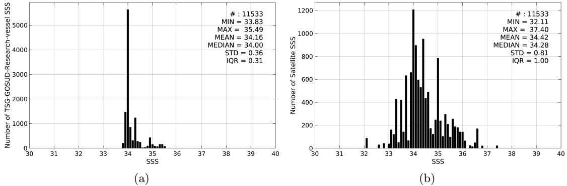
Figure 2: Histograms of SSS from TSG-GOSUD-Research-vessel (a) and AQUARIUS-L2-JPL-V4 (b) considering all match-up pairs per bins of 0.1 over the Roaring Forties and Furious Fifties Pi-MEP region and for the full satellite product period.
