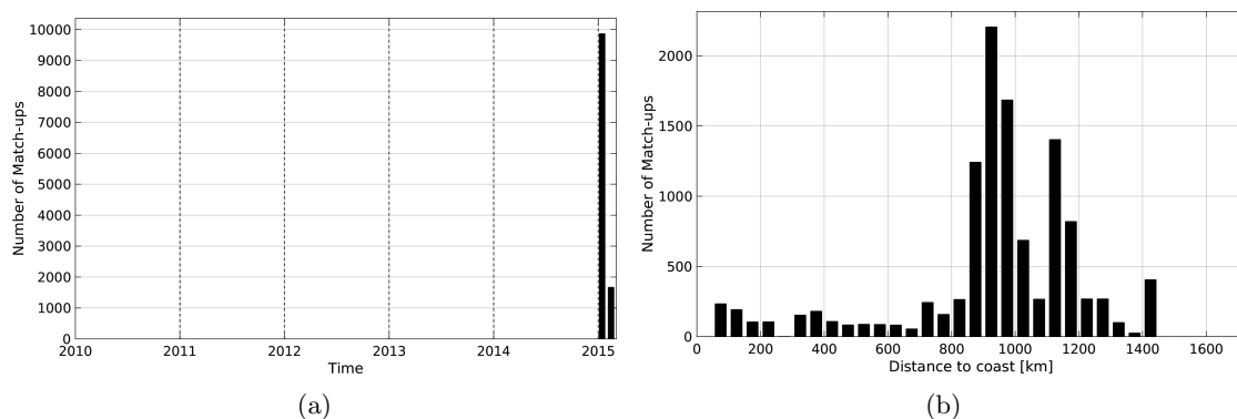
Figure 1: Number of match-ups between TSG-GOSUD-Research-vessel and AQUARIUS-L2-JPL-V4 SSS as a function of time (a) and as function of the distance to coast (b) over the Roaring Forties and Furious Fifties Pi-MEP region and for the full satellite product period.
