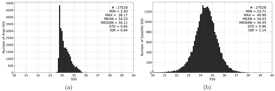
Figure 2: Histograms of SSS from Argo (a) and AQUARIUS-L2-JPL-V4 (b) considering all match-up pairs per bins of 0.1 over the Roaring Forties and Furious Fifties Pi-MEP region and for the full satellite product period.
