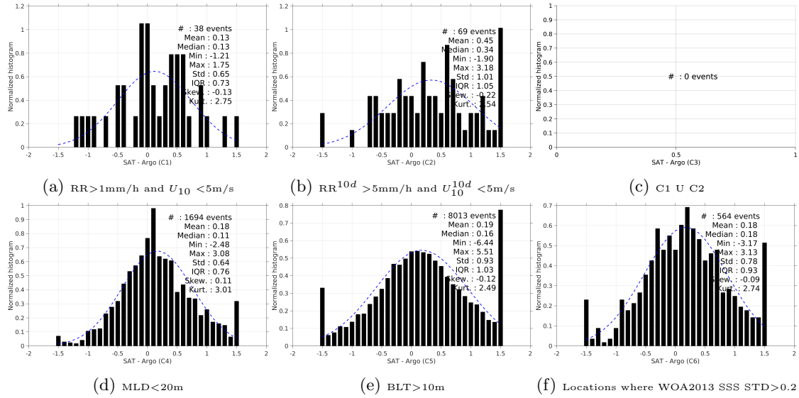
Figure 13: Normalized histogram of \Delta SSS (AQUARIUS-L2-JPL-V4 - Argo) for 6 different sub-datasets corresponding to: RR>1mm/h and U_{10} < 5\text{m/s} (a), RR^{10d} > 5\text{mm/h} and U_{10}^{10d} < 5\text{m/s} (b), C1 U C2 (c),MLD<20m (d),BLT>10m (e),Locations where WOA2013 SSS STD>0.2 (f).
