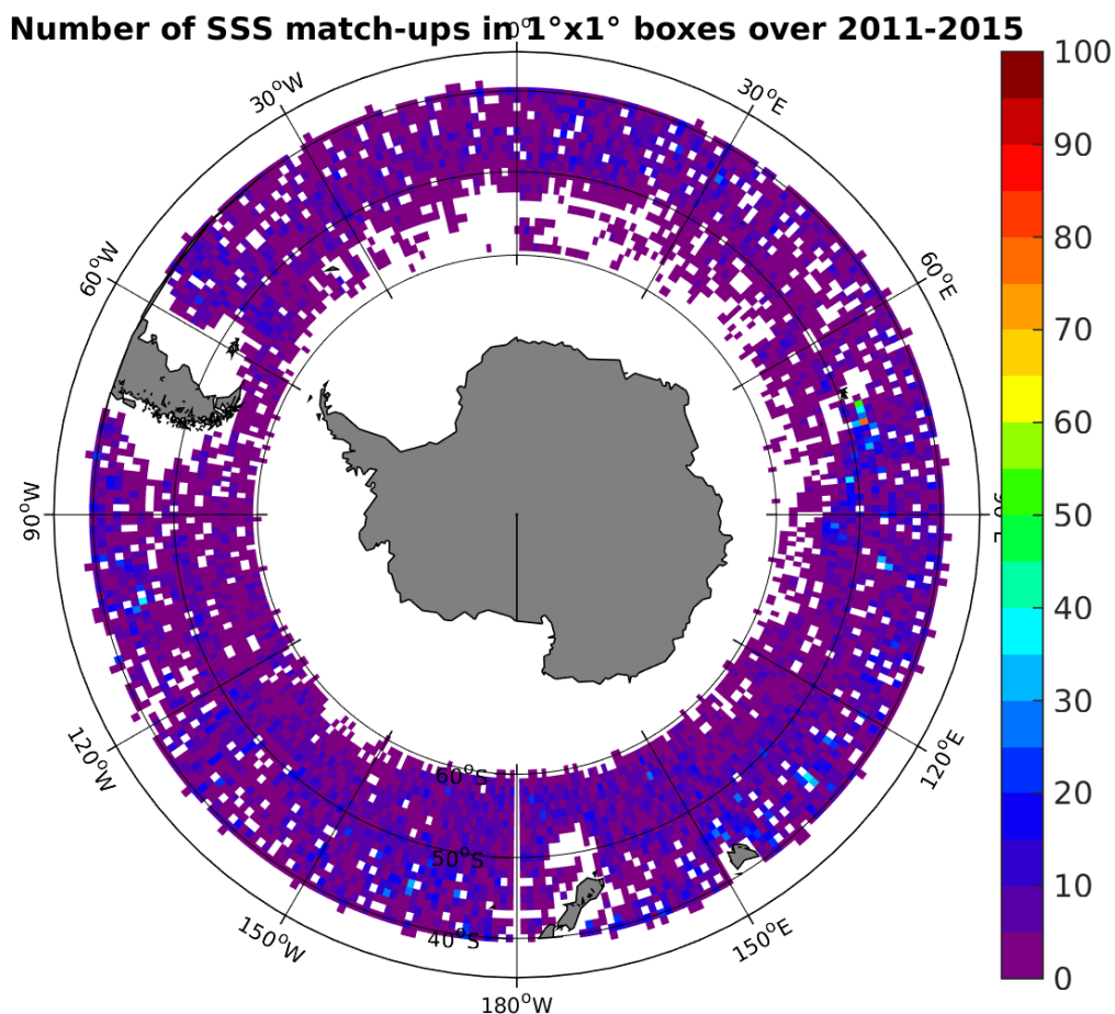
Figure 4: Number of SSS match-ups between Argo SSS and the AQUARIUS-L2-JPL-V4 SSS product for the Roaring Forties and Furious Fifties Pi-MEP region over 1^\circ \times 1^\circ boxes and for the full satellite product period.
