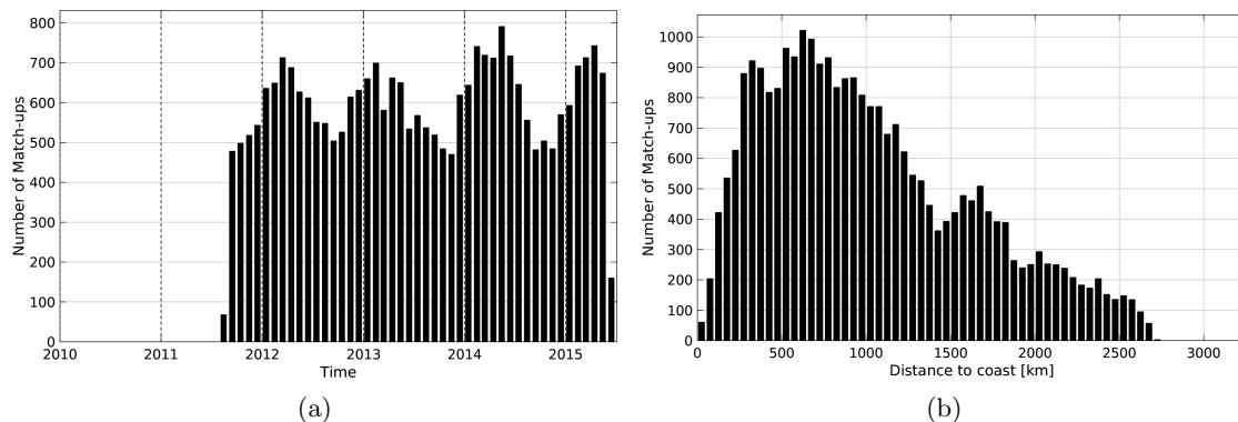
Figure 1: Number of match-ups between Argo and AQUARIUS-L2-JPL-V4 SSS as a function of time (a) and as function of the distance to coast (b) over the Roaring Forties and Furious Fifties Pi-MEP region and for the full satellite product period.
