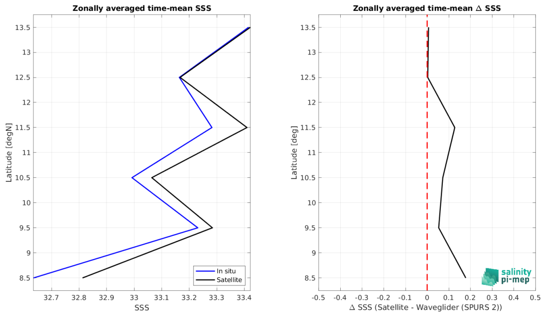
Figure 8: Left panel: Zonal mean SSS from SMOS SSS L4 v1 - Weekly (CMEMS-CNR) satellite product (black) and from Waveglider (SPURS 2) (blue). Right panel: Zonal mean of \Delta SSS (Satellite - Waveglider (SPURS 2)) for all the collected Pi-MEP match-up pairs estimated over the full satellite product period.
