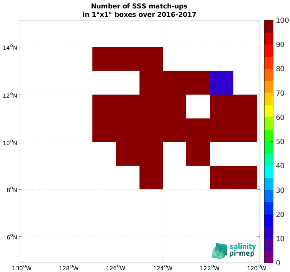
Figure 4: Number of SSS match-ups between Waveglider (SPURS 2) SSS and the SMOS SSS L4 v1 - Weekly (CMEMS-CNR) SSS product for the SPURS 2 Pi-MEP region over 1^\circ \times 1^\circ boxes and for the full satellite product period.
