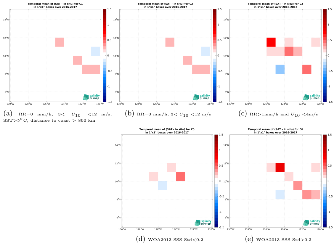
Figure 12: Temporal mean gridded over spatial boxes of size 1^\circ \times 1^\circ of \Delta SSS (SMOS SSS L4 v1 - Weekly (CMEMS-CNR) - Waveglider (SPURS 2)) for 5 different subdatasets corresponding to:RR=0 mm/h, 3 < U_{10} < 12 m/s, SST >5^\circ C, distance to coast > 800 km (a), RR=0 mm/h, 3 < U_{10} < 12 m/s (b), RR >1 mm/h and U_{10} < 4 m/s (c), WOA2013 SSS Std <0.2 (d), WOA2013 SSS Std >0.2 (e).
