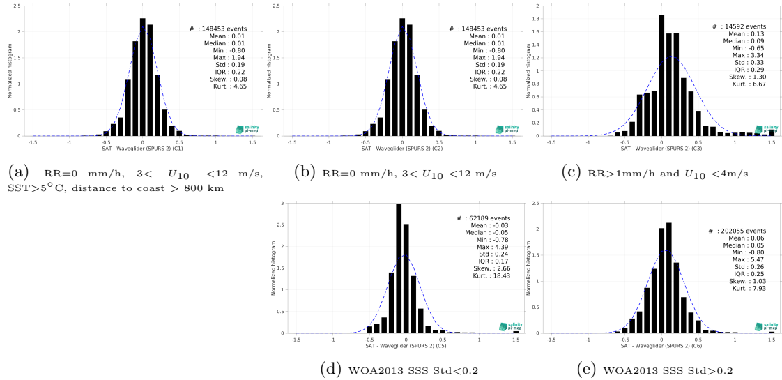
Figure 13: Normalized histogram of \Delta SSS (SMOS SSS L4 v1 - Weekly (CMEMS-CNR) - Waveglider (SPURS 2)) for 5 different subdatasets corresponding to: RR=0 mm/h, 3 < U_{10} < 12 m/s, SST > 5°C, distance to coast > 800 km (a), RR=0 mm/h, 3 < U_{10} < 12 m/s (b), RR > 1mm/h and U_{10} < 4 m/s (c), WOA2013 SSS Std < 0.2 (d), WOA2013 SSS Std > 0.2 (e).
