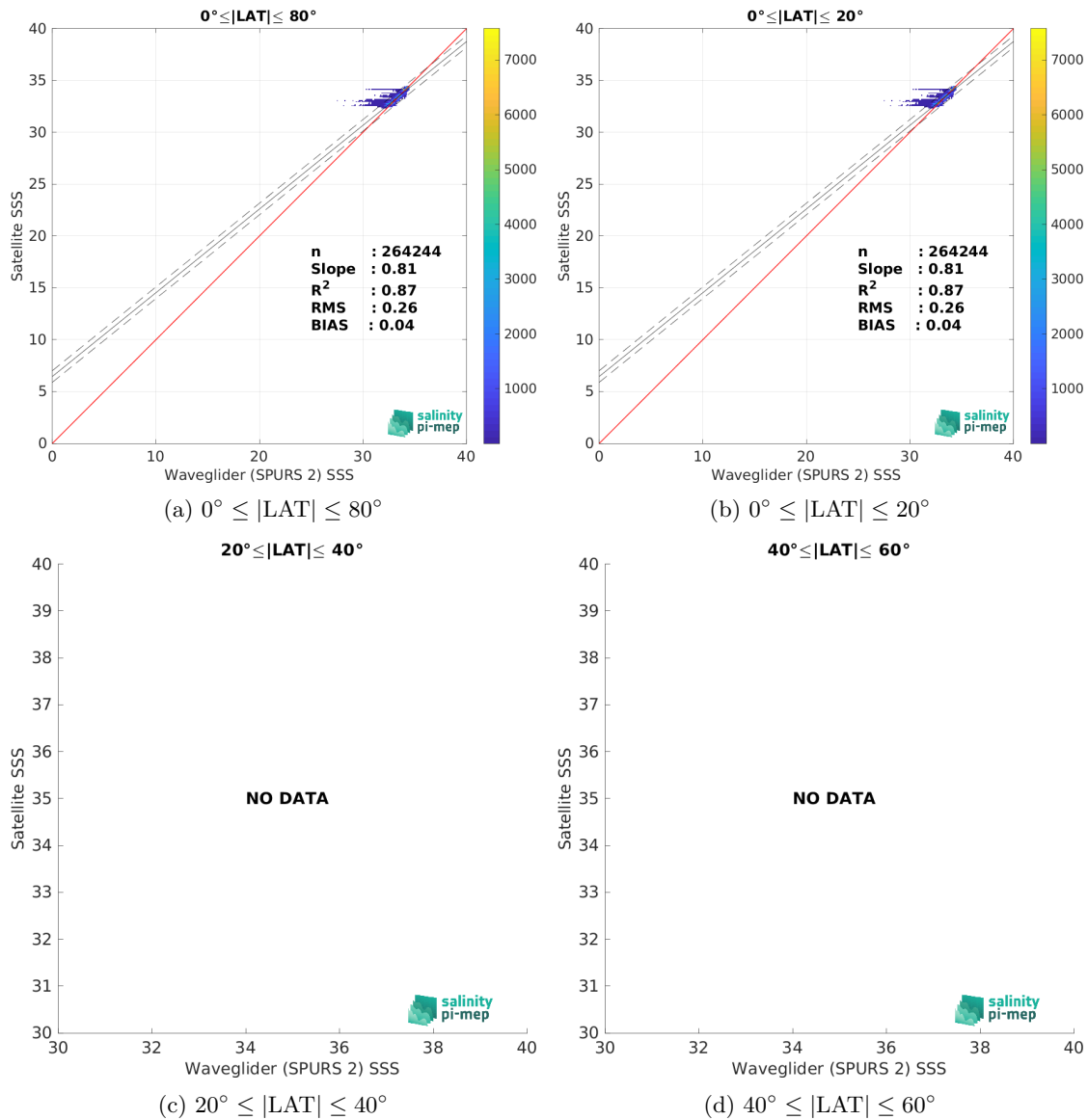
Figure 9: Contour maps of the concentration of SMOS SSS L4 v1 - Weekly (CMEMS-CNR) SSS (y-axis) versus Waveglider (SPURS 2) SSS (x-axis) at match-up pairs for different latitude bands. For each plot, the red line shows x=y . The black thin and dashed lines indicate a linear fit through the data cloud and the \pm 95\% confidence levels, respectively. The number match-up pairs n , the slope and R^2 coefficient of the linear fit, the root mean square (RMS) and the mean bias between satellite and in situ data are indicated for each latitude band in each plots.
