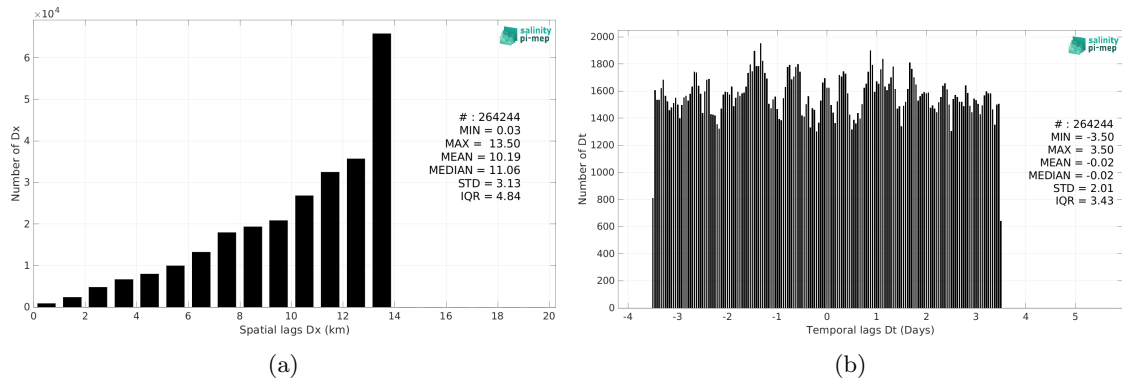
Figure 5: Histograms of the spatial (a) and temporal (b) lags between the location/time of the Waveglider (SPURS 2) measurement and the date of the corresponding SMOS SSS L4 v1 - Weekly (CMEMS-CNR) SSS pixel.
