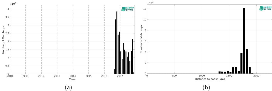
Figure 1: Number of match-ups between Waveglider (SPURS 2) and SMOS SSS L4 v1 - Weekly (CMEMS-CNR) SSS as a function of time (a) and as function of the distance to coast (b) over the SPURS 2 Pi-MEP region and for the full satellite product period.
