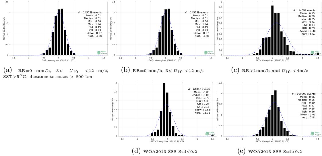
Figure 13: Normalized histogram of \Delta\text{SSS} (SMOS SSS L4 v1 - Weekly (CMEMS-CNR) - Waveglider (SPURS 2)) for 5 different subdatasets corresponding to: RR=0 mm/h, 3 < U_{10} < 12 m/s, SST>5°C, distance to coast > 800 km (a), RR=0 mm/h, 3 < U_{10} < 12 m/s (b), RR>1mm/h and U_{10} < 4 m/s (c), WOA2013 SSS Std<0.2 (d), WOA2013 SSS Std>0.2 (e).
