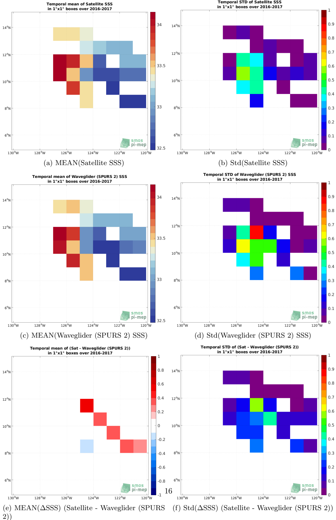
Figure 6: Temporal mean (left) and Std (right) of SSS from SMOS SSS L4 v1 - Weekly (CMEMS-CNR) (top), Waveglider (SPURS 2) (middle), and of \Delta SSS (Satellite - Waveglider (SPURS 2)). Only match-up pairs are used to generate these maps.
