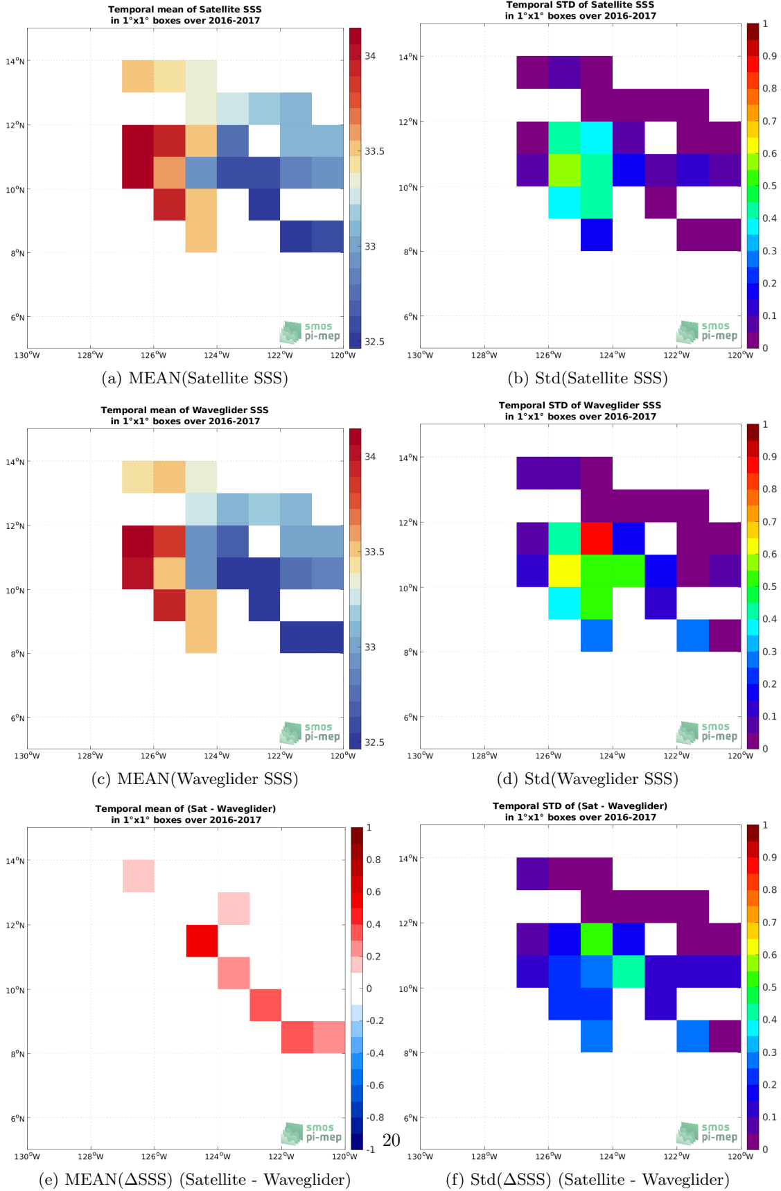
Figure 5: Temporal mean (left) and Std (right) of SSS from SMOS SSS L4 v1 - Weekly (CMEMS-CNR) (top), Waveglider (middle), and of \Delta SSS (Satellite - Waveglider). Only match-up pairs are used to generate these maps.
