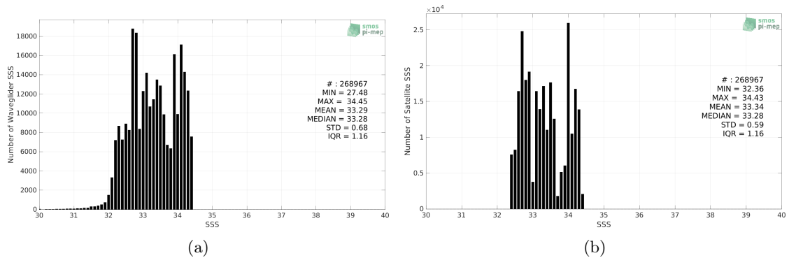
Figure 2: Histograms of SSS from Waveglider (a) and SMOS SSS L4 v1 - Weekly (CMEMS-CNR) (b) considering all match-up pairs per bins of 0.1 over the SPURS 2 Pi-MEP region and for the full satellite product period.
