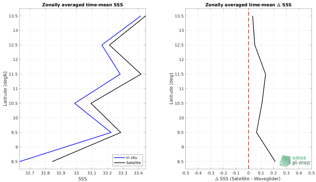
Figure 7: Left panel: Zonal mean SSS from SMOS SSS L4 v1 - Weekly (CMEMS-CNR) satellite product (black) and from Waveglider (blue). Right panel: Zonal mean of \Delta SSS (Satellite - Waveglider) for all the collected Pi-MEP match-up pairs estimated over the full satellite product period.
