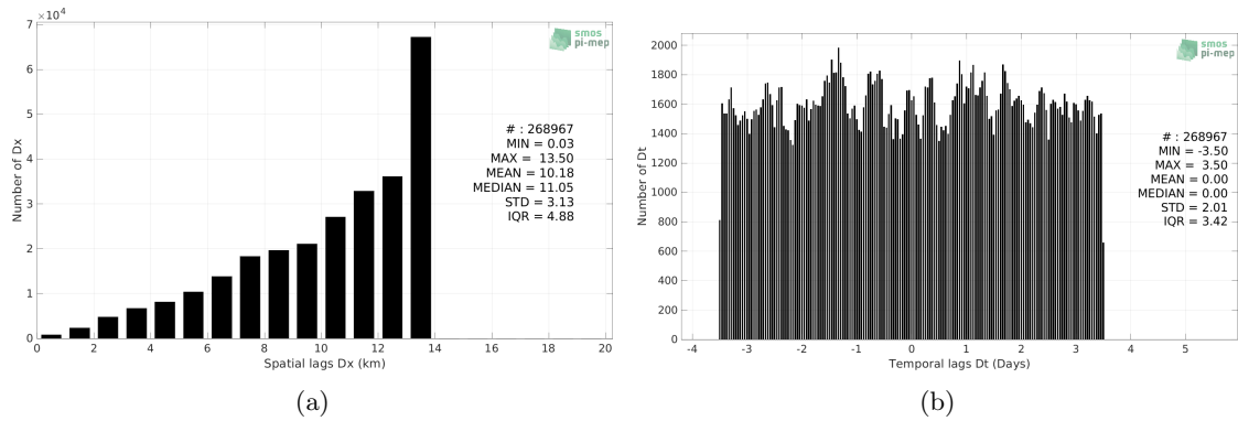
Figure 4: Histograms of the spatial (a) and temporal (b) lags between the location/time of the Waveglider measurement and the date of the corresponding SMOS SSS L4 v1 - Weekly (CMEMS-CNR) SSS pixel.
