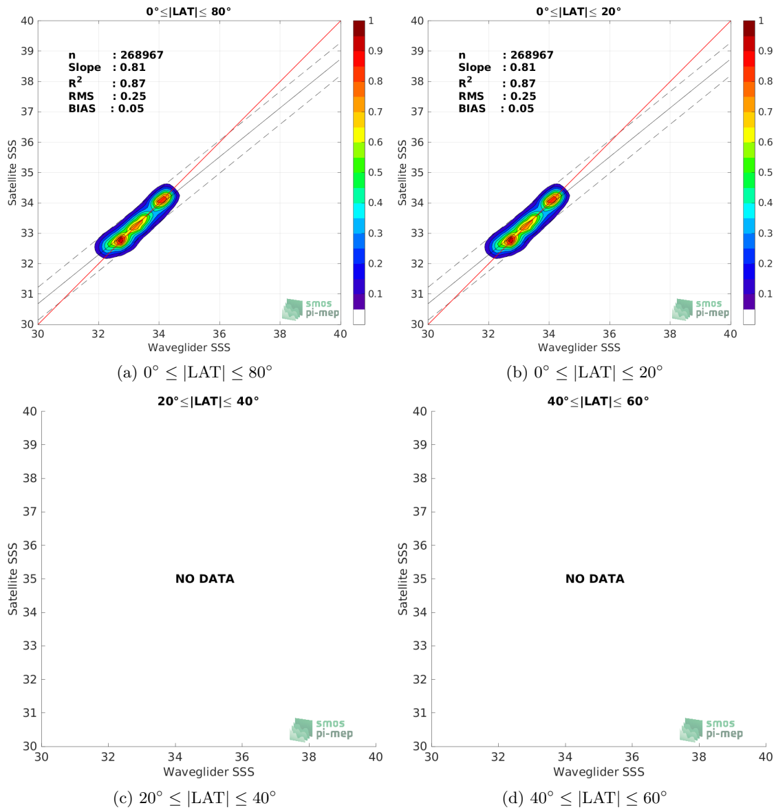
Figure 8: Contour maps of the concentration of SMOS SSS L4 v1 - Weekly (CMEMS-CNR) SSS (y-axis) versus Waveglider SSS (x-axis) at match-up pairs for different latitude bands. For each plot, the red line shows x=y . The black thin and dashed lines indicate a linear fit through the data cloud and the \pm 95\% confidence levels, respectively. The number match-up pairs n , the slope and R^2 coefficient of the linear fit, the root mean square (RMS) and the mean bias between satellite and in situ data are indicated for each latitude band in each plots.
