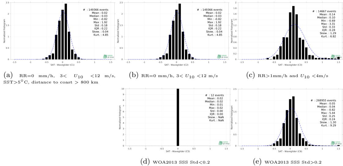
Figure 12: Normalized histogram of \Delta SSS (SMOS SSS L4 v1 - Weekly (CMEMS-CNR) - Waveglider) for 5 different subdatasets corresponding to: RR=0 mm/h, 3 < U_{10} < 12 m/s, SST > 5°C, distance to coast > 800 km (a), RR=0 mm/h, 3 < U_{10} < 12 m/s (b), RR > 1mm/h and U_{10} < 4 m/s (c), WOA2013 SSS Std < 0.2 (d), WOA2013 SSS Std > 0.2 (e).
