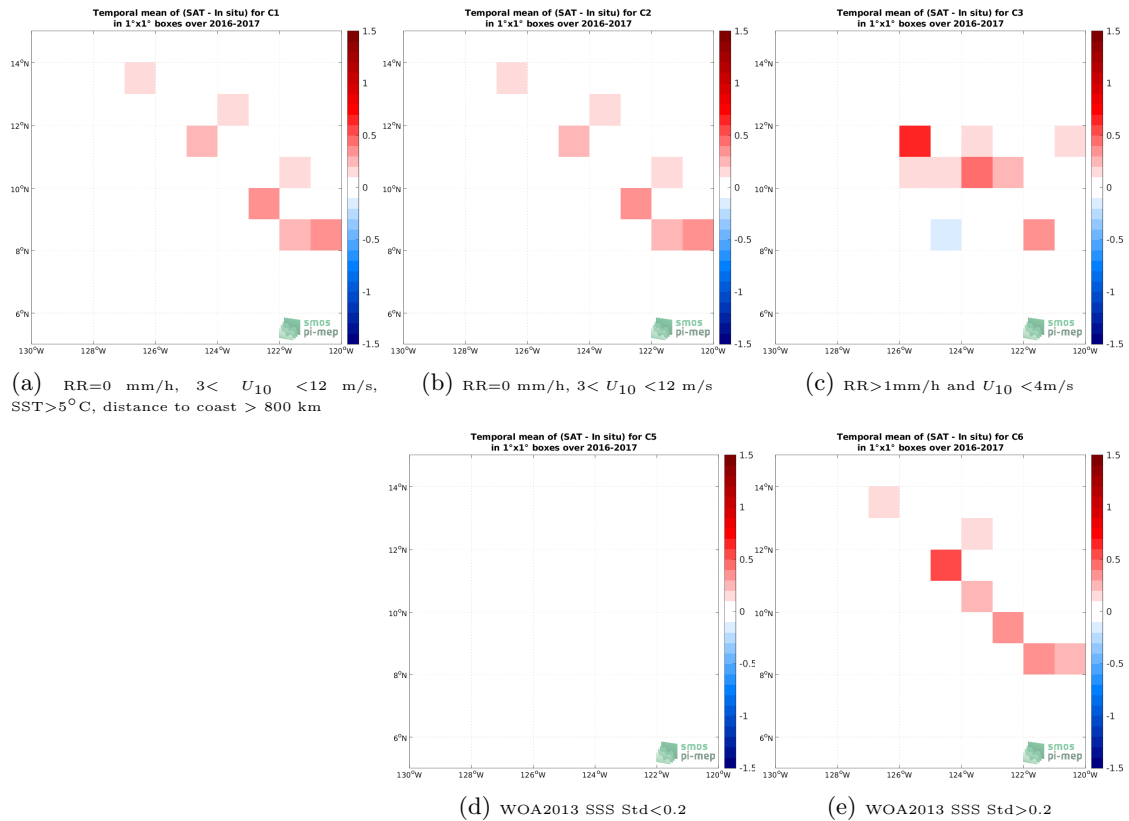
Figure 11: Temporal mean gridded over spatial boxes of size 1^\circ \times 1^\circ of \Delta\text{SSS} (SMOS SSS L4 v1 - Weekly (CMEMS-CNR) - Waveglider) for 5 different subdatasets corresponding to:RR=0 mm/h, 3 < U_{10} < 12 m/s, SST >5^\circ\text{C} , distance to coast > 800 km (a), RR=0 mm/h, 3 < U_{10} < 12 m/s (b), RR >1 mm/h and U_{10} < 4 m/s (c), WOA2013 SSS Std <0.2 (d), WOA2013 SSS Std >0.2 (e).
