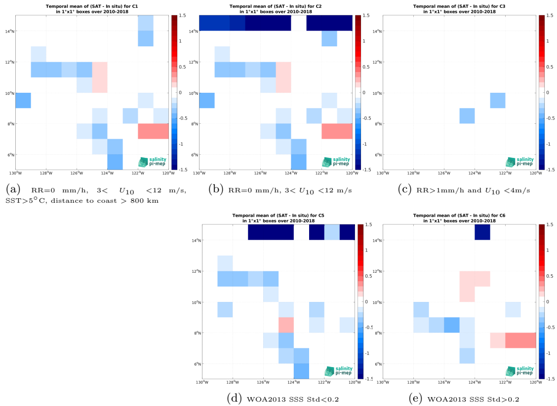
Figure 12: Temporal mean gridded over spatial boxes of size 1^\circ \times 1^\circ of \Delta\text{SSS} (SMOS SSS L4 v1 - Weekly (CMEMS-CNR) - TSG (SAMOS)) for 5 different subdatasets corresponding to:RR=0 mm/h, 3 < U_{10} < 12 m/s, SST >5^\circ\text{C} , distance to coast > 800 km (a), RR=0 mm/h, 3 < U_{10} < 12 m/s (b), RR >1 mm/h and U_{10} < 4 m/s (c), WOA2013 SSS Std <0.2 (d), WOA2013 SSS Std >0.2 (e).
