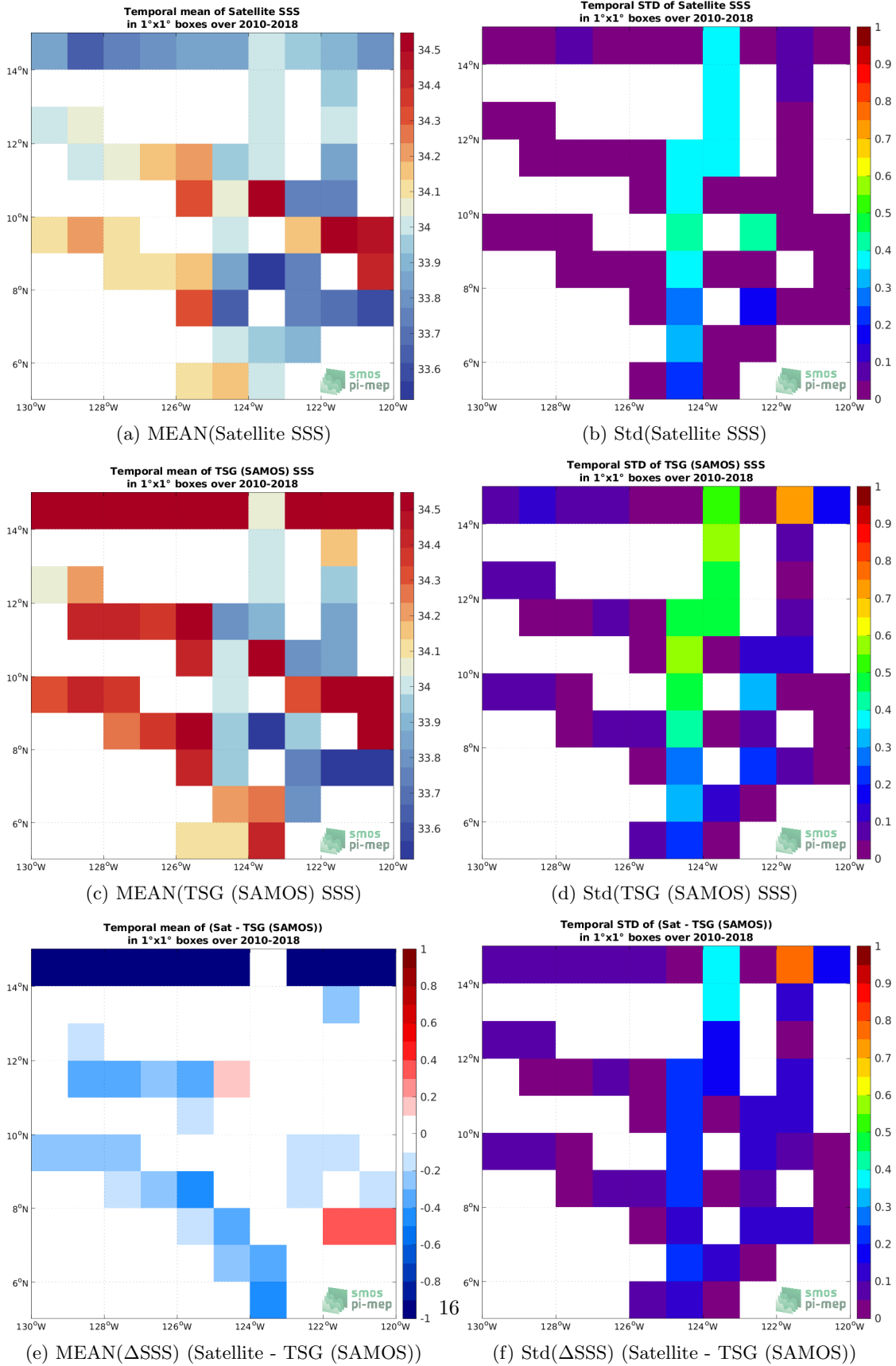
Figure 6: Temporal mean (left) and Std (right) of SSS from SMOS SSS L4 v1 - Weekly (CMEMS-CNR) (top), TSG (SAMOS) (middle), and of \Delta SSS (Satellite - TSG (SAMOS)). Only match-up pairs are used to generate these maps.
