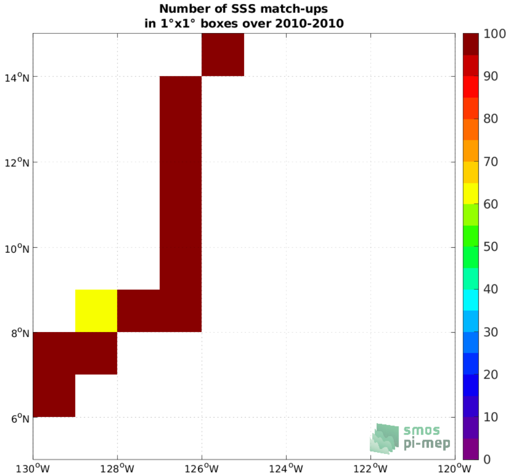
Figure 4: Number of SSS match-ups between TSG (GOSUD-Sailing-ship) SSS and the SMOS SSS L4 v1 - Weekly (CMEMS-CNR) SSS product for the SPURS 2 Pi-MEP region over 1^\circ \times 1^\circ boxes and for the full satellite product period.
