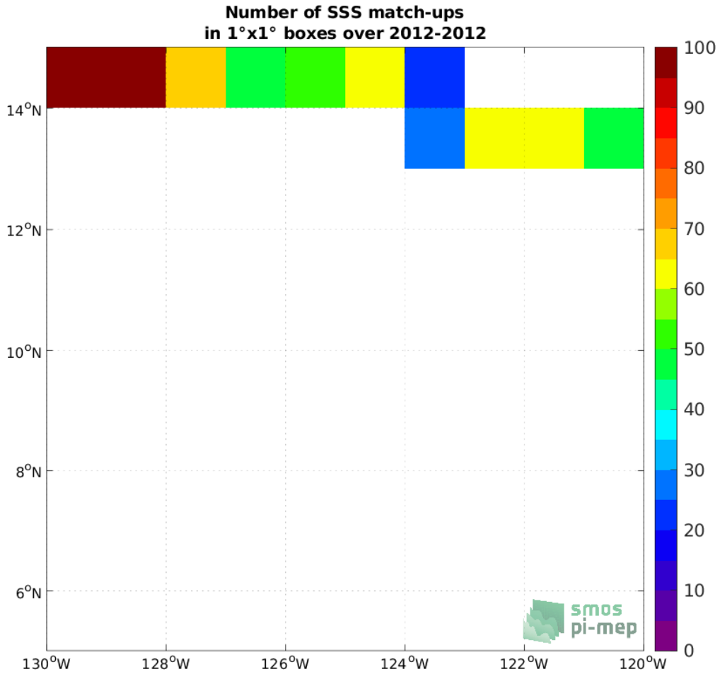
Figure 4: Number of SSS match-ups between TSG (GOSUD-Research-vessel) SSS and the SMOS SSS L4 v1 - Weekly (CMEMS-CNR) SSS product for the SPURS 2 Pi-MEP region over 1^\circ \times 1^\circ boxes and for the full satellite product period.
