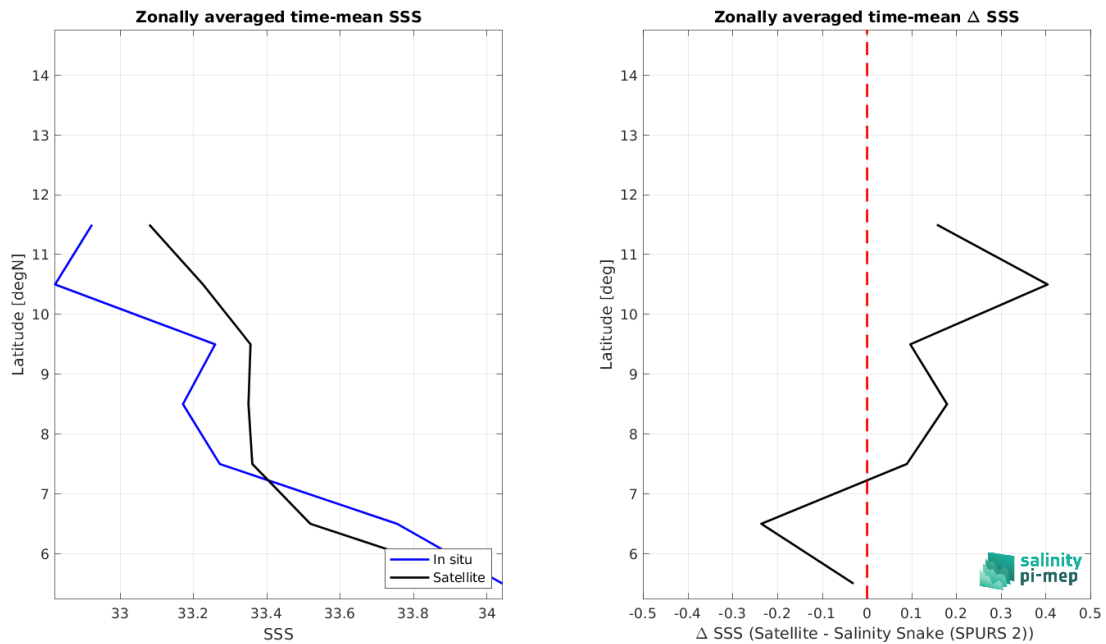
Figure 8: Left panel: Zonal mean SSS from SMOS SSS L4 v1 - Weekly (CMEMS-CNR) satellite product (black) and from Salinity Snake (SPURS 2) (blue). Right panel: Zonal mean of \Delta SSS (Satellite - Salinity Snake (SPURS 2)) for all the collected Pi-MEP match-up pairs estimated over the full satellite product period.
