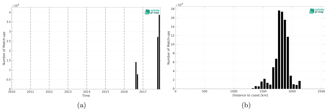
Figure 1: Number of match-ups between Salinity Snake (SPURS 2) and SMOS SSS L4 v1 - Weekly (CMEMS-CNR) SSS as a function of time (a) and as function of the distance to coast (b) over the SPURS 2 Pi-MEP region and for the full satellite product period.
