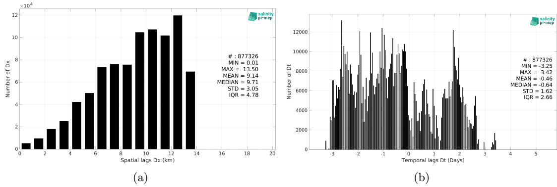
Figure 5: Histograms of the spatial (a) and temporal (b) lags between the location/time of the Salinity Snake (SPURS 2) measurement and the date of the corresponding SMOS SSS L4 v1 - Weekly (CMEMS-CNR) SSS pixel.
