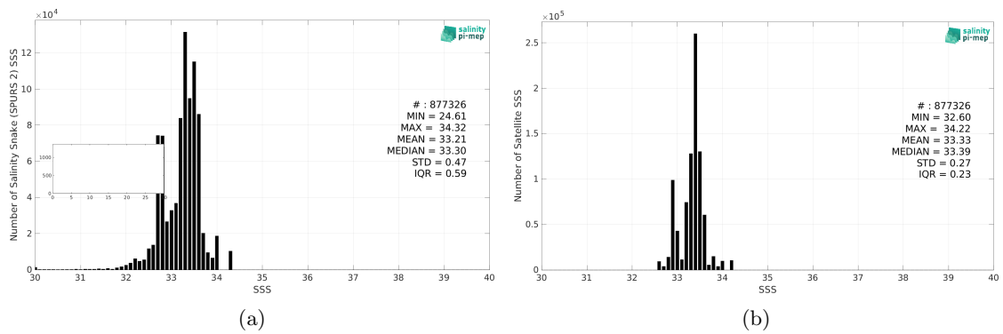
Figure 2: Histograms of SSS from Salinity Snake (SPURS 2) (a) and SMOS SSS L4 v1 - Weekly (CMEMS-CNR) (b) considering all match-up pairs per bins of 0.1 over the SPURS 2 Pi-MEP region and for the full satellite product period.
