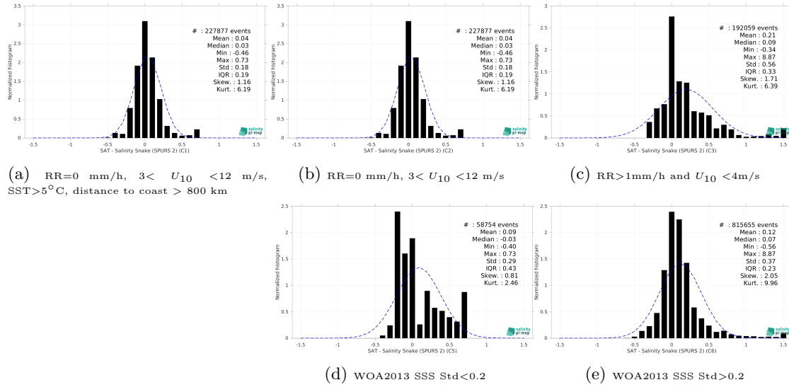
Figure 13: Normalized histogram of \Delta SSS (SMOS SSS L4 v1 - Weekly (CMEMS-CNR) - Salinity Snake (SPURS 2)) for 5 different subdatasets corresponding to: RR=0 mm/h, 3 < U_{10} < 12 m/s, SST > 5°C, distance to coast > 800 km (a), RR=0 mm/h, 3 < U_{10} < 12 m/s (b), RR > 1mm/h and U_{10} < 4 m/s (c), WOA2013 SSS Std < 0.2 (d), WOA2013 SSS Std > 0.2 (e).
