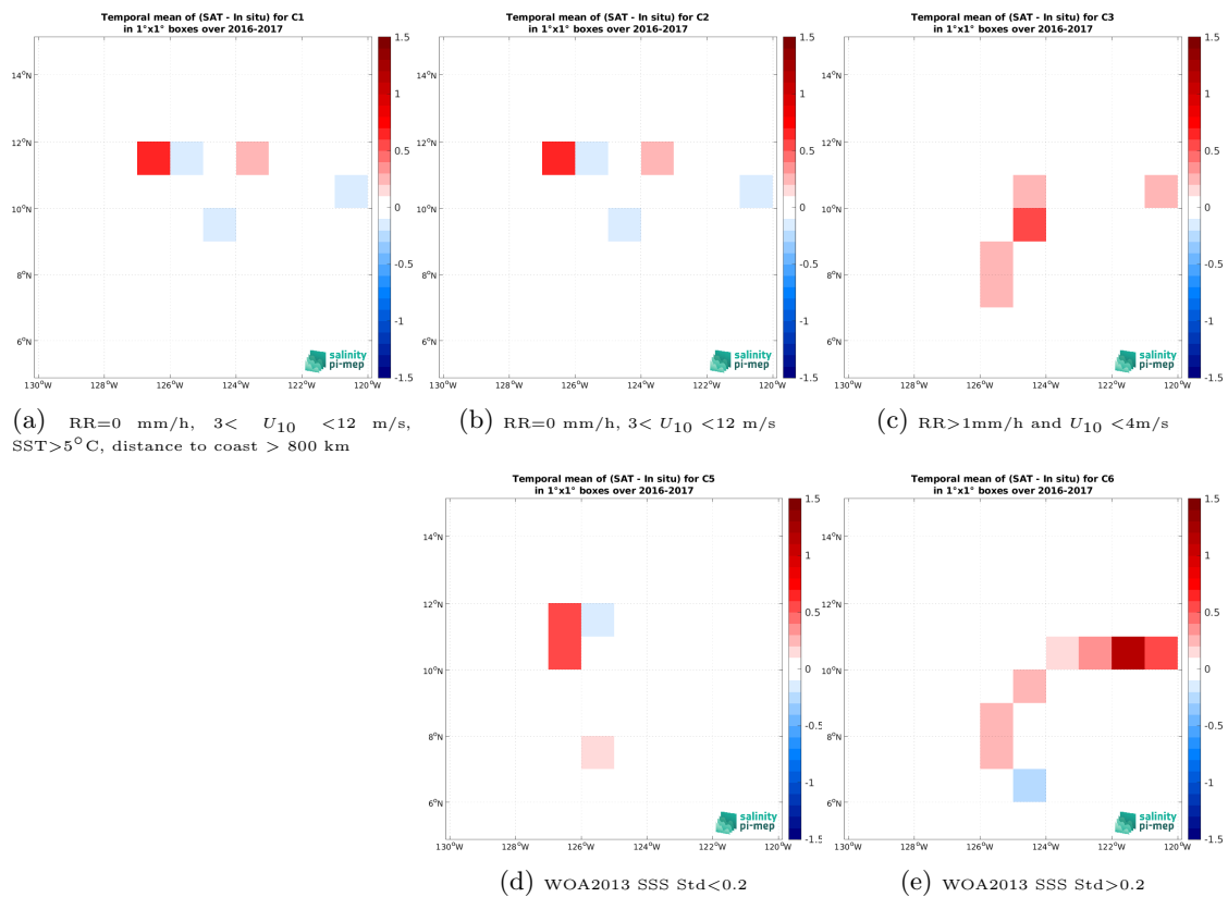
Figure 12: Temporal mean gridded over spatial boxes of size 1^\circ \times 1^\circ of \Delta SSS (SMOS SSS L4 v1 - Weekly (CMEMS-CNR) - Salinity Snake (SPURS 2)) for 5 different subdatasets corresponding to:RR=0 mm/h, 3 < U_{10} < 12 m/s, SST >5^\circ C, distance to coast > 800 km (a), RR=0 mm/h, 3 < U_{10} < 12 m/s (b), RR >1 mm/h and U_{10} < 4 m/s (c), WOA2013 SSS Std <0.2 (d), WOA2013 SSS Std >0.2 (e).
