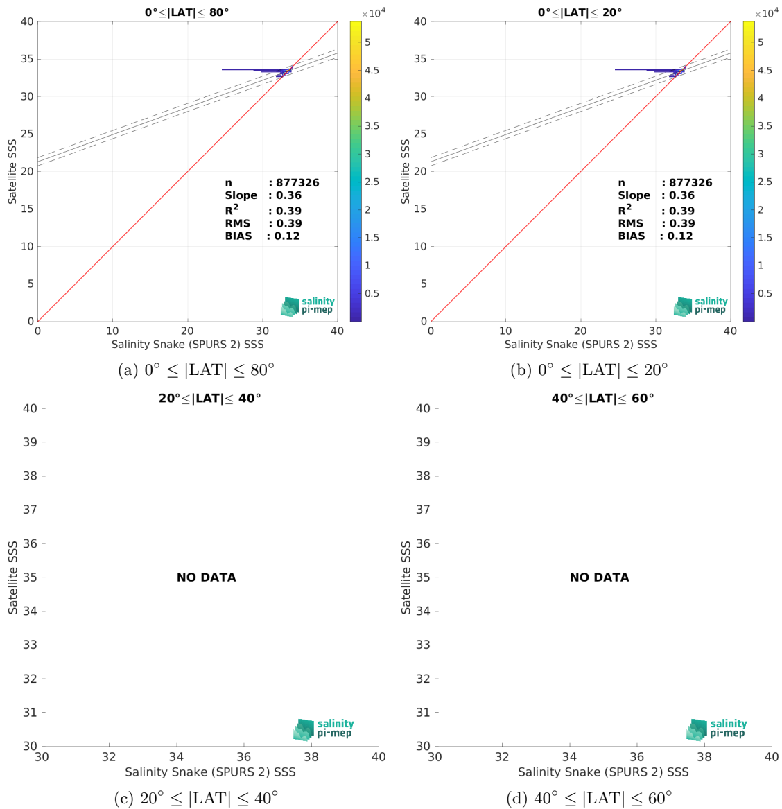
Figure 9: Contour maps of the concentration of SMOS SSS L4 v1 - Weekly (CMEMS-CNR) SSS (y-axis) versus Salinity Snake (SPURS 2) SSS (x-axis) at match-up pairs for different latitude bands. For each plot, the red line shows x=y . The black thin and dashed lines indicate a linear fit through the data cloud and the \pm 95\% confidence levels, respectively. The number match-up pairs n , the slope and R^2 coefficient of the linear fit, the root mean square (RMS) and the mean bias between satellite and in situ data are indicated for each latitude band in each plots.
