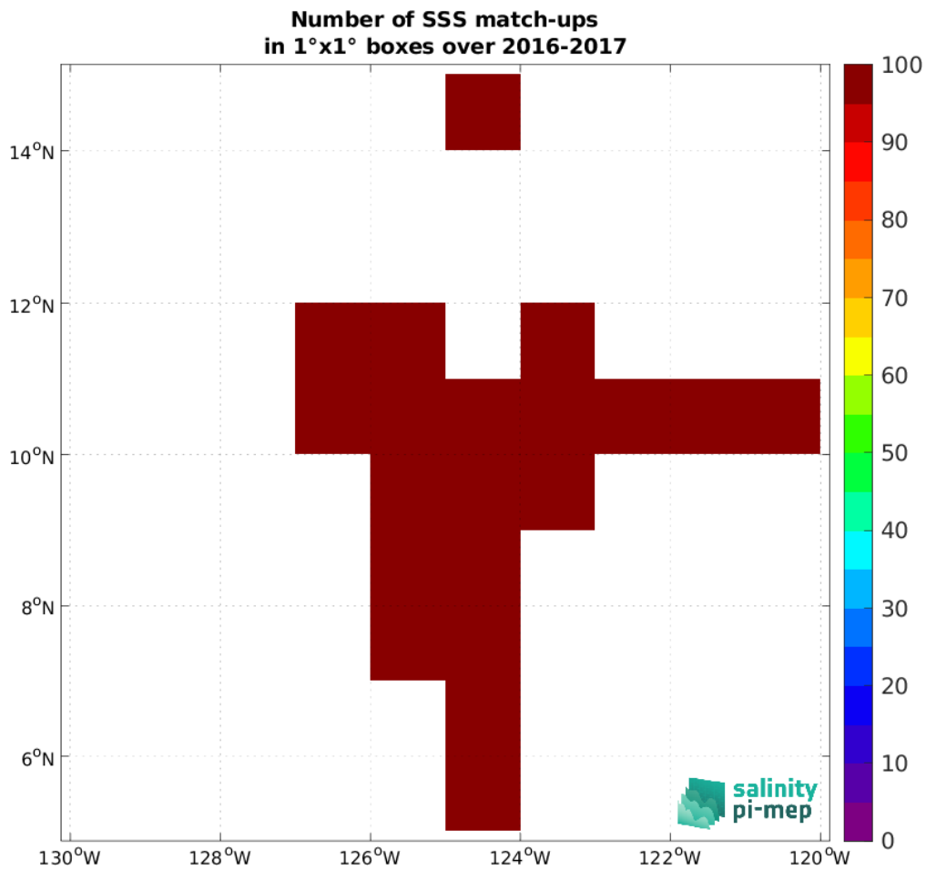
Figure 4: Number of SSS match-ups between Salinity Snake (SPURS 2) SSS and the SMOS SSS L4 v1 - Weekly (CMEMS-CNR) SSS product for the SPURS 2 Pi-MEP region over 1^\circ \times 1^\circ boxes and for the full satellite product period.
