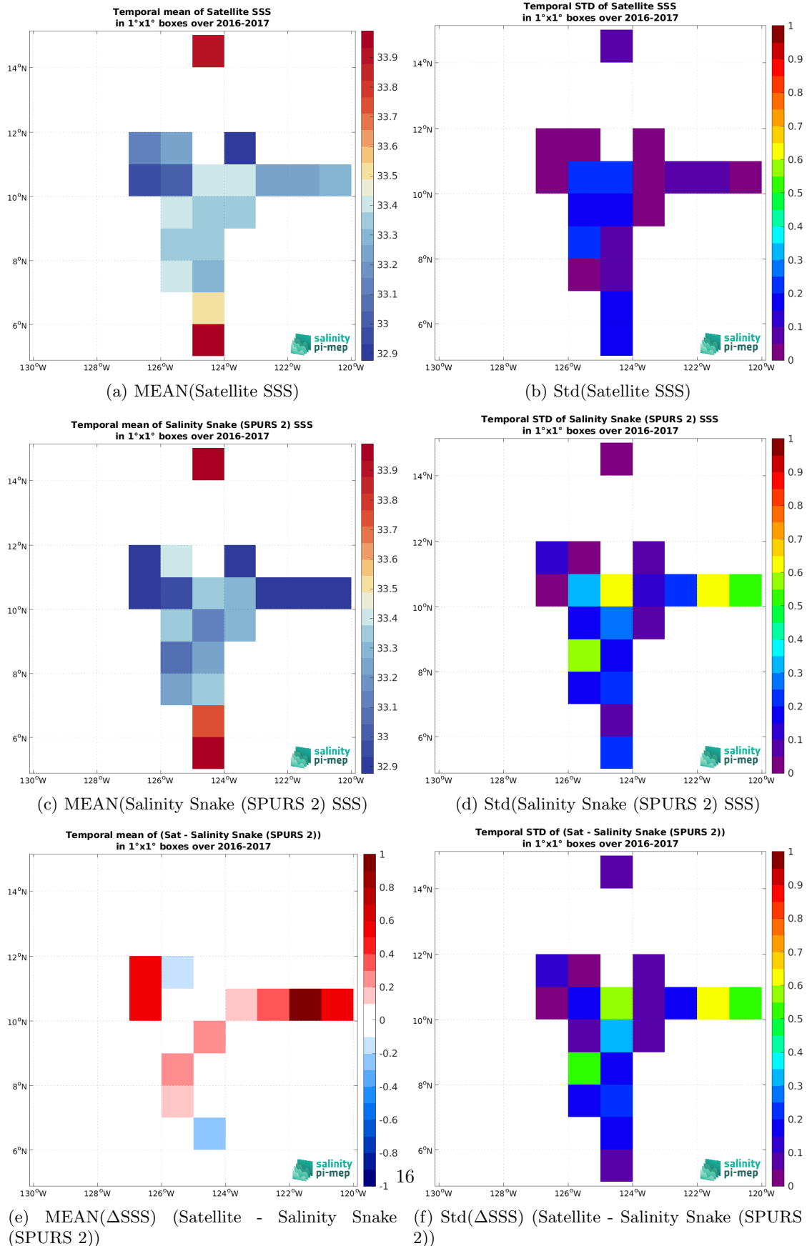
Figure 6: Temporal mean (left) and Std (right) of SSS from SMOS SSS L4 v1 - Weekly (CMEMS-CNR) (top), Salinity Snake (SPURS 2) (middle), and of \Delta SSS (Satellite - Salinity Snake (SPURS 2)). Only match-up pairs are used to generate these maps.
