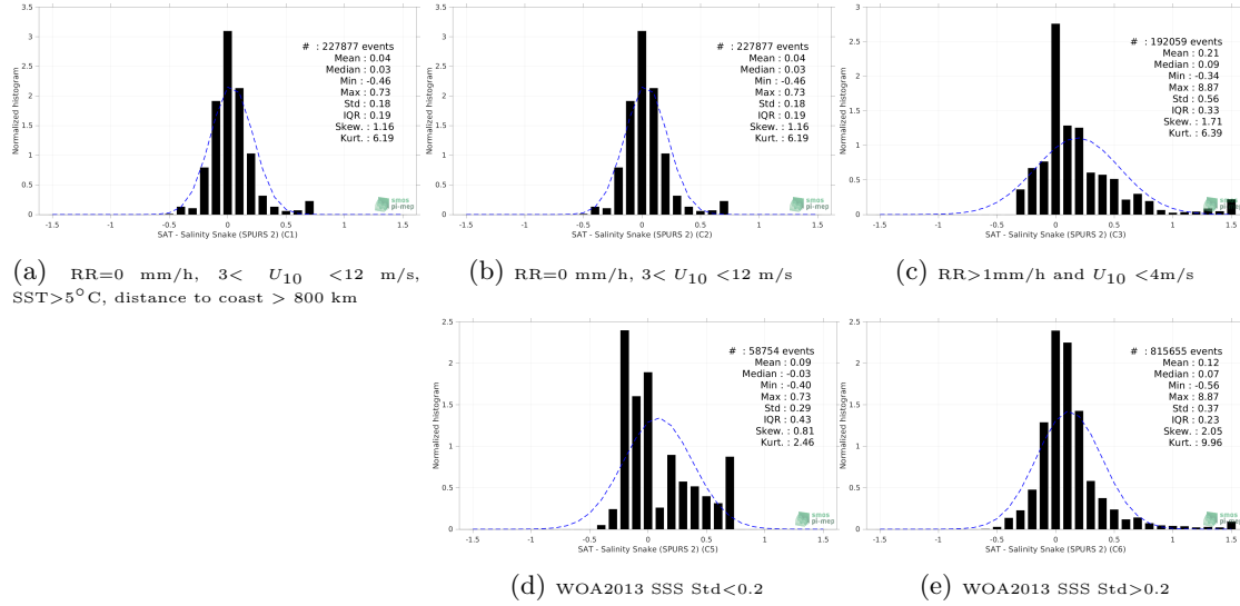
Figure 13: Normalized histogram of \Delta SSS (SMOS SSS L4 v1 - Weekly (CMEMS-CNR) - Salinity Snake (SPURS 2)) for 5 different subdatasets corresponding to: RR=0 mm/h, 3 < U_{10} < 12 m/s, SST>5°C, distance to coast > 800 km (a), RR=0 mm/h, 3 < U_{10} < 12 m/s (b), RR>1mm/h and U_{10} < 4 m/s (c), WOA2013 SSS Std<0.2 (d), WOA2013 SSS Std>0.2 (e).
