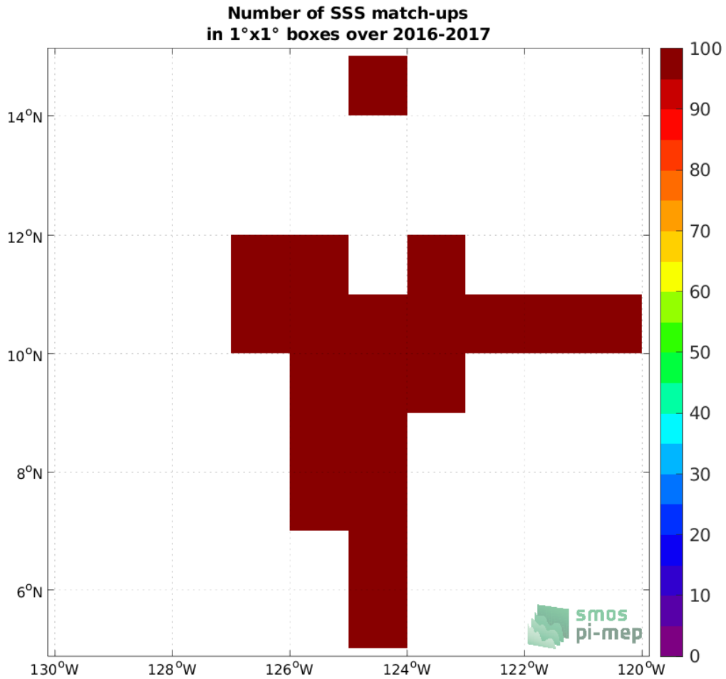
Figure 4: Number of SSS match-ups between Salinity Snake (SPURS 2) SSS and the SMOS SSS L4 v1 - Weekly (CMEMS-CNR) SSS product for the SPURS 2 Pi-MEP region over 1°x1° boxes and for the full satellite product period.
