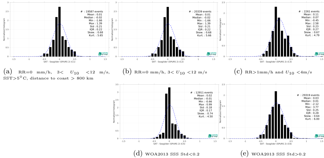
Figure 13: Normalized histogram of \Delta\text{SSS} (SMOS SSS L4 v1 - Weekly (CMEMS-CNR) - Seaglider (SPURS 2)) for 5 different subdatasets corresponding to: RR=0 mm/h, 3 < U_{10} < 12 m/s, SST >5^{\circ}\text{C} , distance to coast > 800 km (a), RR=0 mm/h, 3 < U_{10} < 12 m/s (b), RR >1 mm/h and U_{10} < 4 m/s (c), WOA2013 SSS Std <0.2 (d), WOA2013 SSS Std >0.2 (e).
