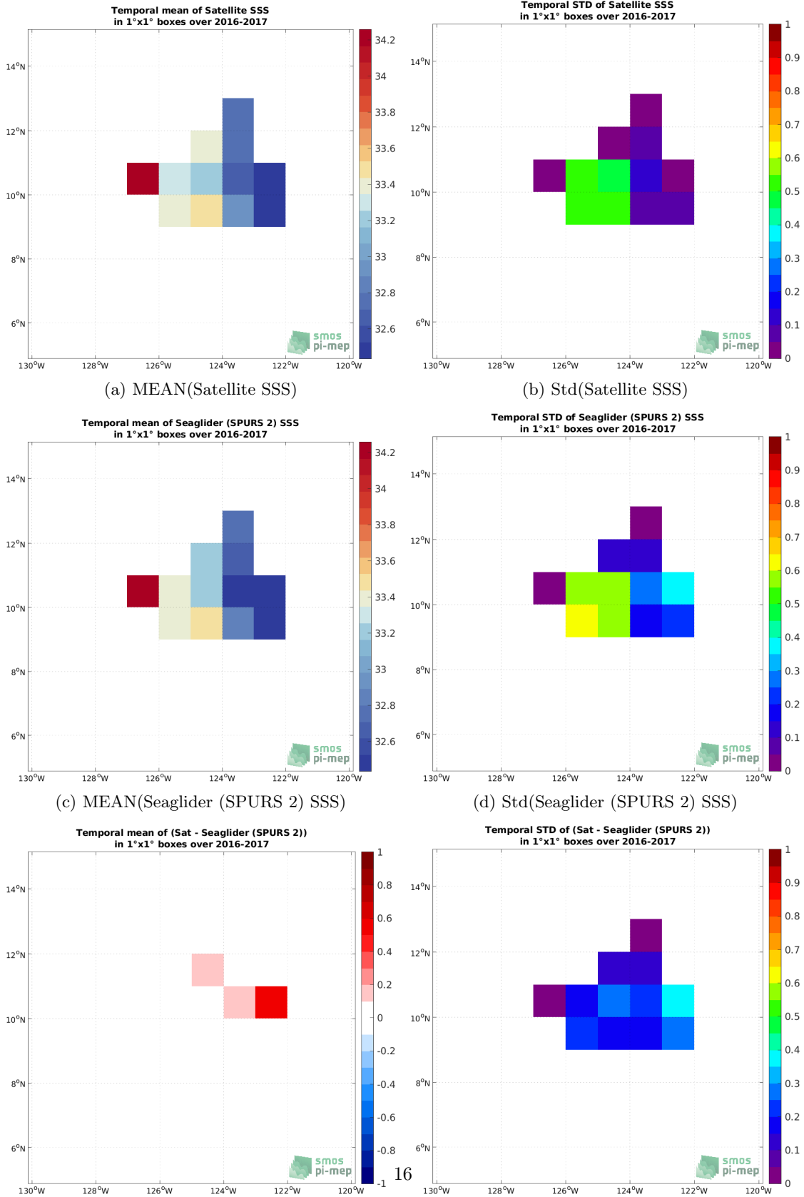
Figure 6: Temporal mean (left) and Std (right) of SSS from SMOS SSS L4 v1 - Weekly (CMEMS-CNR) (top), Seaglider (SPURS 2) (middle), and of \Delta SSS (Satellite - Seaglider (SPURS 2)). Only match-up pairs are used to generate these maps.
