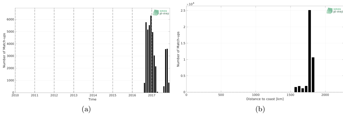
Figure 1: Number of match-ups between Seaglider (SPURS 2) and SMOS SSS L4 v1 - Weekly (CMEMS-CNR) SSS as a function of time (a) and as function of the distance to coast (b) over the SPURS 2 Pi-MEP region and for the full satellite product period.
