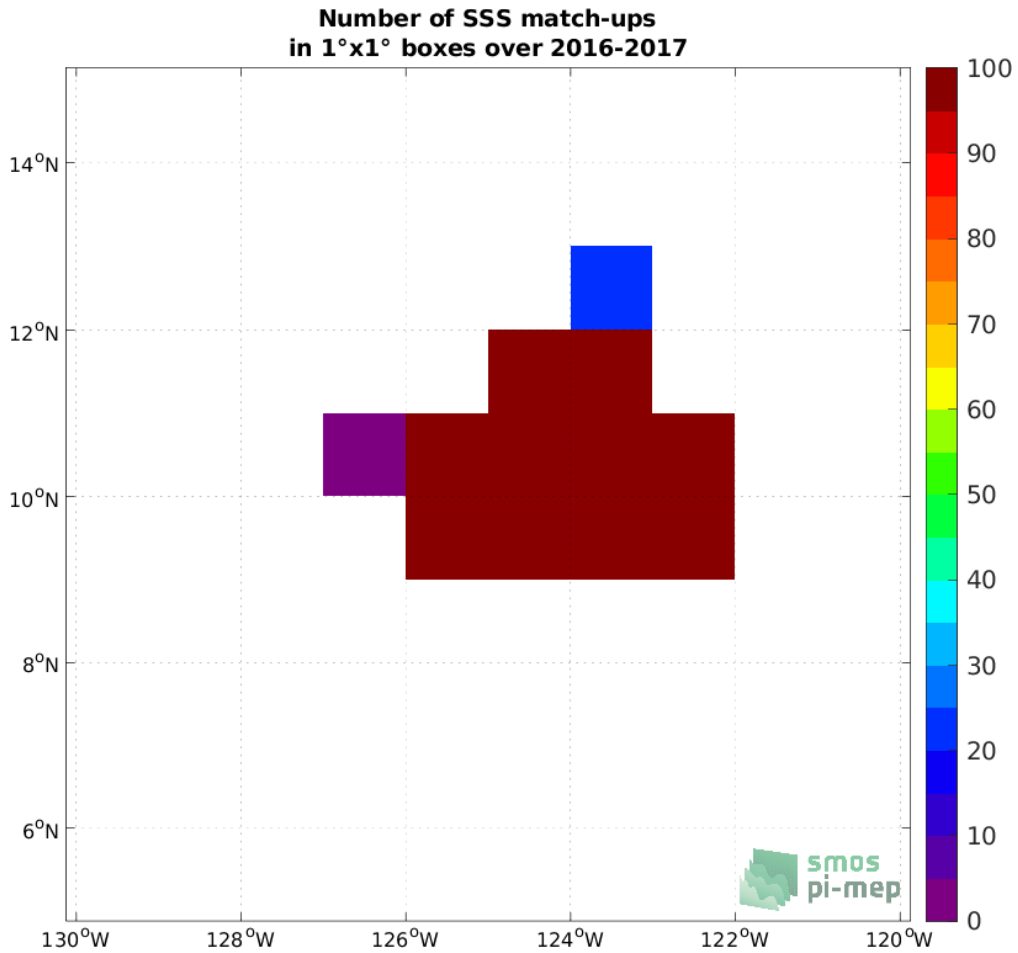
Figure 4: Number of SSS match-ups between Seaglider (SPURS 2) SSS and the SMOS SSS L4 v1 - Weekly (CMEMS-CNR) SSS product for the SPURS 2 Pi-MEP region over 1°x1° boxes and for the full satellite product period.
