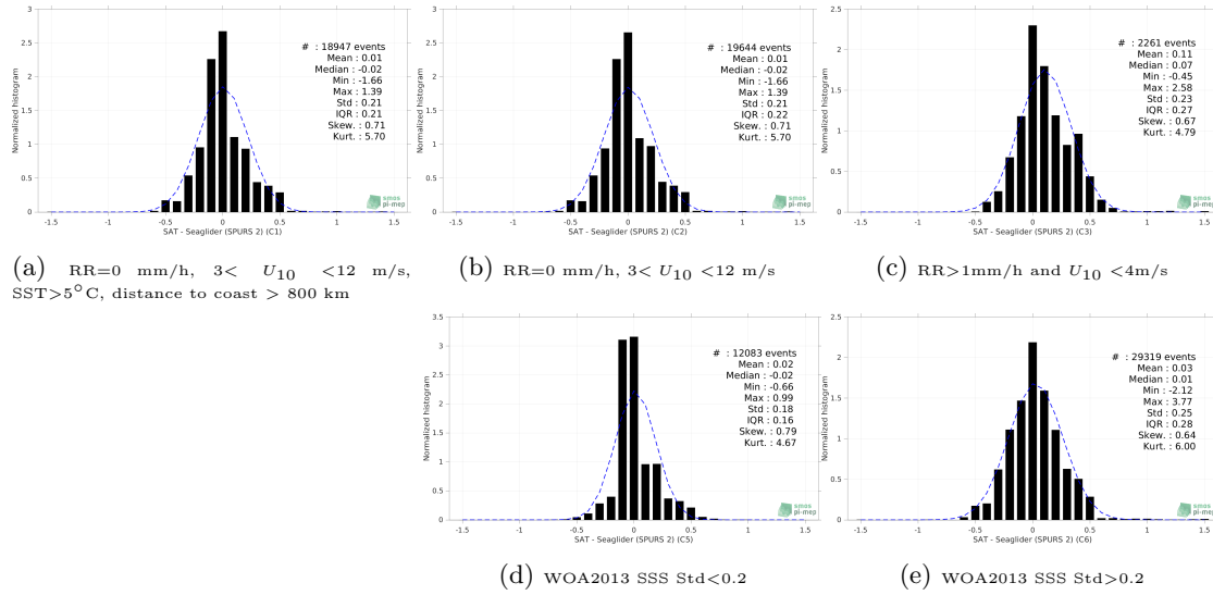
Figure 13: Normalized histogram of \Delta SSS (SMOS SSS L4 v1 - Weekly (CMEMS-CNR) - Seaglider (SPURS 2)) for 5 different subdatasets corresponding to: RR=0 mm/h, 3 < U_{10} < 12 m/s, SST > 5°C, distance to coast > 800 km (a), RR=0 mm/h, 3 < U_{10} < 12 m/s (b), RR > 1mm/h and U_{10} < 4 m/s (c), WOA2013 SSS Std < 0.2 (d), WOA2013 SSS Std > 0.2 (e).
