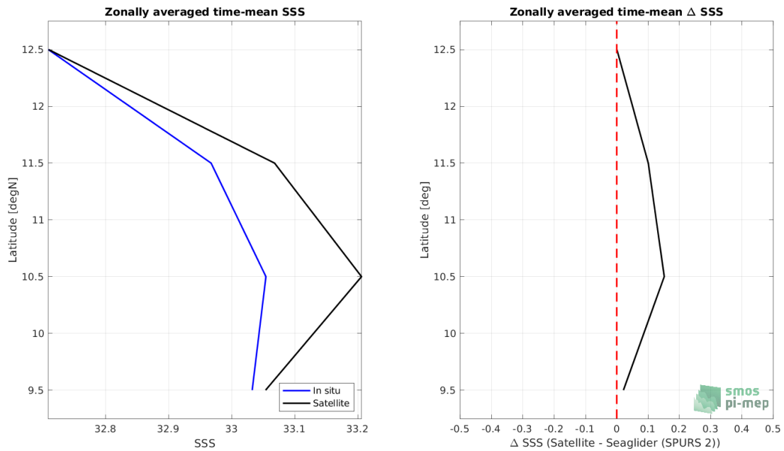
Figure 8: Left panel: Zonal mean SSS from SMOS SSS L4 v1 - Weekly (CMEMS-CNR) satellite product (black) and from Seaglider (SPURS 2) (blue). Right panel: Zonal mean of \Delta SSS (Satellite - Seaglider (SPURS 2)) for all the collected Pi-MEP match-up pairs estimated over the full satellite product period.
