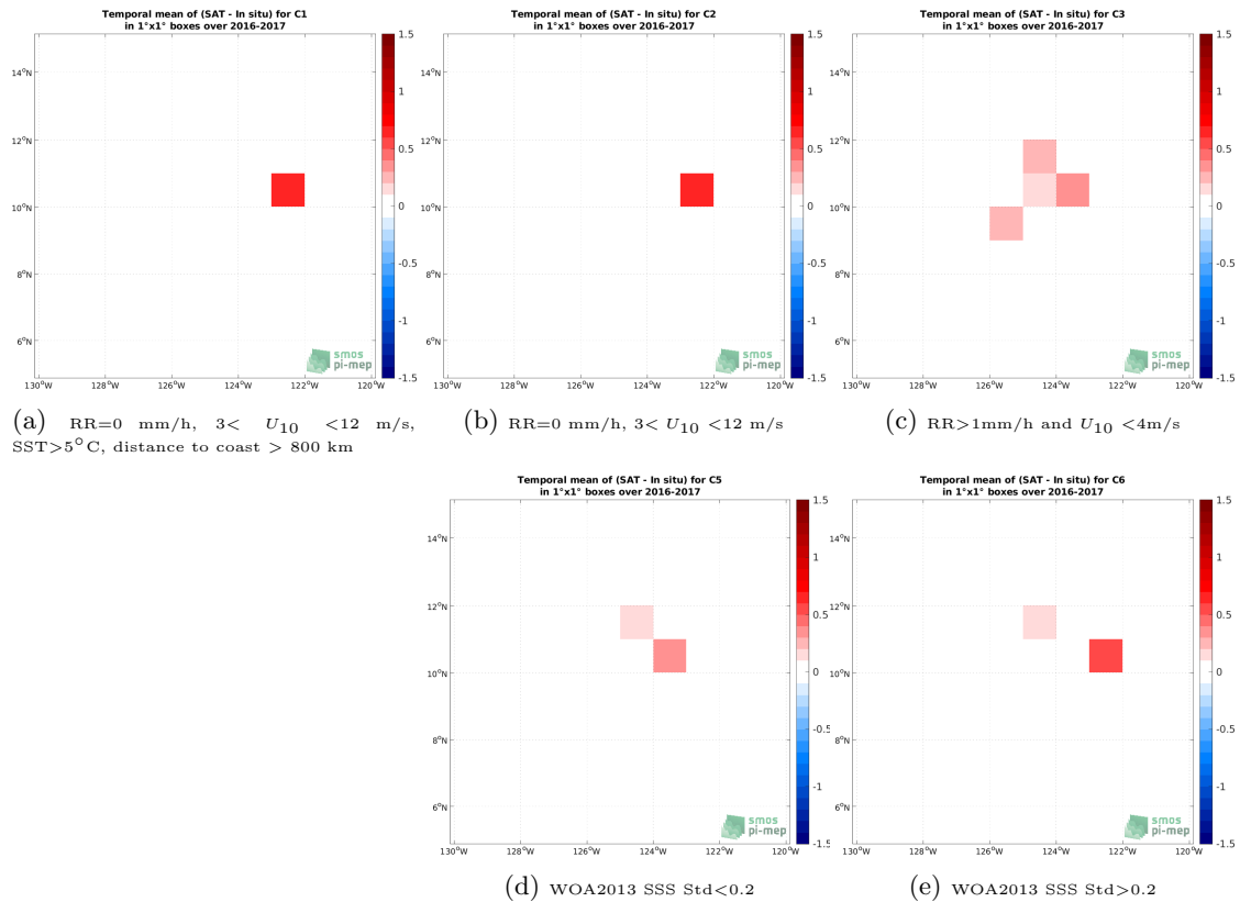
Figure 12: Temporal mean gridded over spatial boxes of size 1^\circ \times 1^\circ of \Delta SSS (SMOS SSS L4 v1 - Weekly (CMEMS-CNR) - Seaglider (SPURS 2)) for 5 different subdatasets corresponding to:RR=0 mm/h, 3 < U_{10} < 12 m/s, SST >5^\circ\text{C} , distance to coast > 800 km (a), RR=0 mm/h, 3 < U_{10} < 12 m/s (b), RR >1 mm/h and U_{10} < 4 m/s (c), WOA2013 SSS Std <0.2 (d), WOA2013 SSS Std >0.2 (e).
