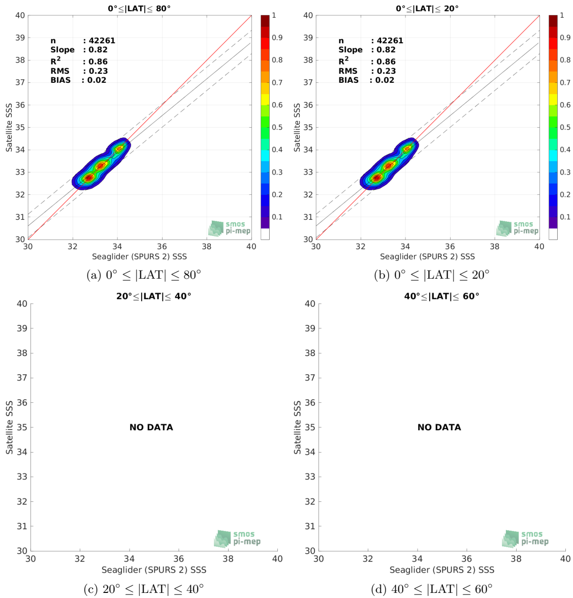
Figure 9: Contour maps of the concentration of SMOS SSS L4 v1 - Weekly (CMEMS-CNR) SSS (y-axis) versus Seaglider (SPURS 2) SSS (x-axis) at match-up pairs for different latitude bands. For each plot, the red line shows x=y . The black thin and dashed lines indicate a linear fit through the data cloud and the \pm 95\% confidence levels, respectively. The number match-up pairs n , the slope and R^2 coefficient of the linear fit, the root mean square (RMS) and the mean bias between satellite and in situ data are indicated for each latitude band in each plots.
