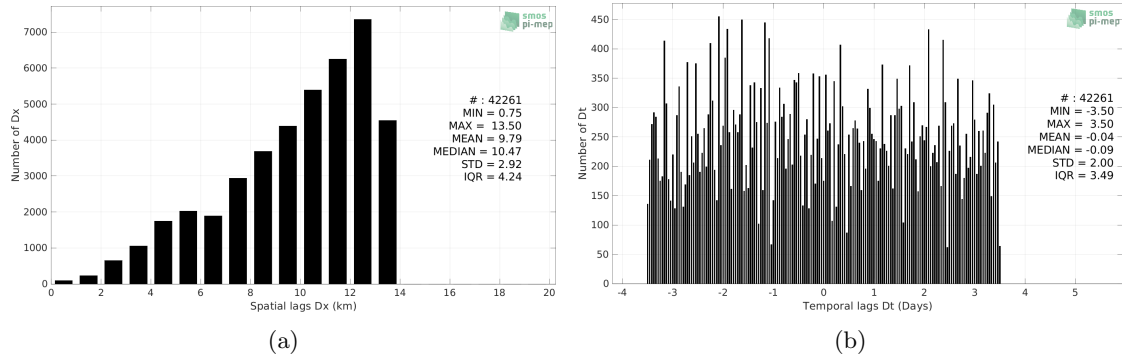
Figure 5: Histograms of the spatial (a) and temporal (b) lags between the location/time of the Seaglider (SPURS 2) measurement and the date of the corresponding SMOS SSS L4 v1 - Weekly (CMEMS-CNR) SSS pixel.
