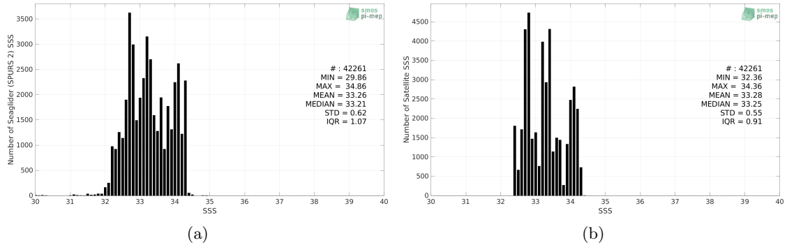
Figure 2: Histograms of SSS from Seaglider (SPURS 2) (a) and SMOS SSS L4 v1 - Weekly (CMEMS-CNR) (b) considering all match-up pairs per bins of 0.1 over the SPURS 2 Pi-MEP region and for the full satellite product period.
