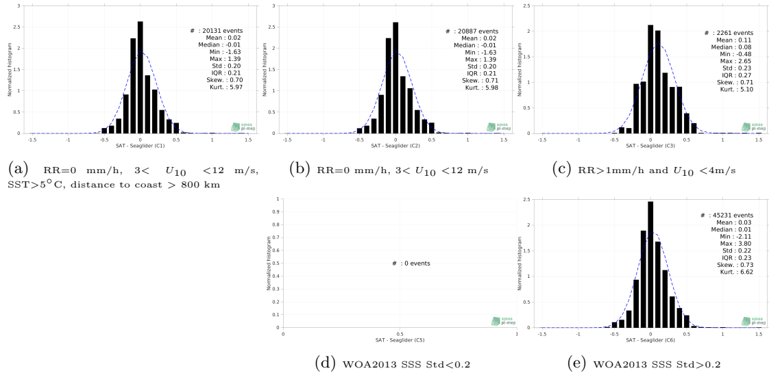
Figure 12: Normalized histogram of \Delta SSS (SMOS SSS L4 v1 - Weekly (CMEMS-CNR) - Seaglider) for 5 different subdatasets corresponding to: RR=0 mm/h, 3 < U_{10} < 12 m/s, SST>5°C, distance to coast > 800 km (a), RR=0 mm/h, 3 < U_{10} < 12 m/s (b), RR>1mm/h and U_{10} < 4 m/s (c), WOA2013 SSS Std<0.2 (d), WOA2013 SSS Std>0.2 (e).
