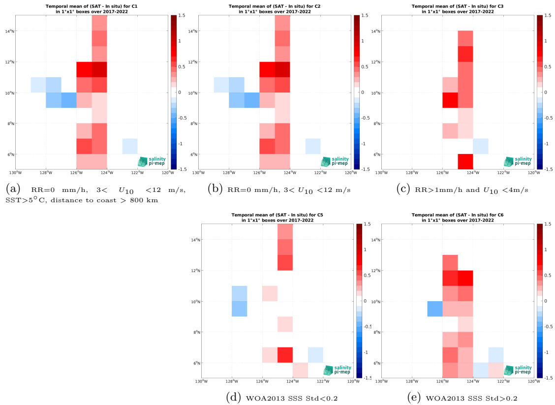
Figure 12: Temporal mean gridded over spatial boxes of size 1^\circ \times 1^\circ of \Delta SSS (SMOS SSS L4 v1 - Weekly (CMEMS-CNR) - Saildrone) for 5 different subdatasets corresponding to:RR=0 mm/h, 3 < U_{10} < 12 m/s, SST >5^\circ\text{C} , distance to coast > 800 km (a), RR=0 mm/h, 3 < U_{10} < 12 m/s (b), RR >1 mm/h and U_{10} < 4 m/s (c), WOA2013 SSS Std <0.2 (d), WOA2013 SSS Std >0.2 (e).
