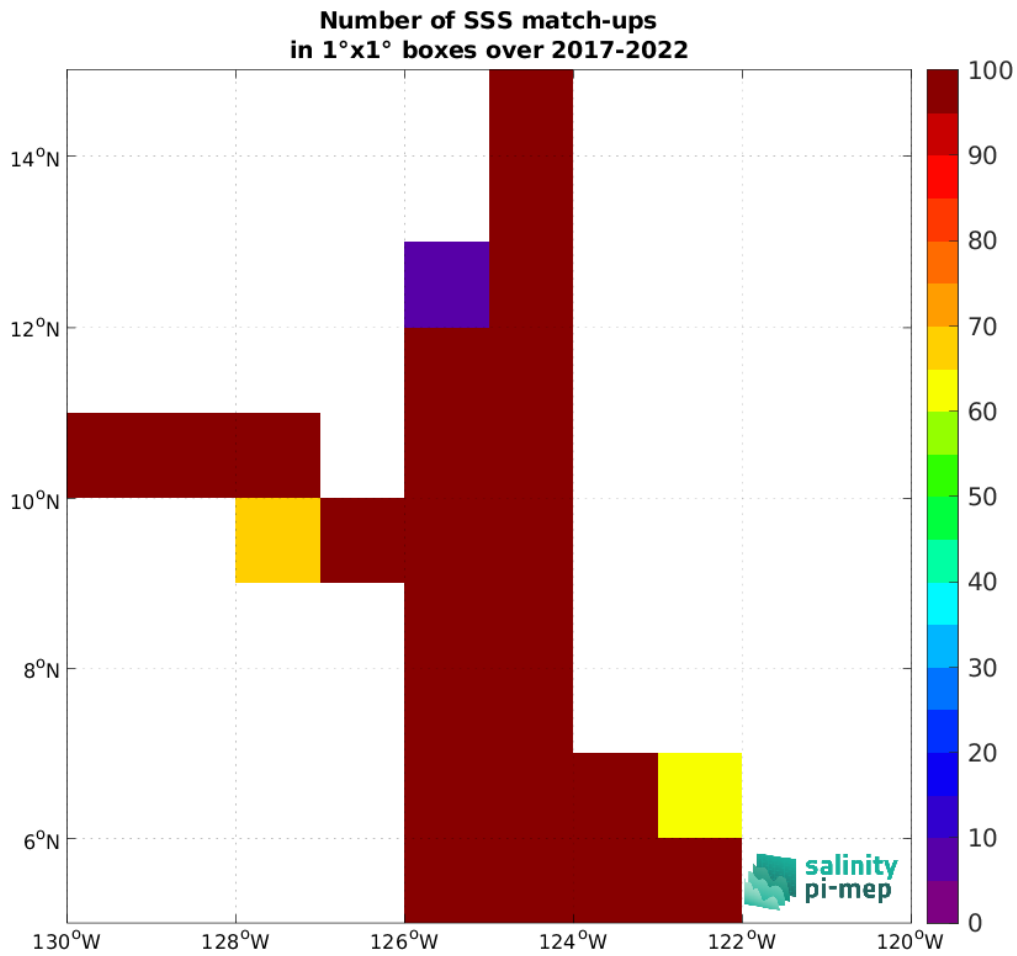
Figure 4: Number of SSS match-ups between Saildrone SSS and the SMOS SSS L4 v1 - Weekly (CMEMS-CNR) SSS product for the SPURS 2 Pi-MEP region over 1°x1° boxes and for the full satellite product period.
