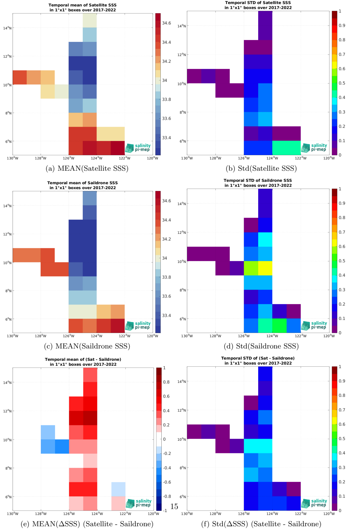
Figure 6: Temporal mean (left) and Std (right) of SSS from SMOS SSS L4 v1 - Weekly (CMEMS-CNR) (top), Saildrone (middle), and of \Delta SSS (Satellite - Saildrone). Only match-up pairs are used to generate these maps.
