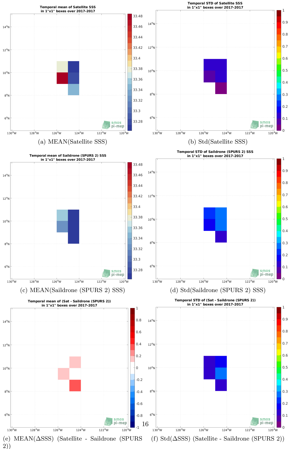
Figure 6: Temporal mean (left) and Std (right) of SSS from SMOS SSS L4 v1 - Weekly (CMEMS-CNR) (top), Saildrone (SPURS 2) (middle), and of \Delta SSS (Satellite - Saildrone (SPURS 2)). Only match-up pairs are used to generate these maps.
