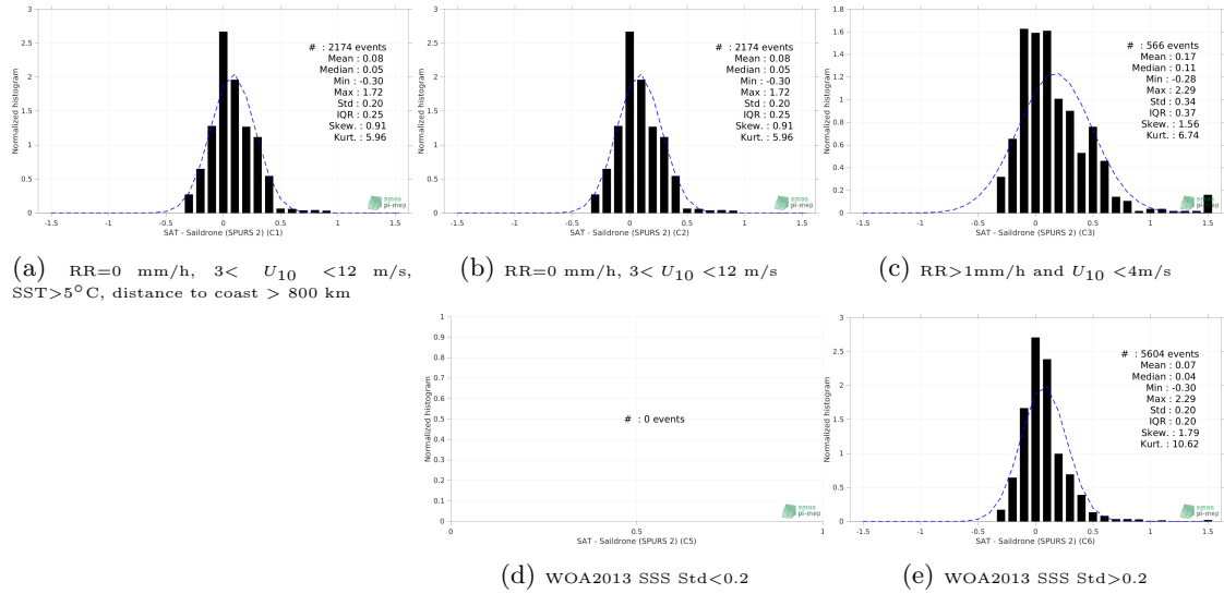
Figure 13: Normalized histogram of \Delta SSS (SMOS SSS L4 v1 - Weekly (CMEMS-CNR) - Saildrone (SPURS 2)) for 5 different subdatasets corresponding to: RR=0 mm/h, 3 < U_{10} < 12 m/s, SST > 5°C, distance to coast > 800 km (a), RR=0 mm/h, 3 < U_{10} < 12 m/s (b), RR > 1mm/h and U_{10} < 4 m/s (c), WOA2013 SSS Std < 0.2 (d), WOA2013 SSS Std > 0.2 (e).
