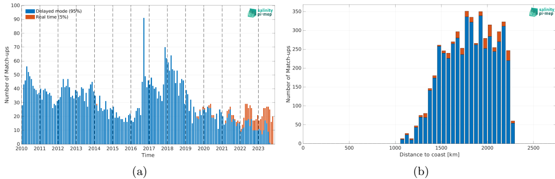
Figure 1: Number of match-ups between Argo and SMOS SSS L4 v1 - Weekly (CMEMS-CNR) SSS as a function of time (a) and as function of the distance to coast (b) over the SPURS 2 Pi-MEP region and for the full satellite product period.
