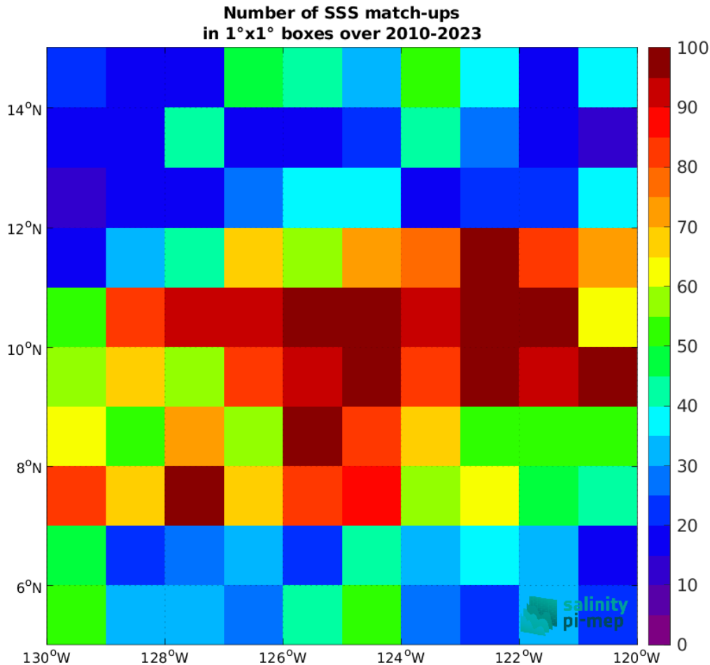
Figure 4: Number of SSS match-ups between Argo SSS and the SMOS SSS L4 v1 - Weekly (CMEMS-CNR) SSS product for the SPURS 2 Pi-MEP region over 1^\circ \times 1^\circ boxes and for the full satellite product period.
