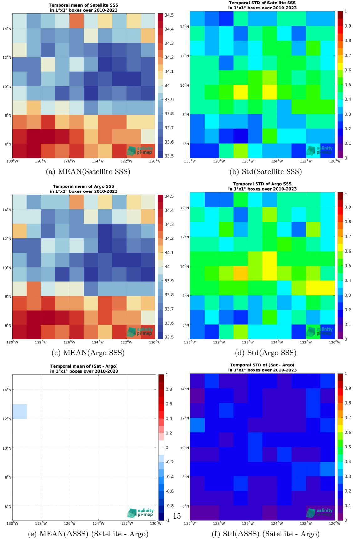
Figure 6: Temporal mean (left) and Std (right) of SSS from SMOS SSS L4 v1 - Weekly (CMEMS-CNR) (top), Argo (middle), and of \Delta SSS (Satellite - Argo). Only match-up pairs are used to generate these maps.
