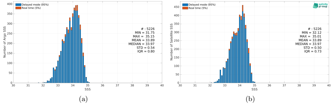
Figure 2: Histograms of SSS from Argo (a) and SMOS SSS L4 v1 - Weekly (CMEMS-CNR) (b) considering all match-up pairs per bins of 0.1 over the SPURS 2 Pi-MEP region and for the full satellite product period.
