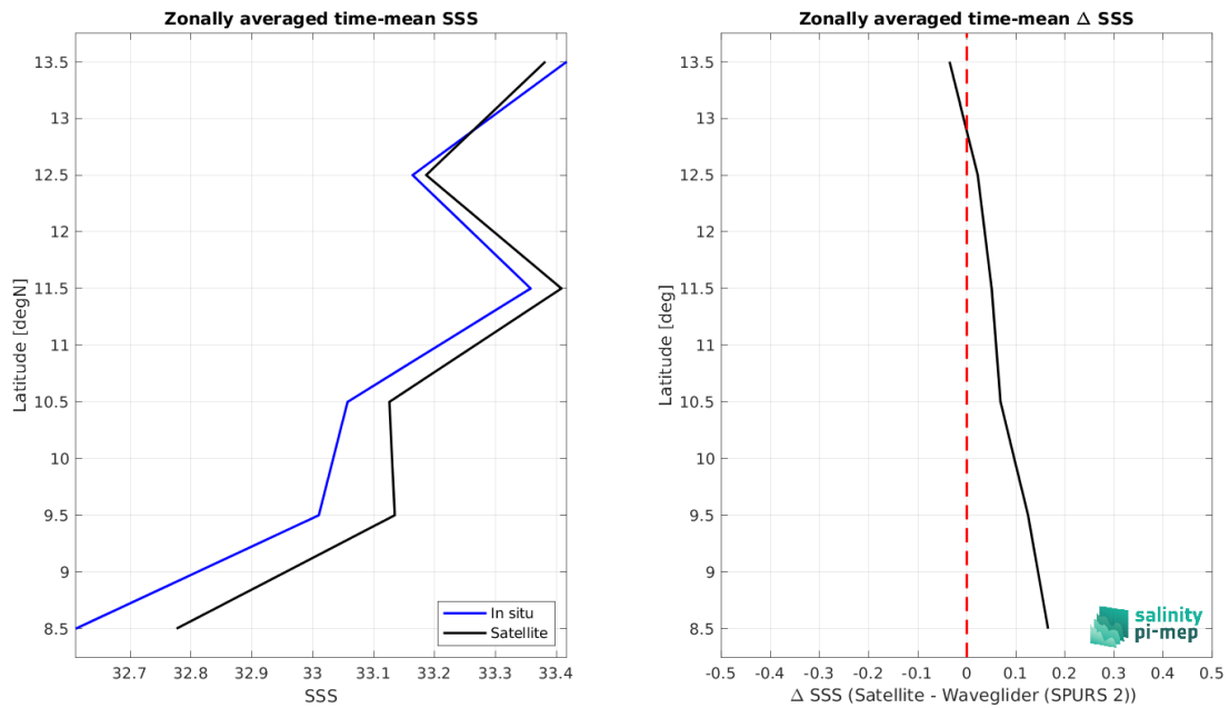
Figure 8: Left panel: Zonal mean SSS from SMOS SSS L4 v1 - Monthly (CMEMS-CNR) satellite product (black) and from Waveglider (SPURS 2) (blue). Right panel: Zonal mean of \Delta SSS (Satellite - Waveglider (SPURS 2)) for all the collected Pi-MEP match-up pairs estimated over the full satellite product period.
