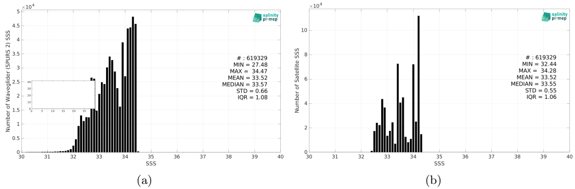
Figure 2: Histograms of SSS from Waveglider (SPURS 2) (a) and SMOS SSS L4 v1 - Monthly (CMEMS-CNR) (b) considering all match-up pairs per bins of 0.1 over the SPURS 2 Pi-MEP region and for the full satellite product period.
