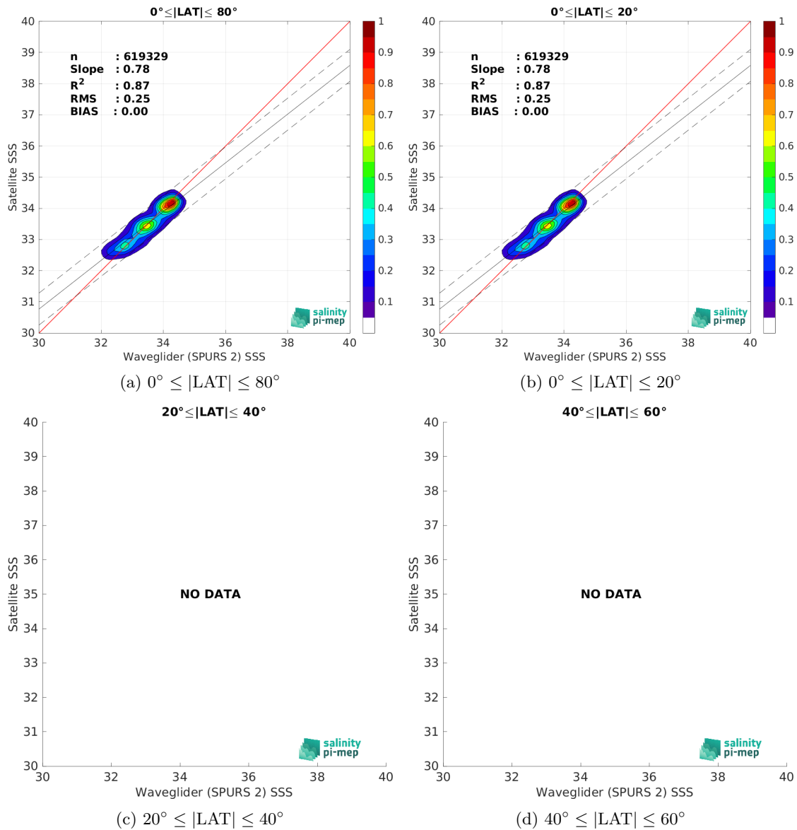
Figure 9: Contour maps of the concentration of SMOS SSS L4 v1 - Monthly (CMEMS-CNR) SSS (y-axis) versus Waveglider (SPURS 2) SSS (x-axis) at match-up pairs for different latitude bands. For each plot, the red line shows x=y . The black thin and dashed lines indicate a linear fit through the data cloud and the \pm 95\% confidence levels, respectively. The number match-up pairs n , the slope and R^2 coefficient of the linear fit, the root mean square (RMS) and the mean bias between satellite and in situ data are indicated for each latitude band in each plots.
