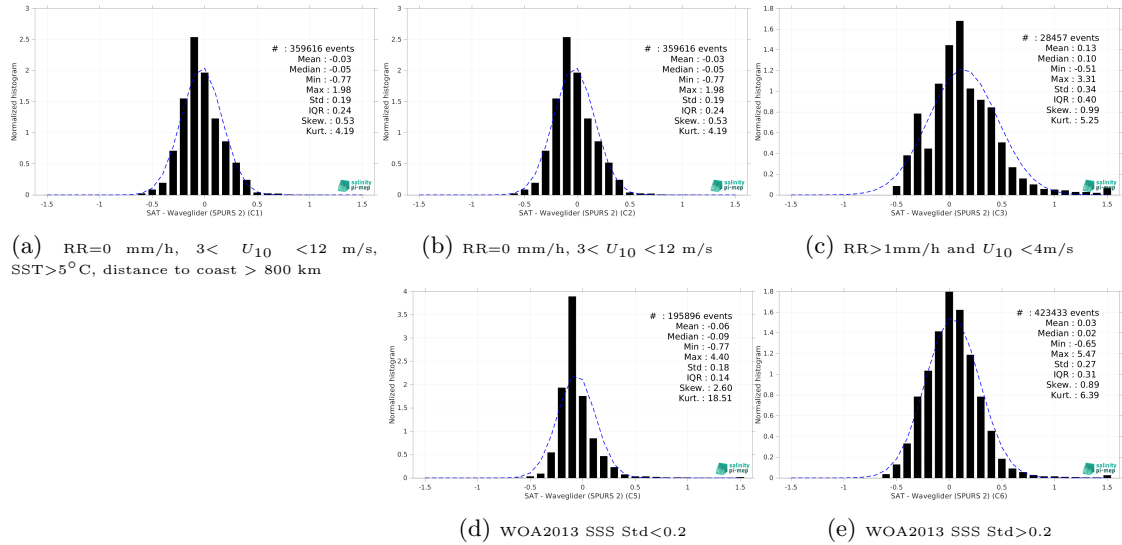
Figure 13: Normalized histogram of \Delta SSS (SMOS SSS L4 v1 - Monthly (CMEMS-CNR) - Waveglider (SPURS 2)) for 5 different subdatasets corresponding to: RR=0 mm/h, 3 < U_{10} < 12 m/s, SST > 5°C, distance to coast > 800 km (a), RR=0 mm/h, 3 < U_{10} < 12 m/s (b), RR > 1mm/h and U_{10} < 4 m/s (c), WOA2013 SSS Std < 0.2 (d), WOA2013 SSS Std > 0.2 (e).
