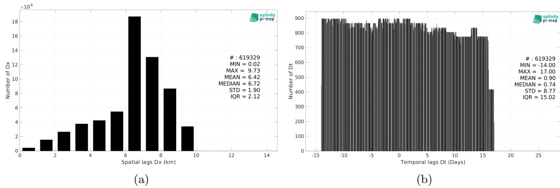
Figure 5: Histograms of the spatial (a) and temporal (b) lags between the location/time of the Waveglider (SPURS 2) measurement and the date of the corresponding SMOS SSS L4 v1 - Monthly (CMEMS-CNR) SSS pixel.
