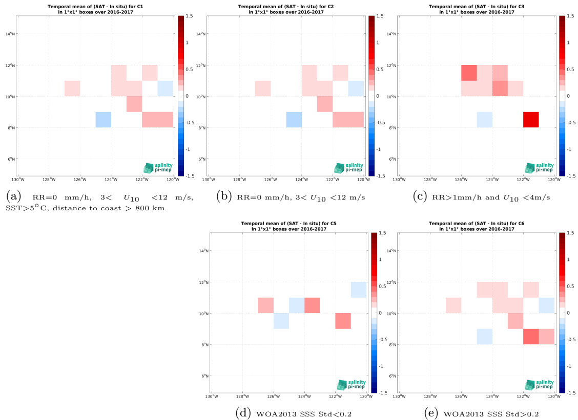
Figure 12: Temporal mean gridded over spatial boxes of size 1^\circ \times 1^\circ of \Delta SSS (SMOS SSS L4 v1 - Monthly (CMEMS-CNR) - Waveglider (SPURS 2)) for 5 different subdatasets corresponding to:RR=0 mm/h, 3 < U_{10} < 12 m/s, SST >5^\circ\text{C} , distance to coast > 800 km (a), RR=0 mm/h, 3 < U_{10} < 12 m/s (b), RR >1 mm/h and U_{10} < 4 m/s (c), WOA2013 SSS Std <0.2 (d), WOA2013 SSS Std >0.2 (e).
