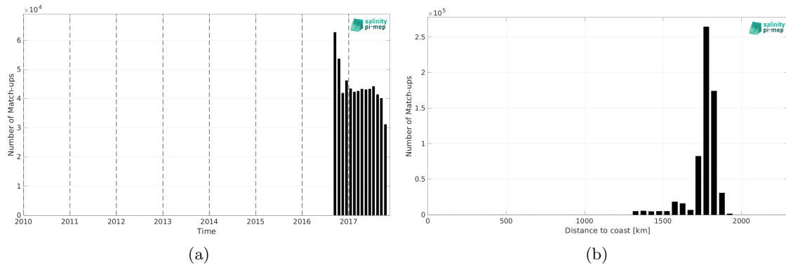
Figure 1: Number of match-ups between Waveglider (SPURS 2) and SMOS SSS L4 v1 - Monthly (CMEMS-CNR) SSS as a function of time (a) and as function of the distance to coast (b) over the SPURS 2 Pi-MEP region and for the full satellite product period.
