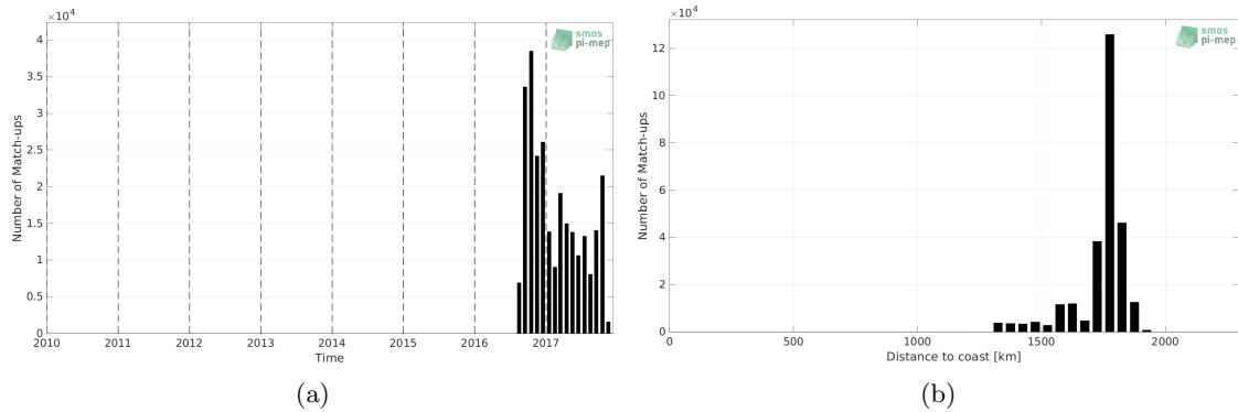
Figure 1: Number of match-ups between Waveglider and SMOS SSS L4 v1 - Monthly (CMEMS-CNR) SSS as a function of time (a) and as function of the distance to coast (b) over the SPURS 2 Pi-MEP region and for the full satellite product period.
