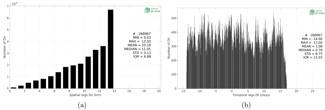
Figure 4: Histograms of the spatial (a) and temporal (b) lags between the location/time of the Waveglider measurement and the date of the corresponding SMOS SSS L4 v1 - Monthly (CMEMS-CNR) SSS pixel.
