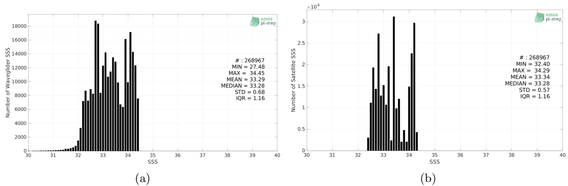
Figure 2: Histograms of SSS from Waveglider (a) and SMOS SSS L4 v1 - Monthly (CMEMS-CNR) (b) considering all match-up pairs per bins of 0.1 over the SPURS 2 Pi-MEP region and for the full satellite product period.
