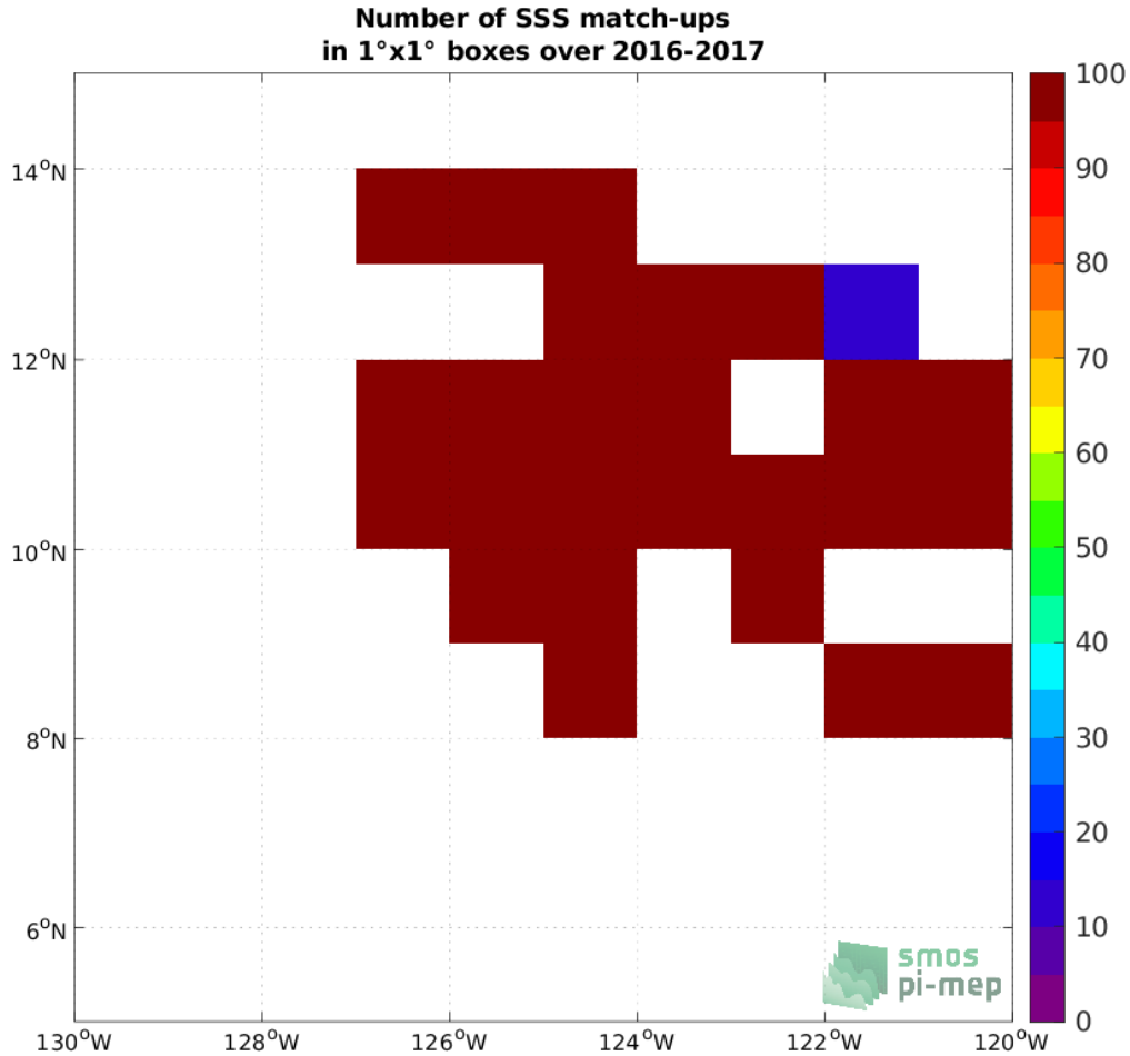
Figure 3: Number of SSS match-ups between Waveglider SSS and the SMOS SSS L4 v1 - Monthly (CMEMS-CNR) SSS product for the SPURS 2 Pi-MEP region over 1^\circ \times 1^\circ boxes and for the full satellite product period.
