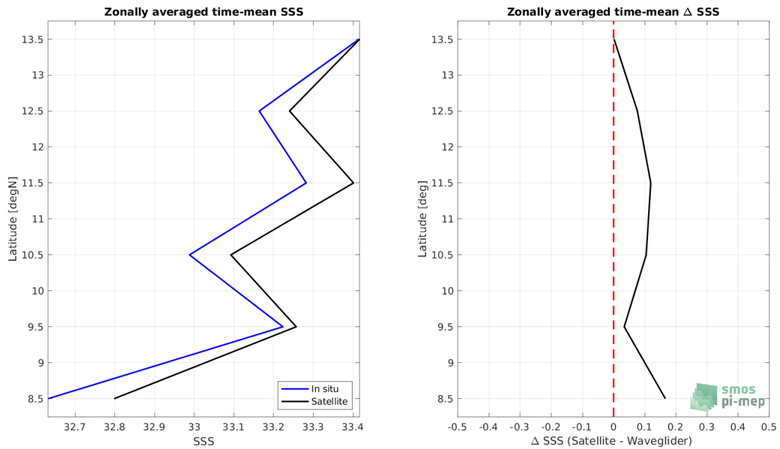
Figure 7: Left panel: Zonal mean SSS from SMOS SSS L4 v1 - Monthly (CMEMS-CNR) satellite product (black) and from Waveglider (blue). Right panel: Zonal mean of \Delta SSS (Satellite - Waveglider) for all the collected Pi-MEP match-up pairs estimated over the full satellite product period.
