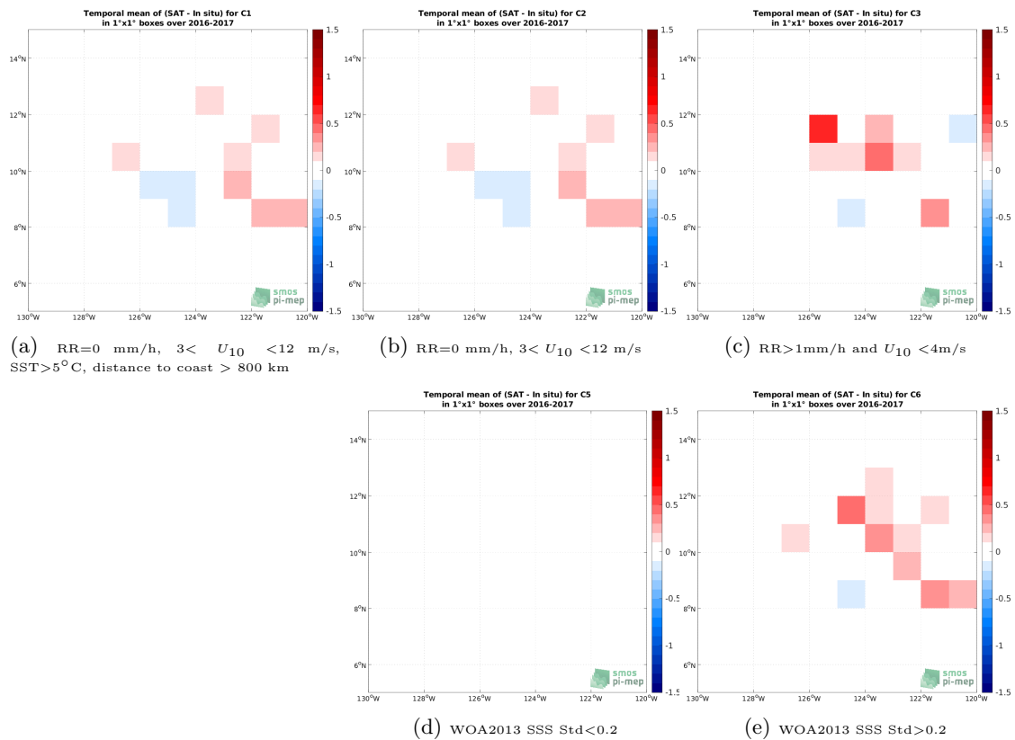
Figure 11: Temporal mean gridded over spatial boxes of size 1^\circ \times 1^\circ of \Delta SSS (SMOS SSS L4 v1 - Monthly (CMEMS-CNR) - Waveglider) for 5 different subdatasets corresponding to:RR=0 mm/h, 3 < U_{10} < 12 m/s, SST >5^\circ\text{C} , distance to coast > 800 km (a), RR=0 mm/h, 3 < U_{10} < 12 m/s (b), RR >1 mm/h and U_{10} < 4 m/s (c), WOA2013 SSS Std <0.2 (d), WOA2013 SSS Std >0.2 (e).
