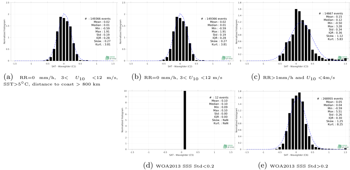
Figure 12: Normalized histogram of \Delta SSS (SMOS SSS L4 v1 - Monthly (CMEMS-CNR) - Waveglider) for 5 different subdatasets corresponding to: RR=0 mm/h, 3 < U_{10} < 12 m/s, SST > 5°C, distance to coast > 800 km (a), RR=0 mm/h, 3 < U_{10} < 12 m/s (b), RR > 1mm/h and U_{10} < 4 m/s (c), WOA2013 SSS Std < 0.2 (d), WOA2013 SSS Std > 0.2 (e).
