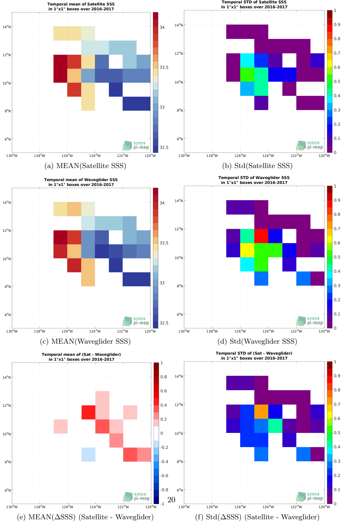
Figure 5: Temporal mean (left) and Std (right) of SSS from SMOS SSS L4 v1 - Monthly (CMEMS-CNR) (top), Waveglider (middle), and of \Delta SSS (Satellite - Waveglider). Only match-pairs are used to generate these maps.
