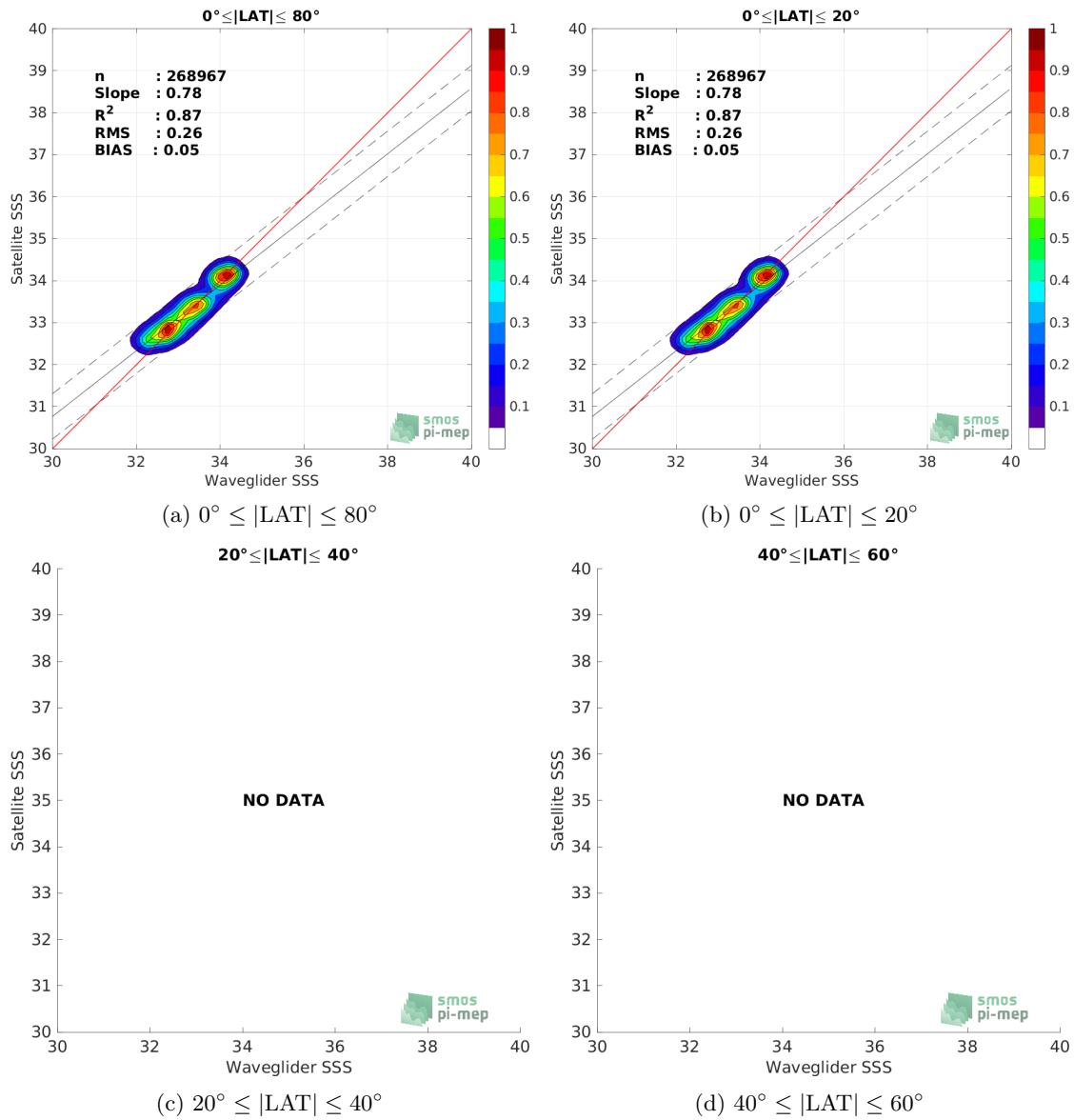
Figure 8: Contour maps of the concentration of SMOS SSS L4 v1 - Monthly (CMEMS-CNR) SSS (y-axis) versus Waveglider SSS (x-axis) at match-up pairs for different latitude bands. For each plot, the red line shows x=y . The black thin and dashed lines indicate a linear fit through the data cloud and the \pm 95\% confidence levels, respectively. The number match-up pairs n , the slope and R^2 coefficient of the linear fit, the root mean square (RMS) and the mean bias between satellite and in situ data are indicated for each latitude band in each plots.
