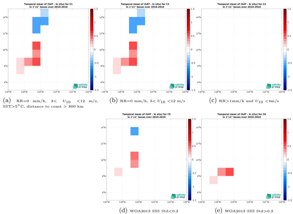
Figure 12: Temporal mean gridded over spatial boxes of size 1^\circ \times 1^\circ of \Delta\text{SSS} (SMOS SSS L4 v1 - Monthly (CMEMS-CNR) - TSG (GOSUD-Sailing-ship)) for 5 different subdatasets corresponding to:RR=0 mm/h, 3 < U_{10} < 12 m/s, SST>5°C, distance to coast > 800 km (a), RR=0 mm/h, 3 < U_{10} < 12 m/s (b), RR>1mm/h and U_{10} < 4 m/s (c), WOA2013 SSS Std<0.2 (d), WOA2013 SSS Std>0.2 (e).
