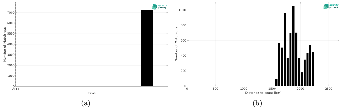
Figure 1: Number of match-ups between TSG (GOSUD-Sailing-ship) and SMOS SSS L4 v1 - Monthly (CMEMS-CNR) SSS as a function of time (a) and as function of the distance to coast (b) over the SPURS 2 Pi-MEP region and for the full satellite product period.
