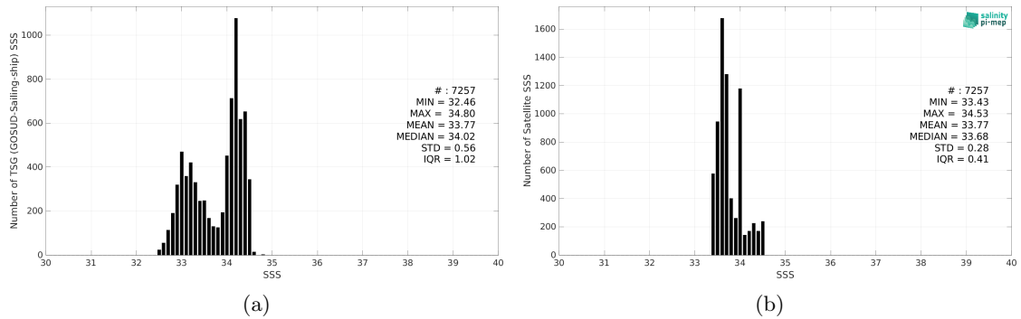
Figure 2: Histograms of SSS from TSG (GOSUD-Sailing-ship) (a) and SMOS SSS L4 v1 - Monthly (CMEMS-CNR) (b) considering all match-up pairs per bins of 0.1 over the SPURS 2 Pi-MEP region and for the full satellite product period.
