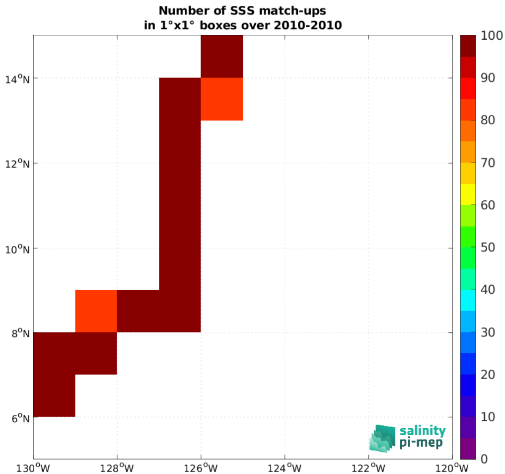
Figure 4: Number of SSS match-ups between TSG (GOSUD-Sailing-ship) SSS and the SMOS SSS L4 v1 - Monthly (CMEMS-CNR) SSS product for the SPURS 2 Pi-MEP region over 1°x1° boxes and for the full satellite product period.
