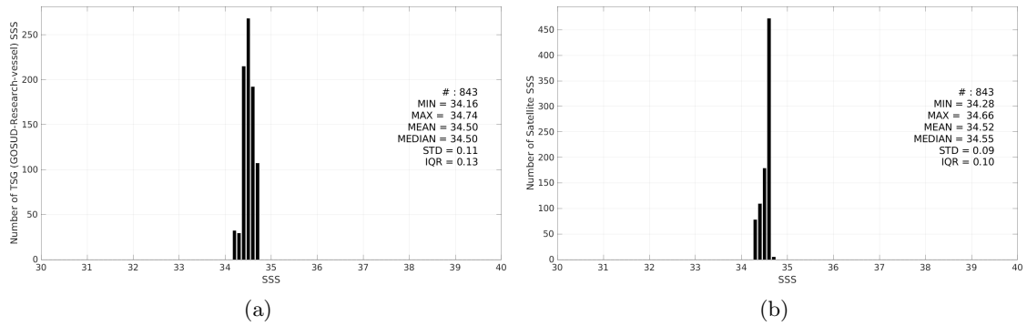
Figure 3: Histograms of SSS from TSG (GOSUD-Research-vessel) (a) and SMOS SSS L4 v1 - Monthly (CMEMS-CNR) (b) considering all match-up pairs per bins of 0.1 over the SPURS 2 Pi-MEP region and for the full satellite product period.
