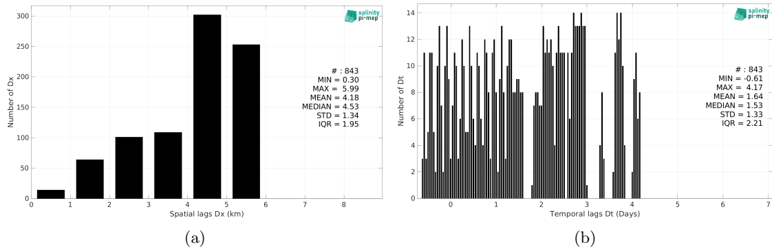
Figure 6: Histograms of the spatial (a) and temporal (b) lags between the location/time of the TSG (GOSUD-Research-vessel) measurement and the date of the corresponding SMOS SSS L4 v1 - Monthly (CMEMS-CNR) SSS pixel.
