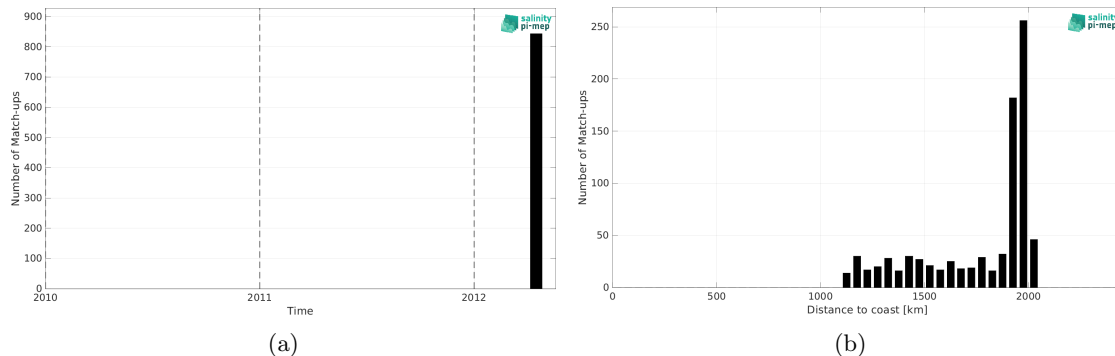
Figure 2: Number of match-ups between TSG (GOSUD-Research-vessel) and SMOS SSS L4 v1 - Monthly (CMEMS-CNR) SSS as a function of time (a) and as function of the distance to coast (b) over the SPURS 2 Pi-MEP region and for the full satellite product period.
