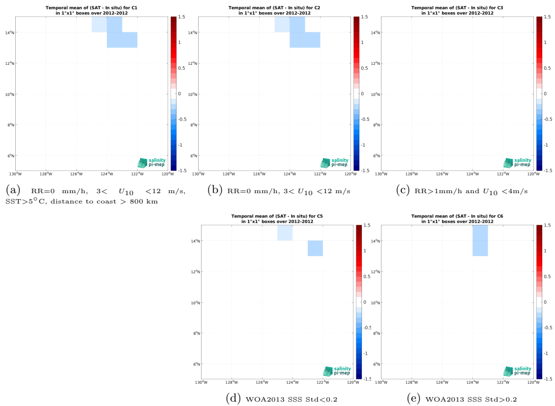
Figure 14: Temporal mean gridded over spatial boxes of size 1^\circ \times 1^\circ of \Delta SSS (SMOS SSS L4 v1 - Monthly (CMEMS-CNR) - TSG (GOSUD-Research-vessel)) for 5 different subdatasets corresponding to: RR=0 mm/h, 3 < U_{10} < 12 m/s, SST > 5^\circ\text{C} , distance to coast > 800 km (a), RR=0 mm/h, 3 < U_{10} < 12 m/s (b), RR > 1 mm/h and U_{10} < 4 m/s (c), WOA2013 SSS Std < 0.2 (d), WOA2013 SSS Std > 0.2 (e).
