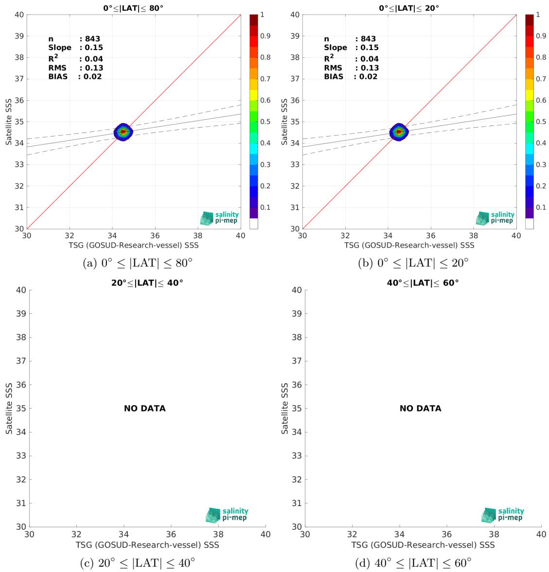
Figure 10: Contour maps of the concentration of SMOS SSS L4 v1 - Monthly (CMEMS-CNR) SSS (y-axis) versus TSG (GOSUD-Research-vessel) SSS (x-axis) at match-up pairs for different latitude bands. For each plot, the red line shows x=y . The black thin and dashed lines indicate a linear fit through the data cloud and the \pm 95\% confidence levels, respectively. The number match-up pairs n , the slope and R^2 coefficient of the linear fit, the root mean square (RMS) and the mean bias between satellite and in situ data are indicated for each latitude band in each plots.
