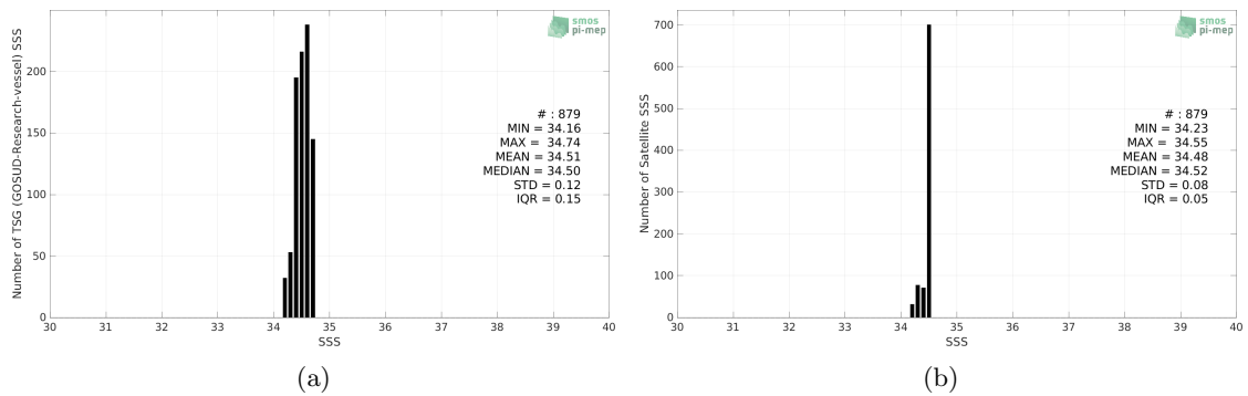
Figure 2: Histograms of SSS from TSG (GOSUD-Research-vessel) (a) and SMOS SSS L4 v1 - Monthly (CMEMS-CNR) (b) considering all match-up pairs per bins of 0.1 over the SPURS 2 Pi-MEP region and for the full satellite product period.
