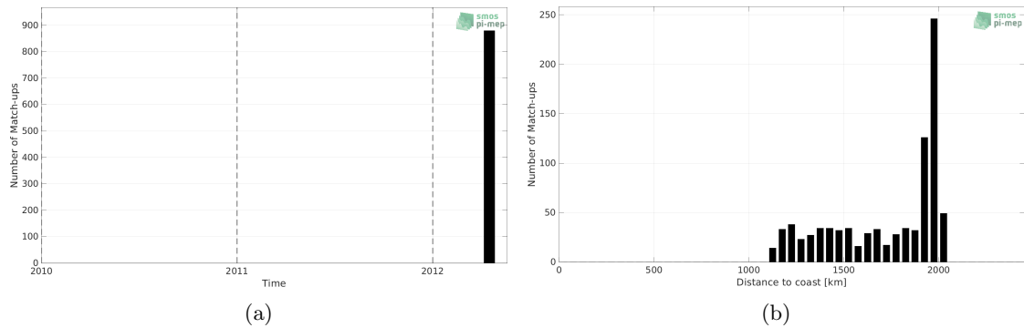
Figure 1: Number of match-ups between TSG (GOSUD-Research-vessel) and SMOS SSS L4 v1 - Monthly (CMEMS-CNR) SSS as a function of time (a) and as function of the distance to coast (b) over the SPURS 2 Pi-MEP region and for the full satellite product period.
