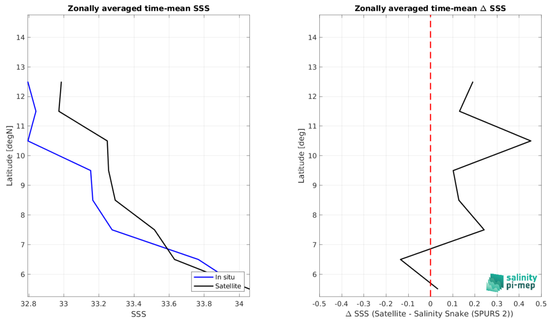
Figure 9: Left panel: Zonal mean SSS from SMOS SSS L4 v1 - Monthly (CMEMS-CNR) satellite product (black) and from Salinity Snake (SPURS 2) (blue). Right panel: Zonal mean of \Delta SSS (Satellite - Salinity Snake (SPURS 2)) for all the collected Pi-MEP match-up pairs estimated over the full satellite product period.
