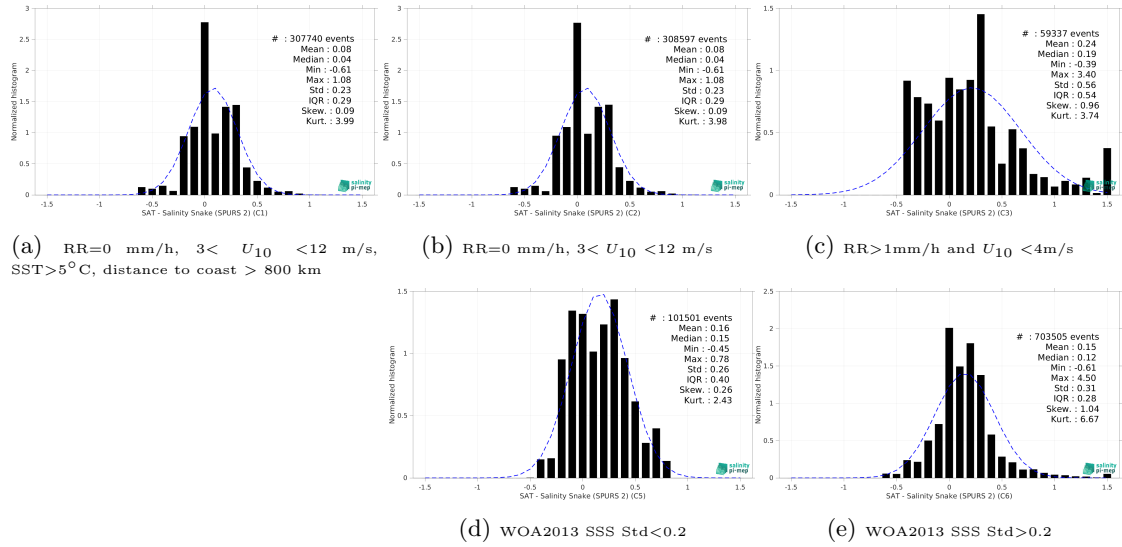
Figure 15: Normalized histogram of \Delta SSS (SMOS SSS L4 v1 - Monthly (CMEMS-CNR) - Salinity Snake (SPURS 2)) for 5 different subdatasets corresponding to: RR=0 mm/h, 3 < U_{10} < 12 m/s, SST > 5°C, distance to coast > 800 km (a), RR=0 mm/h, 3 < U_{10} < 12 m/s (b), RR > 1mm/h and U_{10} < 4 m/s (c), WOA2013 SSS Std < 0.2 (d), WOA2013 SSS Std > 0.2 (e).
