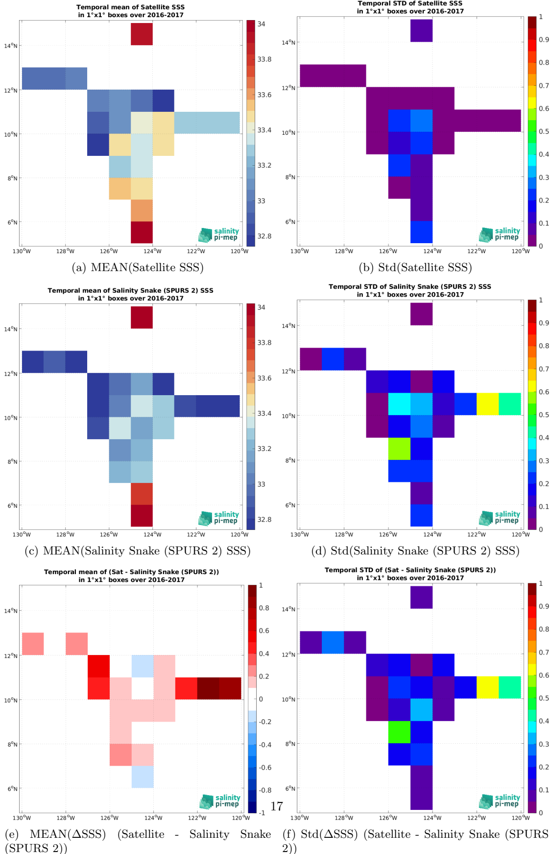
Figure 7: Temporal mean (left) and Std (right) of SSS from SMOS SSS L4 v1 - Monthly (CMEMS-CNR) (top), Salinity Snake (SPURS 2) (middle), and of \Delta SSS (Satellite - Salinity Snake (SPURS 2)). Only match-up pairs are used to generate these maps.
