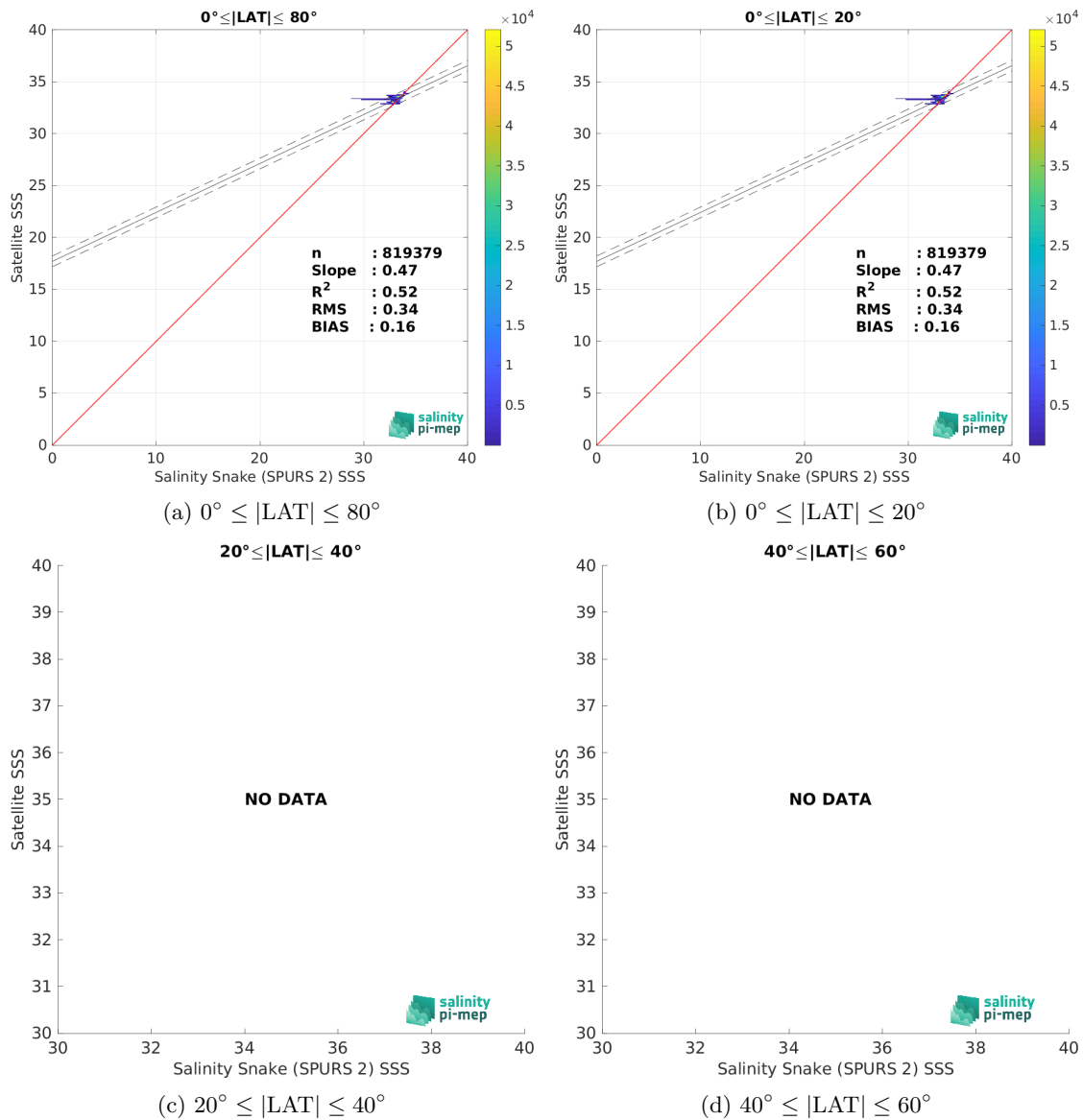
Figure 10: Contour maps of the concentration of SMOS SSS L4 v1 - Monthly (CMEMS-CNR) SSS (y-axis) versus Salinity Snake (SPURS 2) SSS (x-axis) at match-up pairs for different latitude bands. For each plot, the red line shows x=y . The black thin and dashed lines indicate a linear fit through the data cloud and the \pm 95\% confidence levels, respectively. The number match-up pairs n , the slope and R^2 coefficient of the linear fit, the root mean square (RMS) and the mean bias between satellite and in situ data are indicated for each latitude band in each plots.
