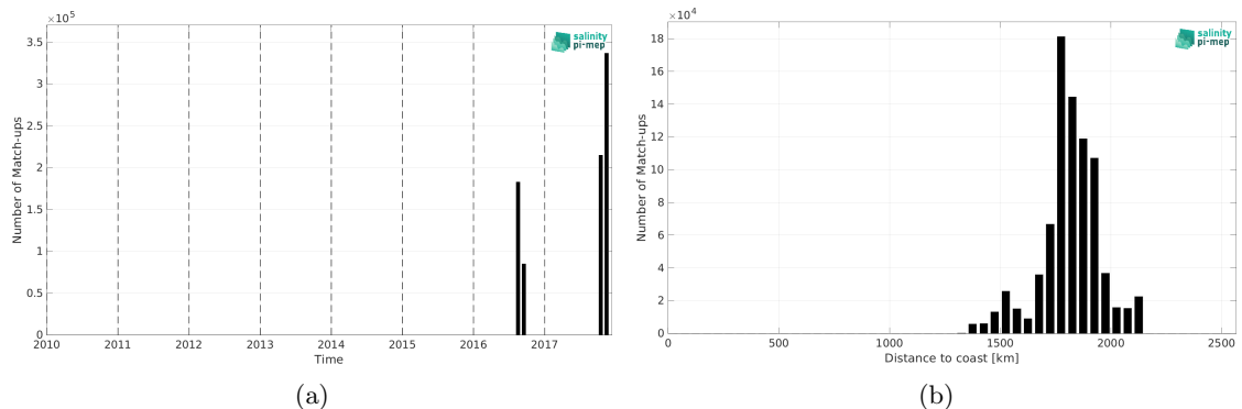
Figure 2: Number of match-ups between Salinity Snake (SPURS 2) and SMOS SSS L4 v1 - Monthly (CMEMS-CNR) SSS as a function of time (a) and as function of the distance to coast (b) over the SPURS 2 Pi-MEP region and for the full satellite product period.
