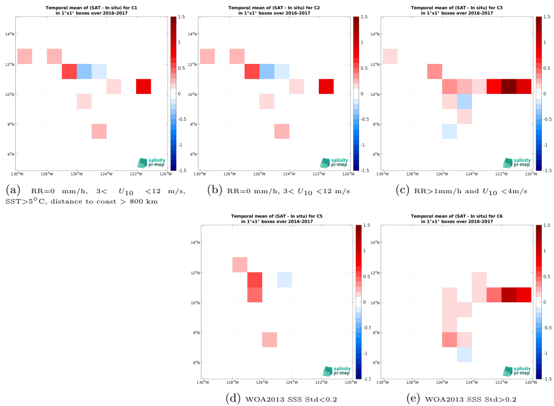
Figure 14: Temporal mean gridded over spatial boxes of size 1^\circ \times 1^\circ of \Delta SSS (SMOS SSS L4 v1 - Monthly (CMEMS-CNR) - Salinity Snake (SPURS 2)) for 5 different subdatasets corresponding to:RR=0 mm/h, 3 < U_{10} < 12 m/s, SST >5^\circ\text{C} , distance to coast > 800 km (a), RR=0 mm/h, 3 < U_{10} < 12 m/s (b), RR >1 mm/h and U_{10} < 4 m/s (c), WOA2013 SSS Std <0.2 (d), WOA2013 SSS Std >0.2 (e).
