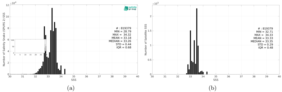
Figure 3: Histograms of SSS from Salinity Snake (SPURS 2) (a) and SMOS SSS L4 v1 - Monthly (CMEMS-CNR) (b) considering all match-up pairs per bins of 0.1 over the SPURS 2 Pi-MEP region and for the full satellite product period.
