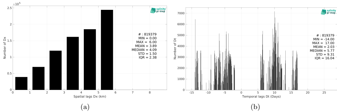
Figure 6: Histograms of the spatial (a) and temporal (b) lags between the location/time of the Salinity Snake (SPURS 2) measurement and the date of the corresponding SMOS SSS L4 v1 - Monthly (CMEMS-CNR) SSS pixel.
