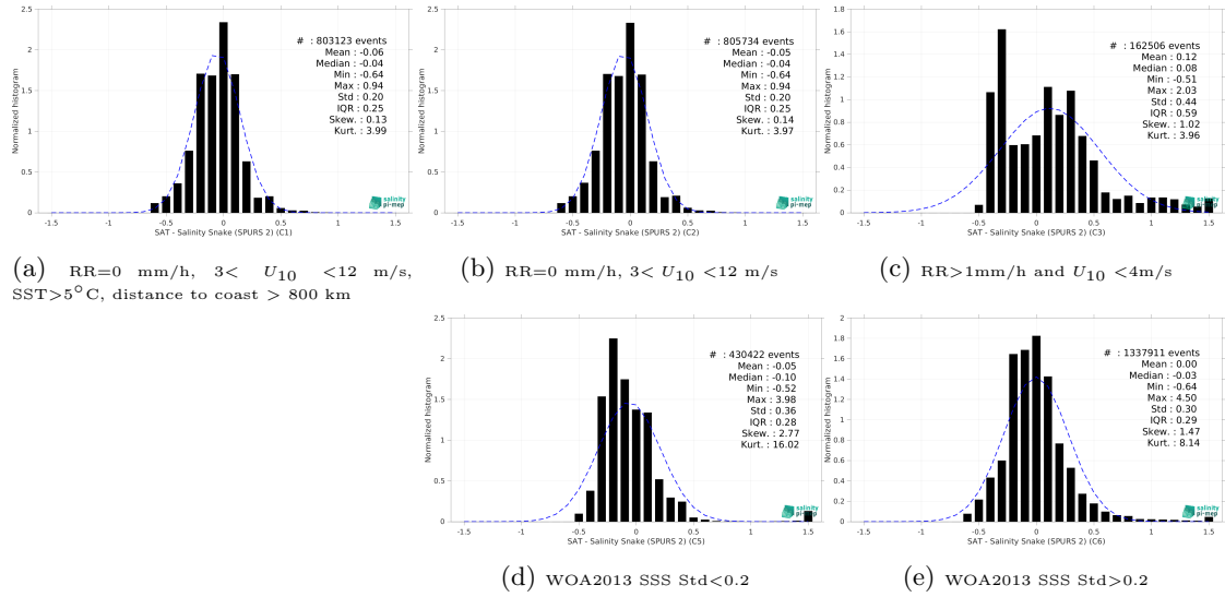
Figure 13: Normalized histogram of \Delta SSS (SMOS SSS L4 v1 - Monthly (CMEMS-CNR) - Salinity Snake (SPURS 2)) for 5 different subdatasets corresponding to: RR=0 mm/h, 3 < U_{10} < 12 m/s, SST > 5°C, distance to coast > 800 km (a), RR=0 mm/h, 3 < U_{10} < 12 m/s (b), RR > 1mm/h and U_{10} < 4 m/s (c), WOA2013 SSS Std < 0.2 (d), WOA2013 SSS Std > 0.2 (e).
