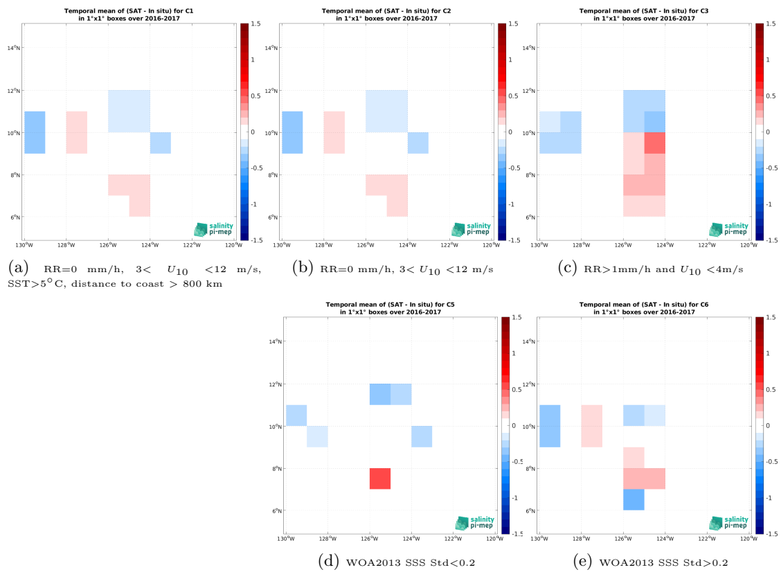
Figure 12: Temporal mean gridded over spatial boxes of size 1^\circ \times 1^\circ of \Delta\text{SSS} (SMOS SSS L4 v1 - Monthly (CMEMS-CNR) - Salinity Snake (SPURS 2)) for 5 different subdatasets corresponding to:RR=0 mm/h, 3 < U_{10} < 12 m/s, SST >5^\circ\text{C} , distance to coast > 800 km (a), RR=0 mm/h, 3 < U_{10} < 12 m/s (b), RR >1 mm/h and U_{10} < 4 m/s (c), WOA2013 SSS Std <0.2 (d), WOA2013 SSS Std >0.2 (e).
