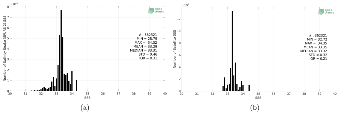
Figure 2: Histograms of SSS from Salinity Snake (SPURS 2) (a) and SMOS SSS L4 v1 - Monthly (CMEMS-CNR) (b) considering all match-up pairs per bins of 0.1 over the SPURS 2 Pi-MEP region and for the full satellite product period.
