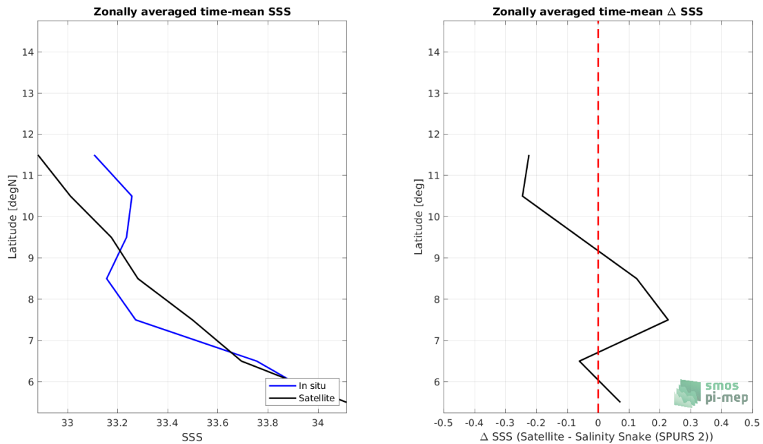
Figure 8: Left panel: Zonal mean SSS from SMOS SSS L4 v1 - Monthly (CMEMS-CNR) satellite product (black) and from Salinity Snake (SPURS 2) (blue). Right panel: Zonal mean of \Delta SSS (Satellite - Salinity Snake (SPURS 2)) for all the collected Pi-MEP match-up pairs estimated over the full satellite product period.
