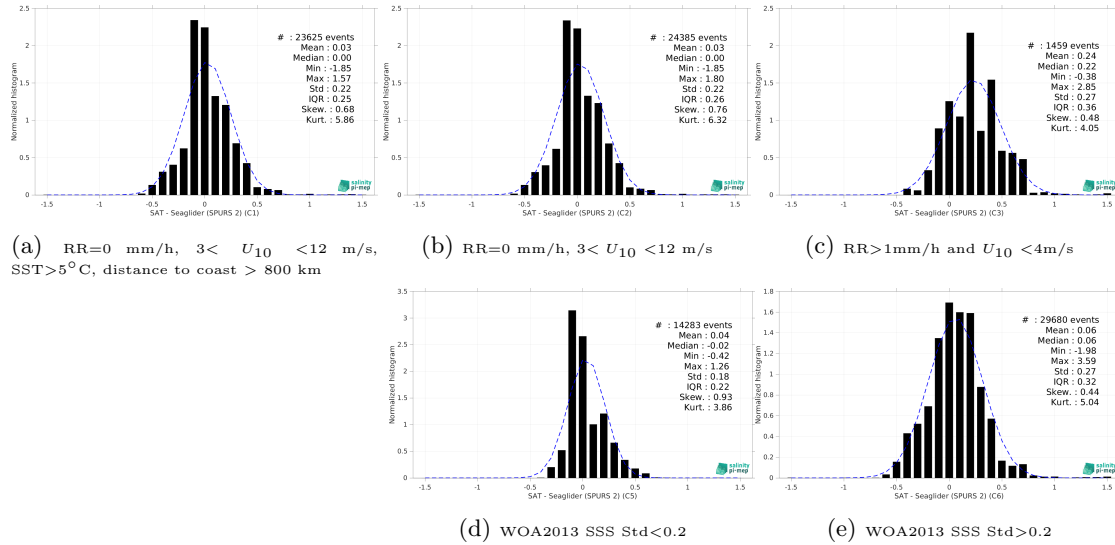
Figure 15: Normalized histogram of \Delta SSS (SMOS SSS L4 v1 - Monthly (CMEMS-CNR) - Seaglider (SPURS 2)) for 5 different subdatasets corresponding to: RR=0 mm/h, 3 < U_{10} < 12 m/s, SST>5°C, distance to coast > 800 km (a), RR=0 mm/h, 3 < U_{10} < 12 m/s (b), RR>1mm/h and U_{10} < 4 m/s (c), WOA2013 SSS Std<0.2 (d), WOA2013 SSS Std>0.2 (e).
