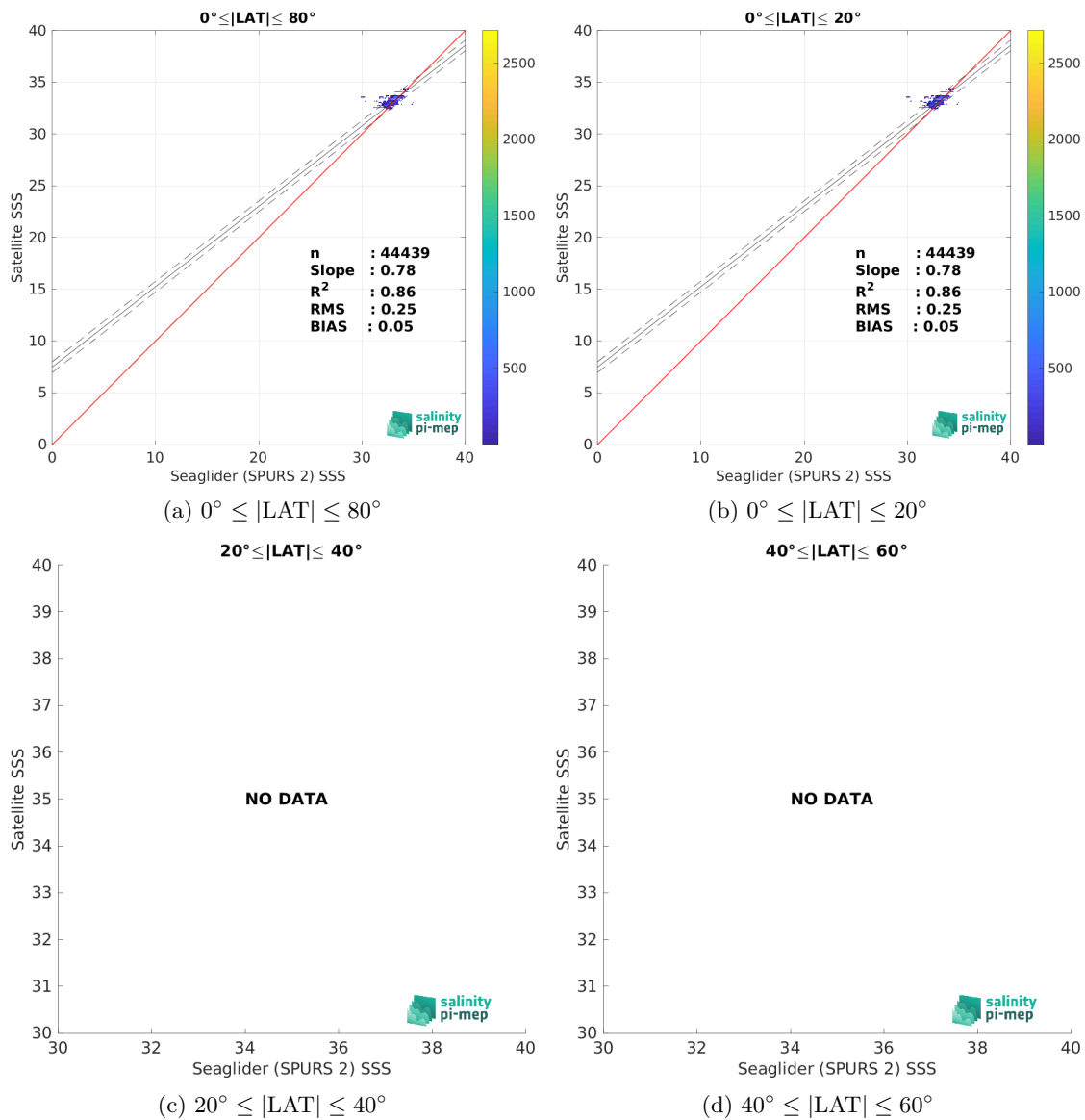
Figure 10: Contour maps of the concentration of SMOS SSS L4 v1 - Monthly (CMEMS-CNR) SSS (y-axis) versus Seaglider (SPURS 2) SSS (x-axis) at match-up pairs for different latitude bands. For each plot, the red line shows x=y . The black thin and dashed lines indicate a linear fit through the data cloud and the \pm 95\% confidence levels, respectively. The number match-up pairs n , the slope and R^2 coefficient of the linear fit, the root mean square (RMS) and the mean bias between satellite and in situ data are indicated for each latitude band in each plots.
