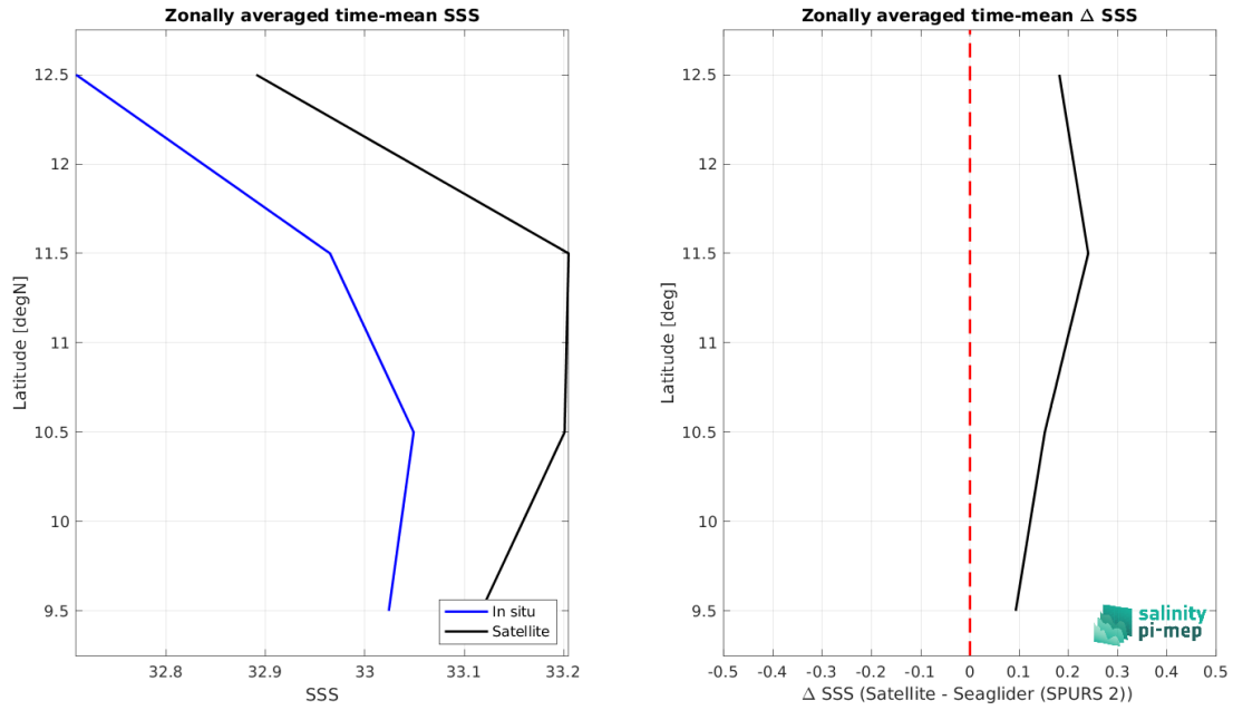
Figure 9: Left panel: Zonal mean SSS from SMOS SSS L4 v1 - Monthly (CMEMS-CNR) satellite product (black) and from Seaglider (SPURS 2) (blue). Right panel: Zonal mean of \Delta SSS (Satellite - Seaglider (SPURS 2)) for all the collected Pi-MEP match-up pairs estimated over the full satellite product period.
