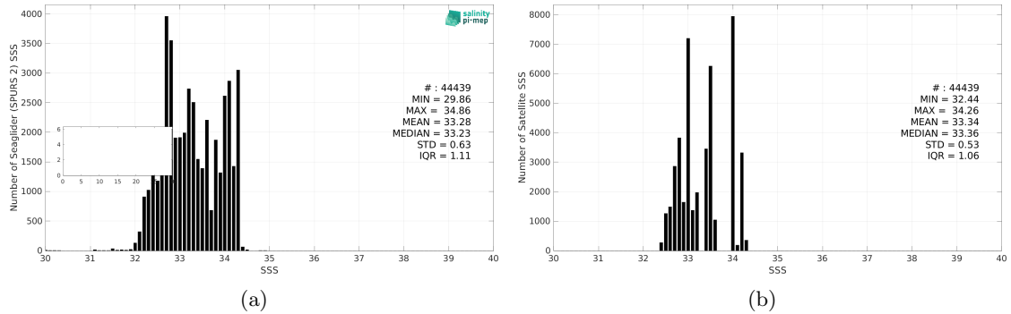
Figure 3: Histograms of SSS from Seaglider (SPURS 2) (a) and SMOS SSS L4 v1 - Monthly (CMEMS-CNR) (b) considering all match-up pairs per bins of 0.1 over the SPURS 2 Pi-MEP region and for the full satellite product period.
