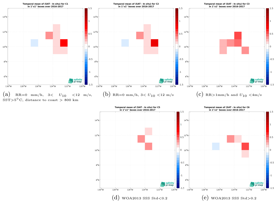
Figure 14: Temporal mean gridded over spatial boxes of size 1^\circ \times 1^\circ of \Delta SSS (SMOS SSS L4 v1 - Monthly (CMEMS-CNR) - Seaglider (SPURS 2)) for 5 different subdatasets corresponding to:RR=0 mm/h, 3 < U_{10} < 12 m/s, SST >5^\circ C, distance to coast > 800 km (a), RR=0 mm/h, 3 < U_{10} < 12 m/s (b), RR >1 mm/h and U_{10} < 4 m/s (c), WOA2013 SSS Std <0.2 (d), WOA2013 SSS Std >0.2 (e).
