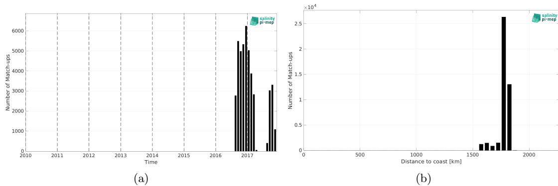
Figure 2: Number of match-ups between Seaglider (SPURS 2) and SMOS SSS L4 v1 - Monthly (CMEMS-CNR) SSS as a function of time (a) and as function of the distance to coast (b) over the SPURS 2 Pi-MEP region and for the full satellite product period.
