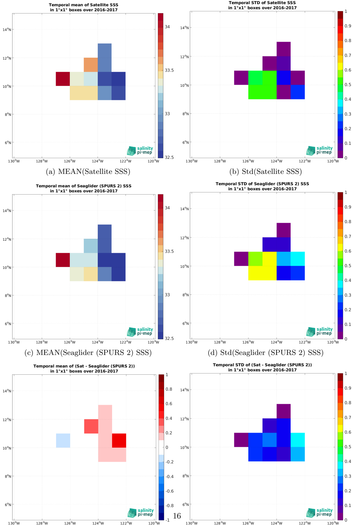
Figure 7: Temporal mean (left) and Std (right) of SSS from SMOS SSS L4 v1 - Monthly (CMEMS-CNR) (top), Seaglider (SPURS 2) (middle), and of \Delta SSS (Satellite - Seaglider (SPURS 2)). Only match-up pairs are used to generate these maps.
