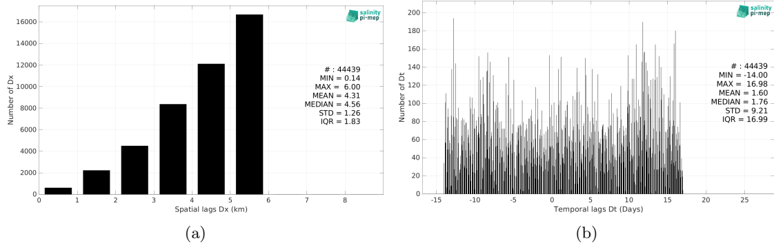
Figure 6: Histograms of the spatial (a) and temporal (b) lags between the location/time of the Seaglider (SPURS 2) measurement and the date of the corresponding SMOS SSS L4 v1 - Monthly (CMEMS-CNR) SSS pixel.
