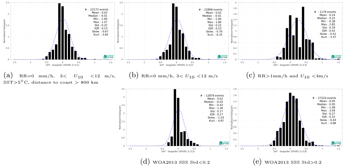
Figure 15: Normalized histogram of \Delta SSS (SMOS SSS L4 v1 - Monthly (CMEMS-CNR) - Seaglider (SPURS 2)) for 5 different subdatasets corresponding to: RR=0 mm/h, 3 < U_{10} < 12 m/s, SST > 5°C, distance to coast > 800 km (a), RR=0 mm/h, 3 < U_{10} < 12 m/s (b), RR > 1mm/h and U_{10} < 4 m/s (c), WOA2013 SSS Std < 0.2 (d), WOA2013 SSS Std > 0.2 (e).
