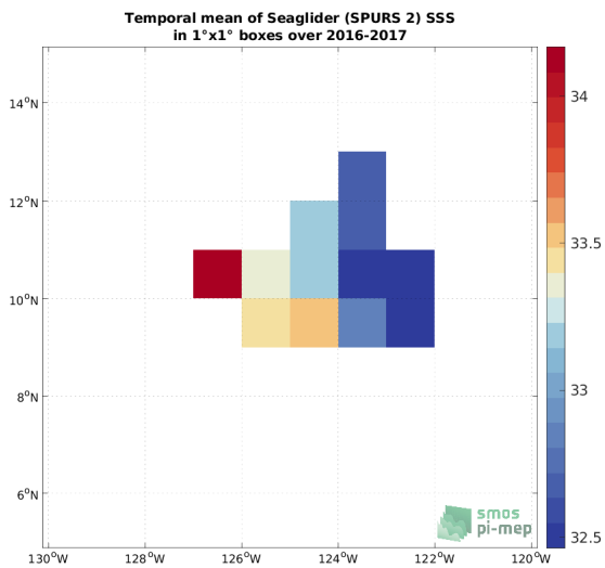
(c) MEAN(Seaglider (SPURS 2) SSS)
