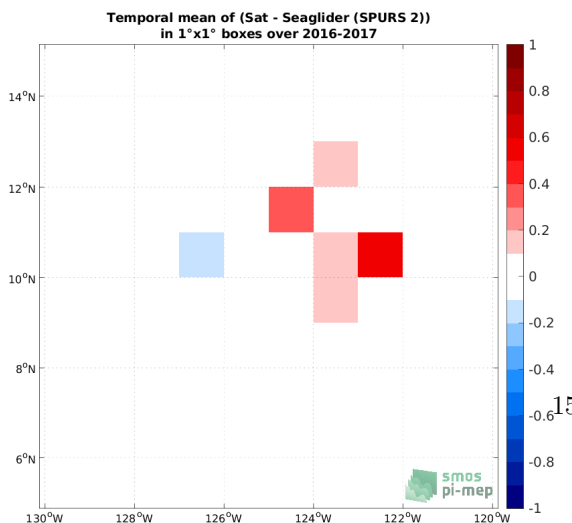
(e) MEAN( \Delta SSS) (Satellite - Seaglider (SPURS 2))
