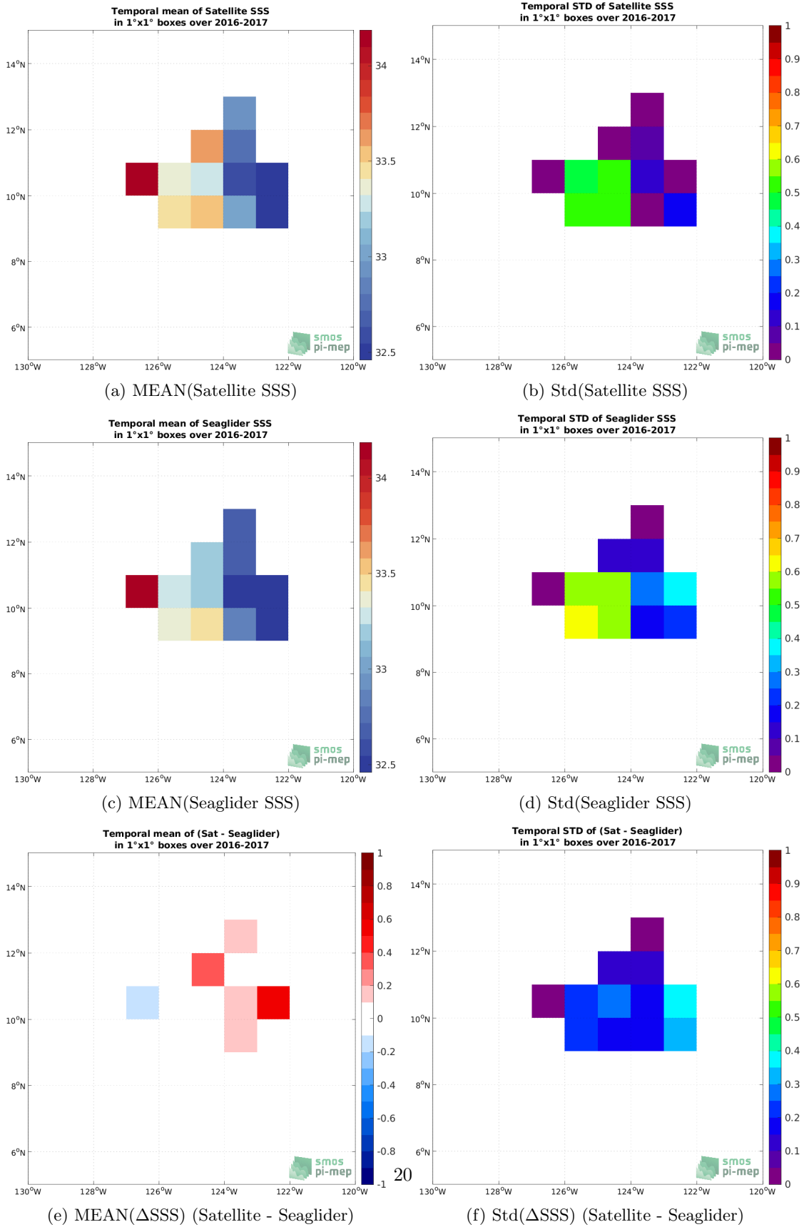
Figure 5: Temporal mean (left) and Std (right) of SSS from SMOS SSS L4 v1 - Monthly (CMEMS-CNR) (top), Seaglider (middle), and of \Delta SSS (Satellite - Seaglider). Only match-up pairs are used to generate these maps.
