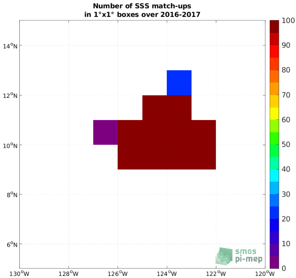
Figure 3: Number of SSS match-ups between Seaglider SSS and the SMOS SSS L4 v1 - Monthly (CMEMS-CNR) SSS product for the SPURS 2 Pi-MEP region over 1°×1° boxes and for the full satellite product period.
