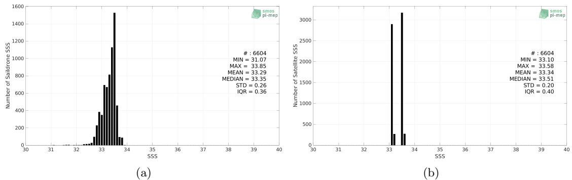
Figure 2: Histograms of SSS from Saildrone (a) and SMOS SSS L4 v1 - Monthly (CMEMS-CNR) (b) considering all match-up pairs per bins of 0.1 over the SPURS 2 Pi-MEP region and for the full satellite product period.
