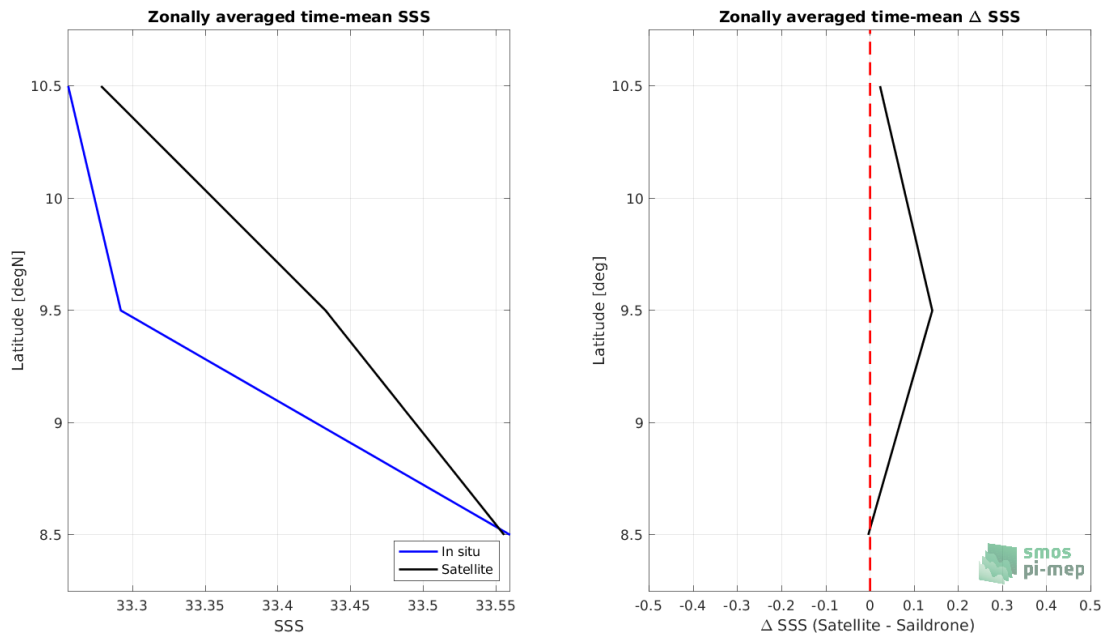
Figure 7: Left panel: Zonal mean SSS from SMOS SSS L4 v1 - Monthly (CMEMS-CNR) satellite product (black) and from Sairdrone (blue). Right panel: Zonal mean of \Delta SSS (Satellite - Sairdrone) for all the collected Pi-MEP match-up pairs estimated over the full satellite product period.
