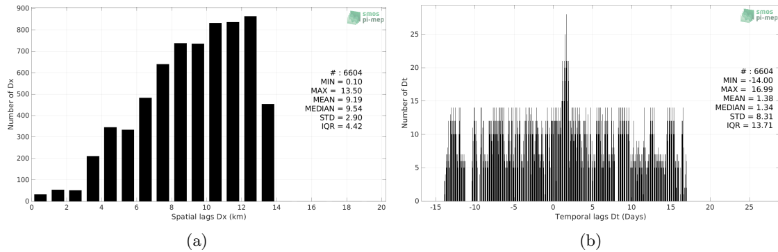
Figure 4: Histograms of the spatial (a) and temporal (b) lags between the location/time of the Saildrone measurement and the date of the corresponding SMOS SSS L4 v1 - Monthly (CMEMS-CNR) SSS pixel.
