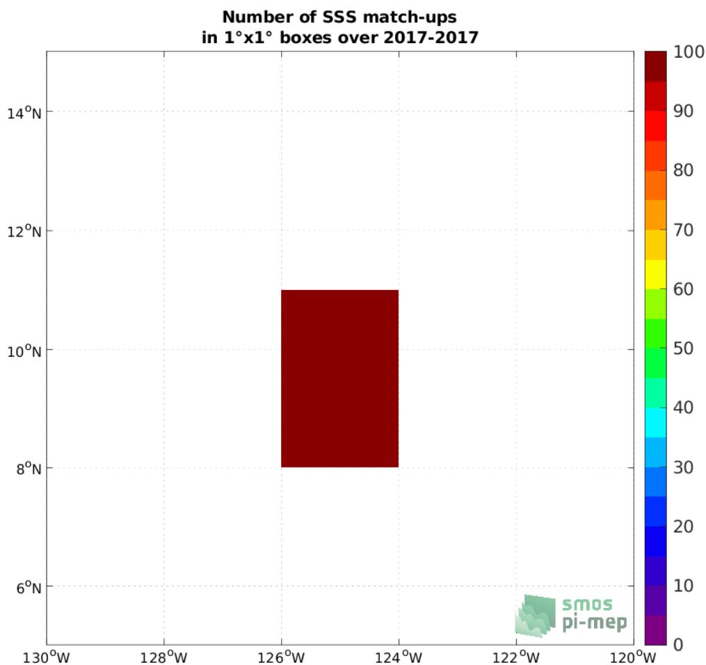
Figure 3: Number of SSS match-ups between Saildrone SSS and the SMOS SSS L4 v1 - Monthly (CMEMS-CNR) SSS product for the SPURS 2 Pi-MEP region over 1°×1° boxes and for the full satellite product period.
