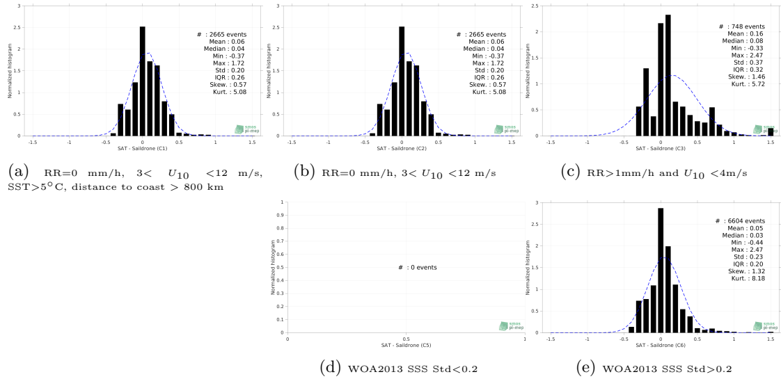
Figure 12: Normalized histogram of \Delta SSS (SMOS SSS L4 v1 - Monthly (CMEMS-CNR) - Saildrone) for 5 different subdatasets corresponding to: RR=0 mm/h, 3 < U_{10} < 12 m/s, SST > 5°C, distance to coast > 800 km (a), RR=0 mm/h, 3 < U_{10} < 12 m/s (b), RR > 1mm/h and U_{10} < 4 m/s (c), WOA2013 SSS Std < 0.2 (d), WOA2013 SSS Std > 0.2 (e).
