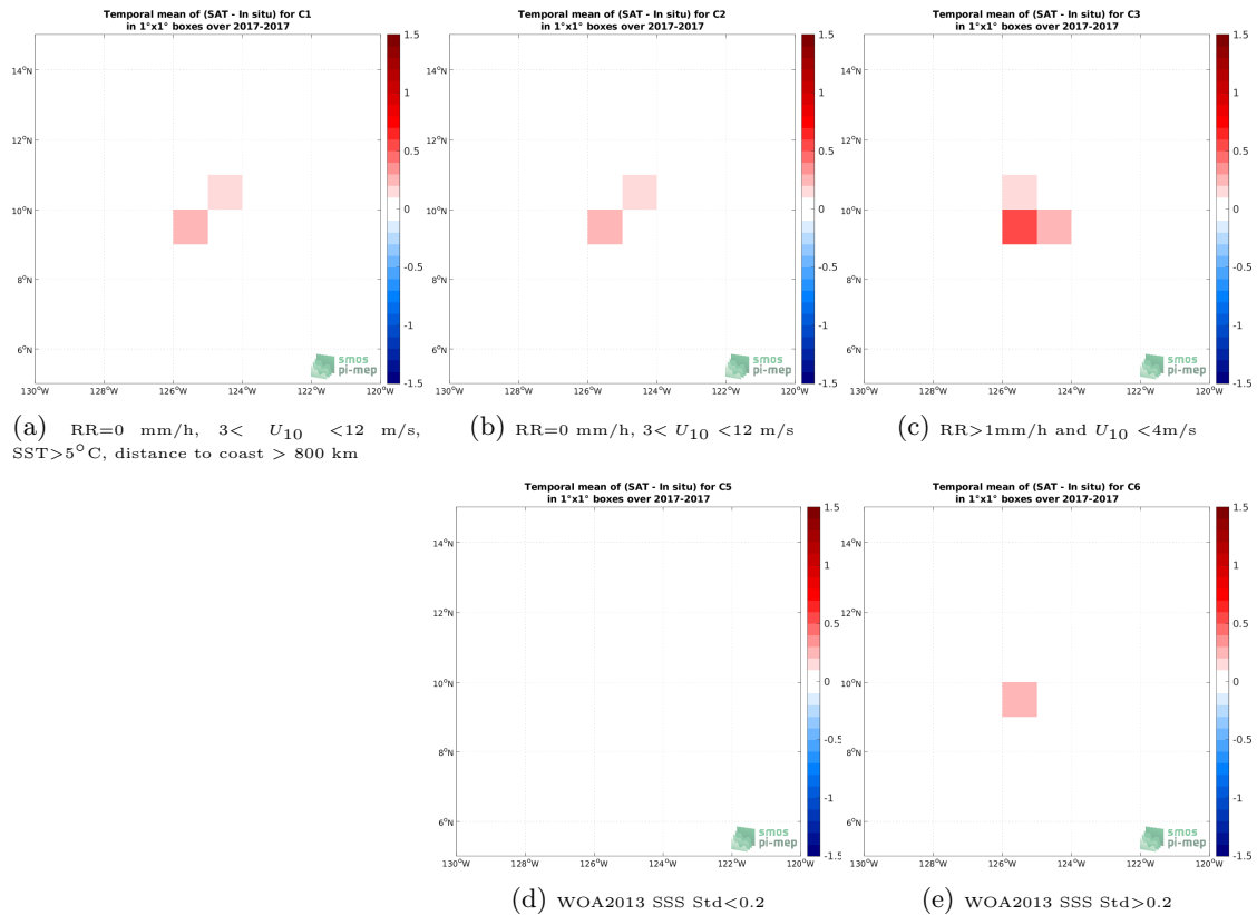
Figure 11: Temporal mean gridded over spatial boxes of size 1^\circ \times 1^\circ of \Delta SSS (SMOS SSS L4 v1 - Monthly (CMEMS-CNR) - Saildrone) for 5 different subdatasets corresponding to:RR=0 mm/h, 3 < U_{10} < 12 m/s, SST >5^\circ C, distance to coast > 800 km (a), RR=0 mm/h, 3 < U_{10} < 12 m/s (b), RR >1 mm/h and U_{10} < 4 m/s (c), WOA2013 SSS Std <0.2 (d), WOA2013 SSS Std >0.2 (e).
