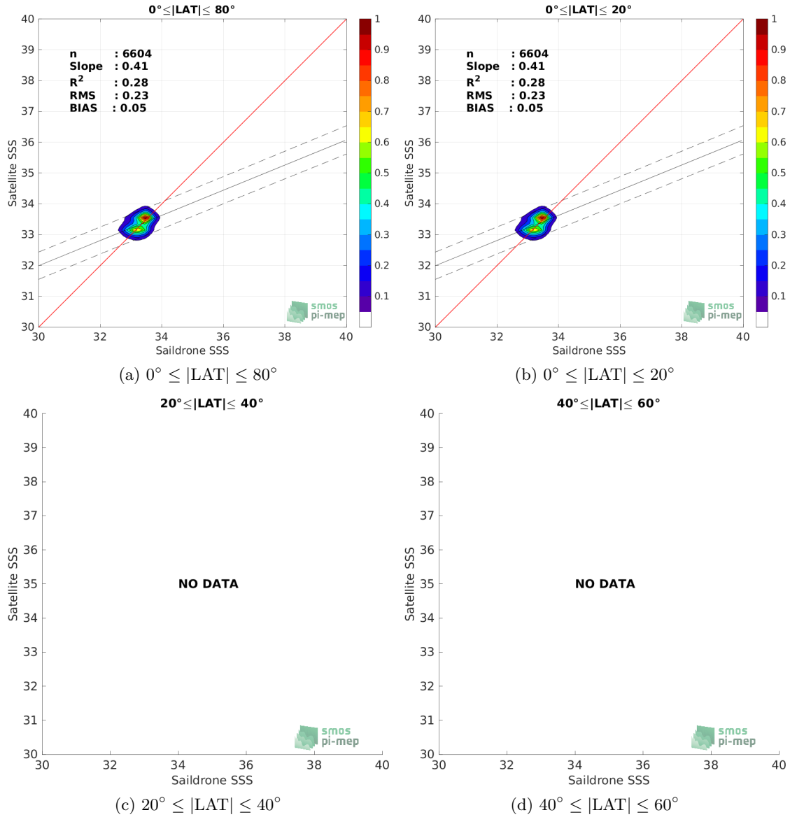
Figure 8: Contour maps of the concentration of SMOS SSS L4 v1 - Monthly (CMEMS-CNR) SSS (y-axis) versus Saïdrone SSS (x-axis) at match-up pairs for different latitude bands. For each plot, the red line shows x=y . The black thin and dashed lines indicate a linear fit through the data cloud and the \pm 95\% confidence levels, respectively. The number match-up pairs n , the slope and R^2 coefficient of the linear fit, the root mean square (RMS) and the mean bias between satellite and in situ data are indicated for each latitude band in each plots.
