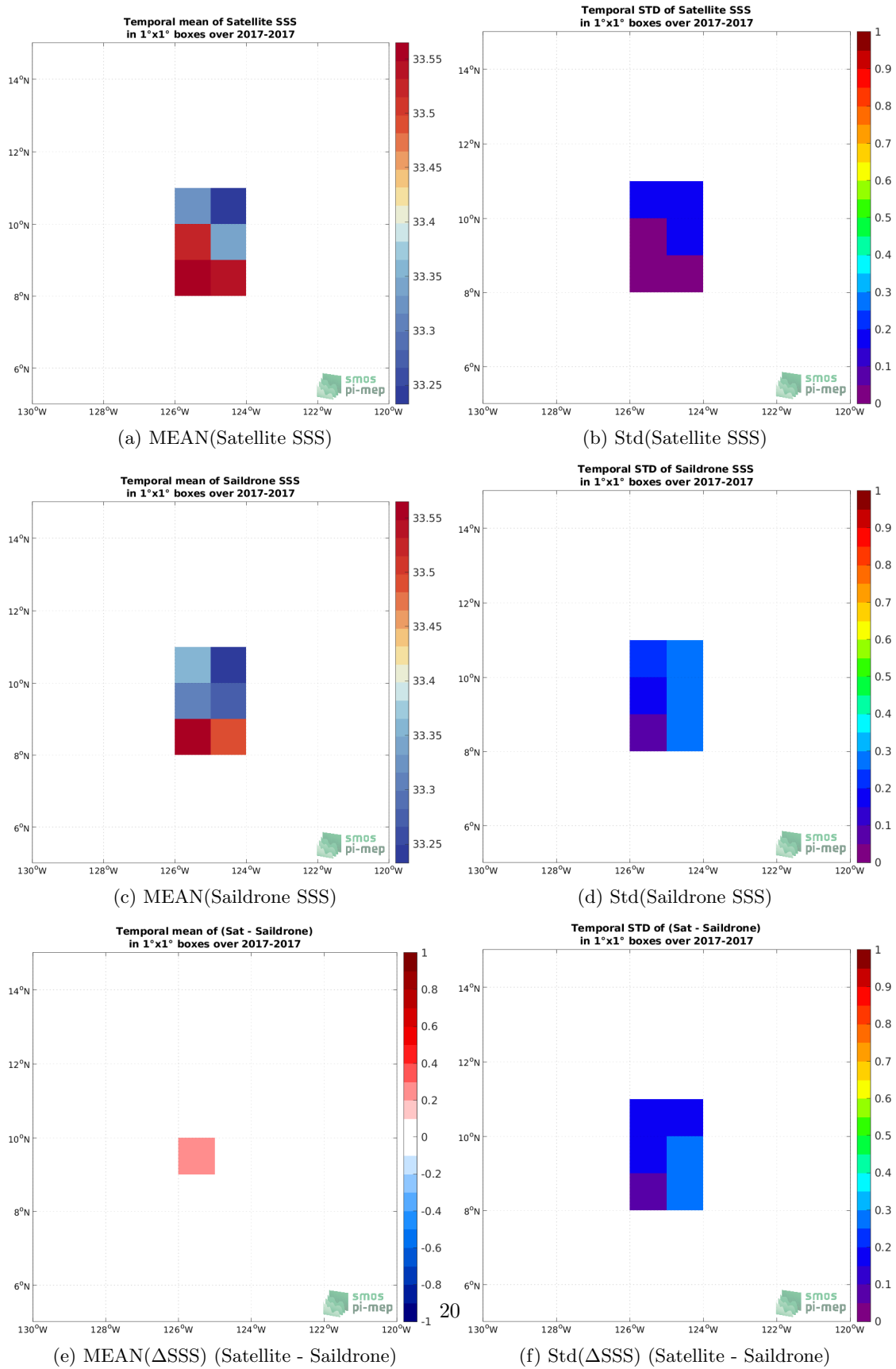
Figure 5: Temporal mean (left) and Std (right) of SSS from SMOS SSS L4 v1 - Monthly (CMEMS-CNR) (top), Saildrone (middle), and of \Delta SSS (Satellite - Saildrone). Only match-pairs are used to generate these maps.
