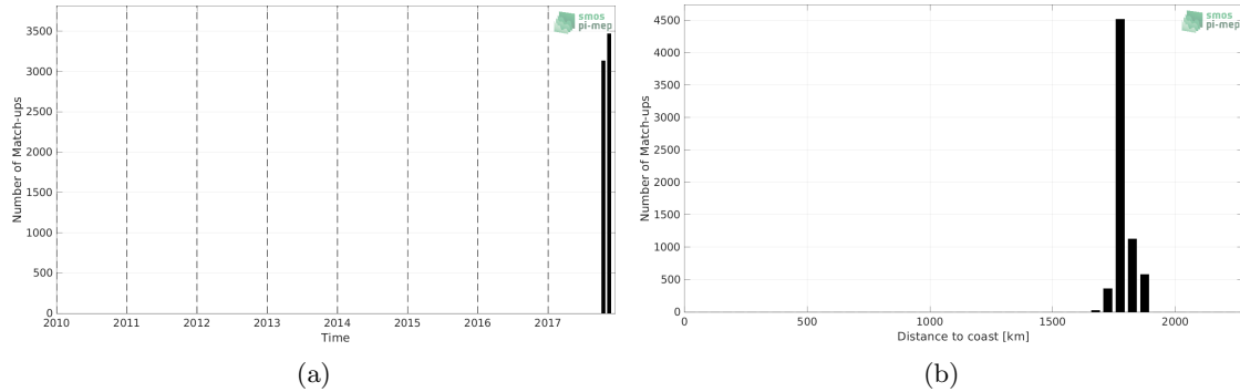
Figure 1: Number of match-ups between Saildrone and SMOS SSS L4 v1 - Monthly (CMEMS-CNR) SSS as a function of time (a) and as function of the distance to coast (b) over the SPURS 2 Pi-MEP region and for the full satellite product period.
