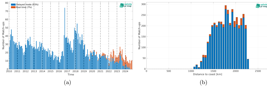
Figure 2: Number of match-ups between Argo and SMOS SSS L4 v1 - Monthly (CMEMS-CNR) SSS as a function of time (a) and as function of the distance to coast (b) over the SPURS 2 Pi-MEP region and for the full satellite product period.
