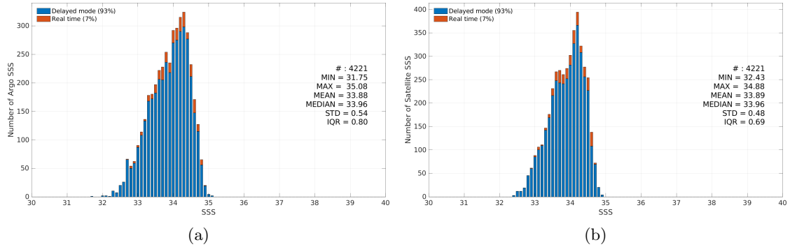
Figure 3: Histograms of SSS from Argo (a) and SMOS SSS L4 v1 - Monthly (CMEMS-CNR) (b) considering all match-up pairs per bins of 0.1 over the SPURS 2 Pi-MEP region and for the full satellite product period.
