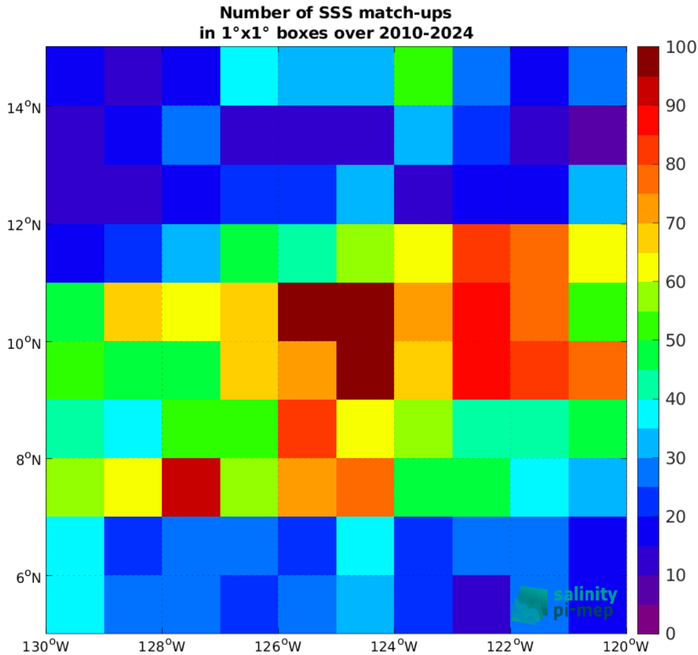
Figure 5: Number of SSS match-ups between Argo SSS and the SMOS SSS L4 v1 - Monthly (CMEMS-CNR) SSS product for the SPURS 2 Pi-MEP region over 1^\circ \times 1^\circ boxes and for the full satellite product period.
