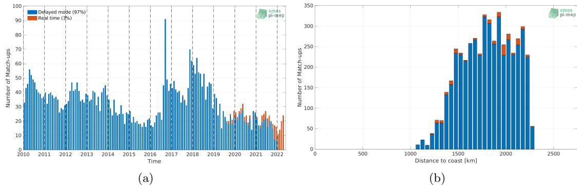
Figure 1: Number of match-ups between Argo and SMOS SSS L4 v1 - Monthly (CMEMS-CNR) SSS as a function of time (a) and as function of the distance to coast (b) over the SPURS 2 Pi-MEP region and for the full satellite product period.
