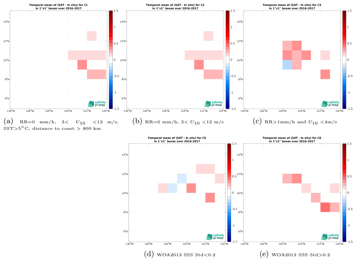
Figure 14: Temporal mean gridded over spatial boxes of size 1^\circ \times 1^\circ of \Delta SSS (SMOS SSS L4 v1 - Daily (CMEMS-CNR) - Waveglider (SPURS 2)) for 5 different subdatasets corresponding to: RR=0 mm/h, 3 < U_{10} < 12 m/s, SST > 5°C, distance to coast > 800 km (a), RR=0 mm/h, 3 < U_{10} < 12 m/s (b), RR > 1mm/h and U_{10} < 4 m/s (c), WOA2013 SSS Std < 0.2 (d), WOA2013 SSS Std > 0.2 (e).
