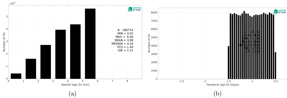
Figure 6: Histograms of the spatial (a) and temporal (b) lags between the location/time of the Waveglider (SPURS 2) measurement and the date of the corresponding SMOS SSS L4 v1 - Daily (CMEMS-CNR) SSS pixel.
