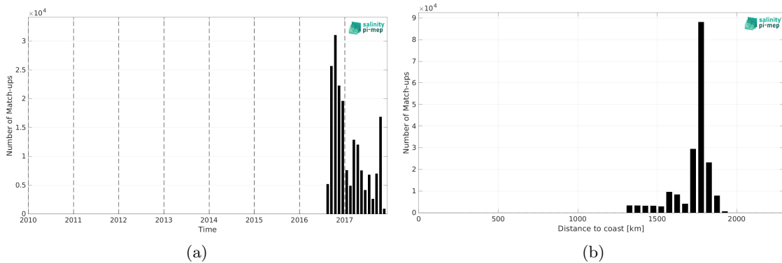
Figure 2: Number of match-ups between Waveglider (SPURS 2) and SMOS SSS L4 v1 - Daily (CMEMS-CNR) SSS as a function of time (a) and as function of the distance to coast (b) over the SPURS 2 Pi-MEP region and for the full satellite product period.
