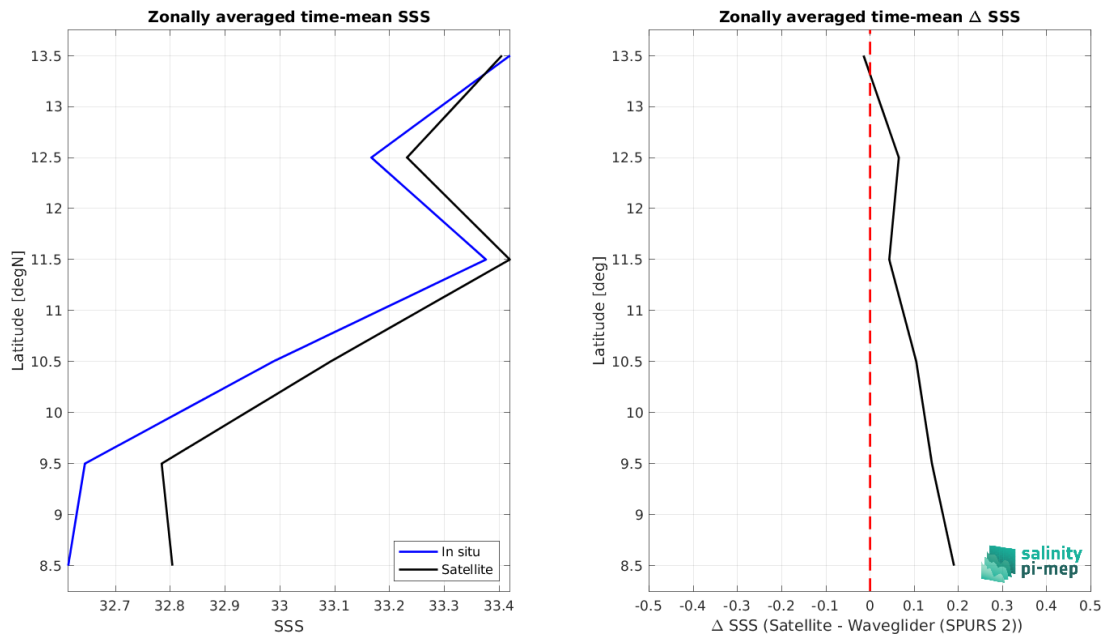
Figure 9: Left panel: Zonal mean SSS from SMOS SSS L4 v1 - Daily (CMEMS-CNR) satellite product (black) and from Waveglider (SPURS 2) (blue). Right panel: Zonal mean of \Delta SSS (Satellite - Waveglider (SPURS 2)) for all the collected Pi-MEP match-up pairs estimated over the full satellite product period.
