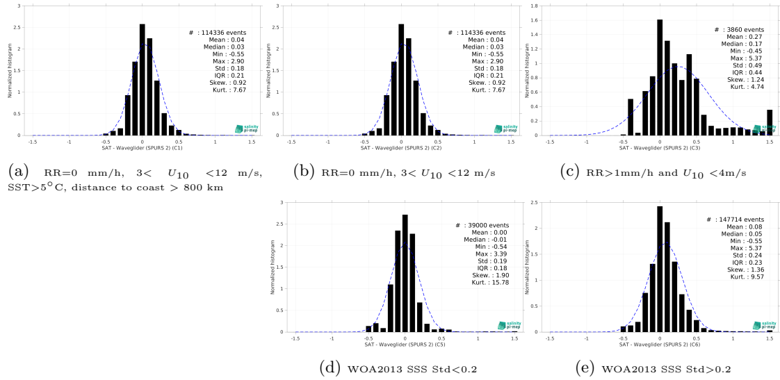
Figure 15: Normalized histogram of \Delta SSS (SMOS SSS L4 v1 - Daily (CMEMS-CNR) - Waveglider (SPURS 2)) for 5 different subdatasets corresponding to: RR=0 mm/h, 3 < U_{10} < 12 m/s, SST > 5°C, distance to coast > 800 km (a), RR=0 mm/h, 3 < U_{10} < 12 m/s (b), RR > 1mm/h and U_{10} < 4 m/s (c), WOA2013 SSS Std < 0.2 (d), WOA2013 SSS Std > 0.2 (e).
