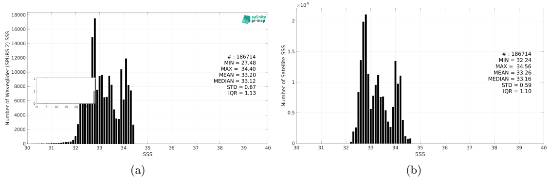
Figure 3: Histograms of SSS from Waveglider (SPURS 2) (a) and SMOS SSS L4 v1 - Daily (CMEMS-CNR) (b) considering all match-up pairs per bins of 0.1 over the SPURS 2 Pi-MEP region and for the full satellite product period.
