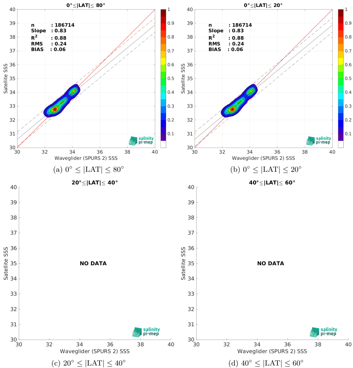
Figure 10: Contour maps of the concentration of SMOS SSS L4 v1 - Daily (CMEMS-CNR) SSS (y-axis) versus Waveglider (SPURS 2) SSS (x-axis) at match-up pairs for different latitude bands. For each plot, the red line shows x=y . The black thin and dashed lines indicate a linear fit through the data cloud and the \pm 95\% confidence levels, respectively. The number match-up pairs n , the slope and R^2 coefficient of the linear fit, the root mean square (RMS) and the mean bias between satellite and in situ data are indicated for each latitude band in each plots.
