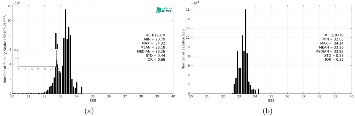
Figure 3: Histograms of SSS from Salinity Snake (SPURS 2) (a) and SMOS SSS L4 v1 - Daily (CMEMS-CNR) (b) considering all match-up pairs per bins of 0.1 over the SPURS 2 Pi-MEP region and for the full satellite product period.
