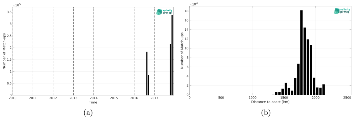
Figure 2: Number of match-ups between Salinity Snake (SPURS 2) and SMOS SSS L4 v1 - Daily (CMEMS-CNR) SSS as a function of time (a) and as function of the distance to coast (b) over the SPURS 2 Pi-MEP region and for the full satellite product period.
