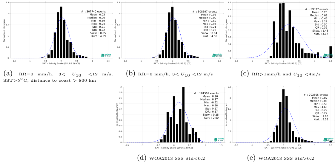
Figure 15: Normalized histogram of \Delta SSS (SMOS SSS L4 v1 - Daily (CMEMS-CNR) - Salinity Snake (SPURS 2)) for 5 different subdatasets corresponding to: RR=0 mm/h, 3 < U_{10} < 12 m/s, SST>5°C, distance to coast > 800 km (a), RR=0 mm/h, 3 < U_{10} < 12 m/s (b), RR>1mm/h and U_{10} < 4 m/s (c), WOA2013 SSS Std<0.2 (d), WOA2013 SSS Std>0.2 (e).
