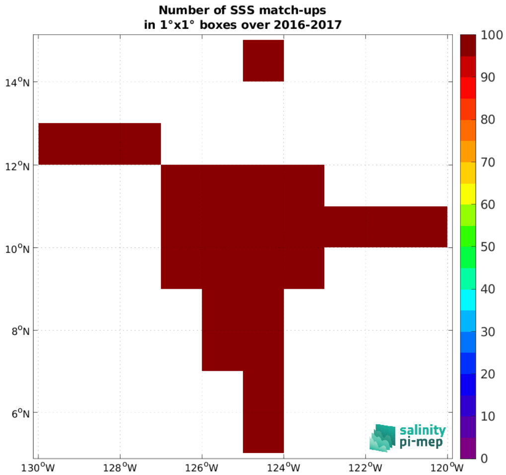
Figure 5: Number of SSS match-ups between Salinity Snake (SPURS 2) SSS and the SMOS SSS L4 v1 - Daily (CMEMS-CNR) SSS product for the SPURS 2 Pi-MEP region over 1^\circ \times 1^\circ boxes and for the full satellite product period.
