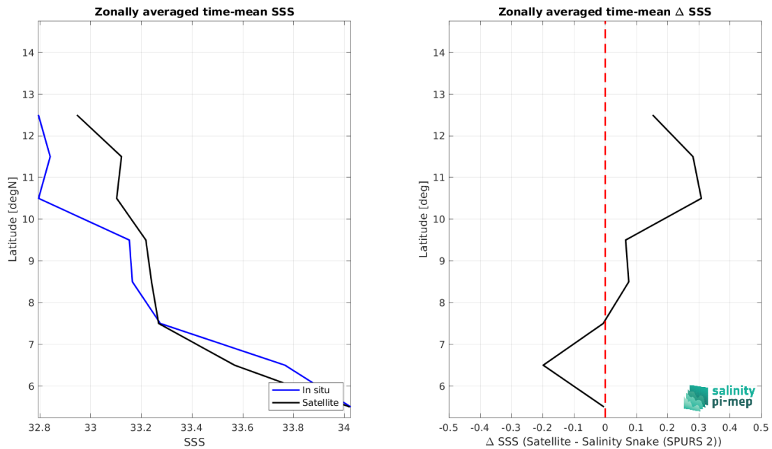
Figure 9: Left panel: Zonal mean SSS from SMOS SSS L4 v1 - Daily (CMEMS-CNR) satellite product (black) and from Salinity Snake (SPURS 2) (blue). Right panel: Zonal mean of \Delta SSS (Satellite - Salinity Snake (SPURS 2)) for all the collected Pi-MEP match-up pairs estimated over the full satellite product period.
