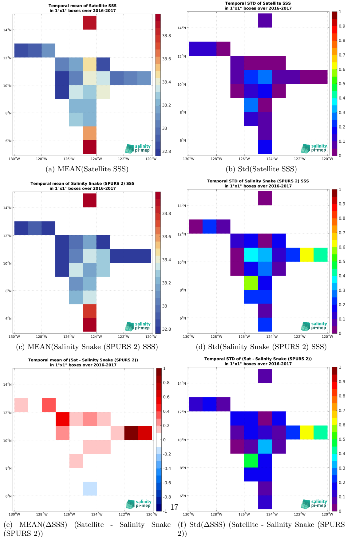
Figure 7: Temporal mean (left) and Std (right) of SSS from SMOS SSS L4 v1 - Daily (CMEMS-CNR) (top), Salinity Snake (SPURS 2) (middle), and of \Delta SSS (Satellite - Salinity Snake (SPURS 2)). Only match-up pairs are used to generate these maps.
