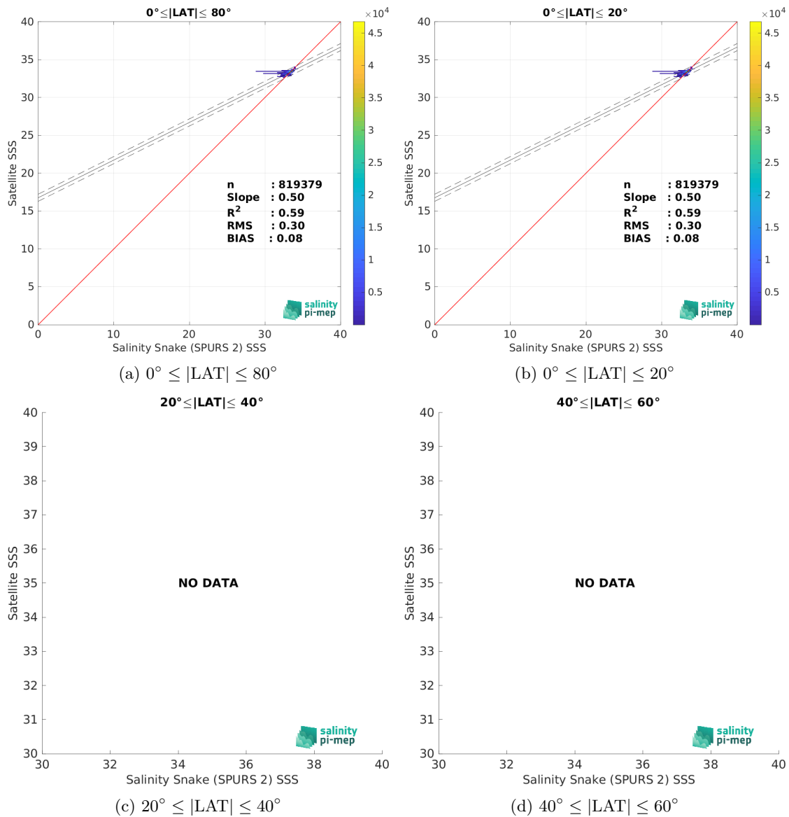
Figure 10: Contour maps of the concentration of SMOS SSS L4 v1 - Daily (CMEMS-CNR) SSS (y-axis) versus Salinity Snake (SPURS 2) SSS (x-axis) at match-up pairs for different latitude bands. For each plot, the red line shows x=y . The black thin and dashed lines indicate a linear fit through the data cloud and the \pm 95\% confidence levels, respectively. The number match-up pairs n , the slope and R^2 coefficient of the linear fit, the root mean square (RMS) and the mean bias between satellite and in situ data are indicated for each latitude band in each plots.
