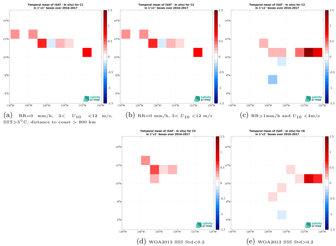
Figure 14: Temporal mean gridded over spatial boxes of size 1^\circ \times 1^\circ of \Delta SSS (SMOS SSS L4 v1 - Daily (CMEMS-CNR) - Salinity Snake (SPURS 2)) for 5 different subdatasets corresponding to:RR=0 mm/h, 3 < U_{10} < 12 m/s, SST >5^\circ C, distance to coast > 800 km (a), RR=0 mm/h, 3 < U_{10} < 12 m/s (b), RR >1 mm/h and U_{10} < 4 m/s (c), WOA2013 SSS Std <0.2 (d), WOA2013 SSS Std >0.2 (e).
