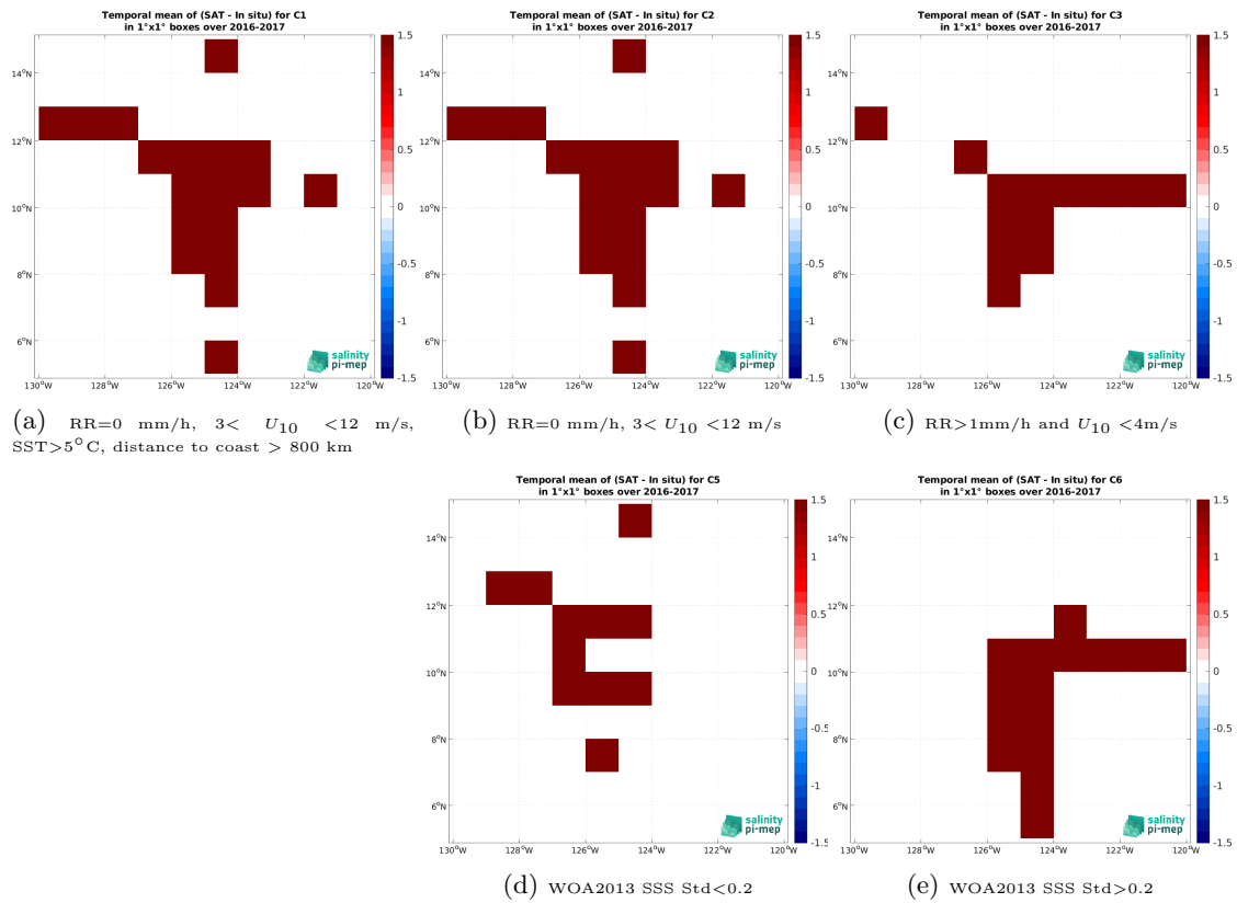
Figure 14: Temporal mean gridded over spatial boxes of size 1^\circ \times 1^\circ of \Delta\text{SSS} (SMOS SSS L4 v1 - Daily (CMEMS-CNR) - Salinity Snake (SPURS 2)) for 5 different subdatasets corresponding to: RR=0 mm/h, 3 < U_{10} < 12 m/s, SST > 5°C, distance to coast > 800 km (a), RR=0 mm/h, 3 < U_{10} < 12 m/s (b), RR > 1mm/h and U_{10} < 4 m/s (c), WOA2013 SSS Std < 0.2 (d), WOA2013 SSS Std > 0.2 (e).
