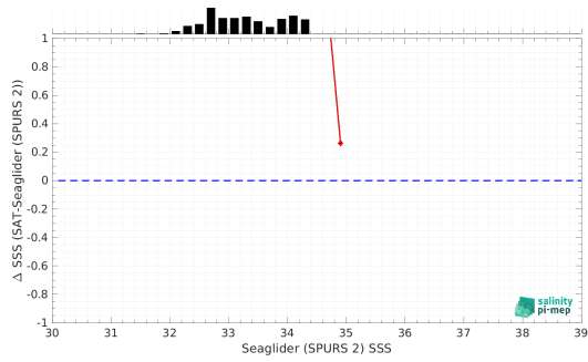
(a) Seaglider (SPURS 2) SSS
