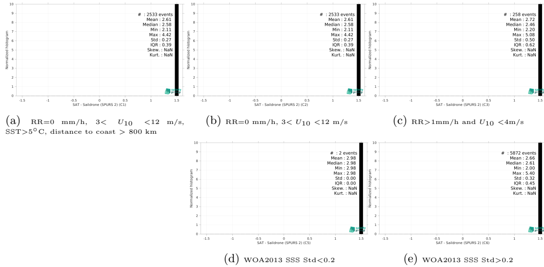
Figure 15: Normalized histogram of \Delta SSS (SMOS SSS L4 v1 - Daily (CMEMS-CNR) - Saildrone (SPURS 2)) for 5 different subdatasets corresponding to: RR=0 mm/h, 3 < U_{10} < 12 m/s, SST >5^{\circ} C, distance to coast > 800 km (a), RR=0 mm/h, 3 < U_{10} < 12 m/s (b), RR >1 mm/h and U_{10} < 4 m/s (c), WOA2013 SSS Std <0.2 (d), WOA2013 SSS Std >0.2 (e).
