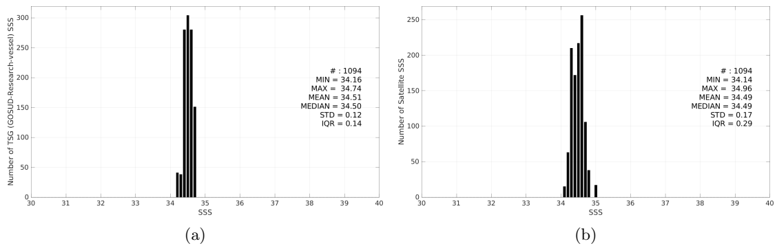
Figure 3: Histograms of SSS from TSG (GOSUD-Research-vessel) (a) and SMOS SSS L4 OI v346 - Weekly (CMEMS-CATDS-LOPS) (b) considering all match-up pairs per bins of 0.1 over the SPURS 2 Pi-MEP region and for the full satellite product period.
