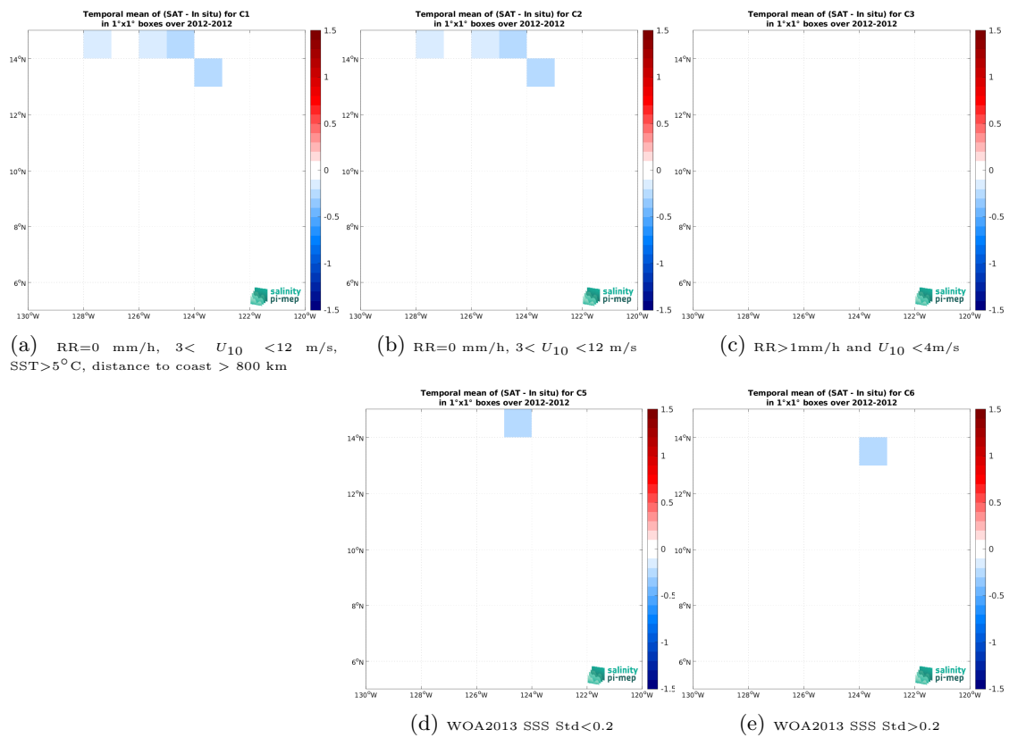
Figure 14: Temporal mean gridded over spatial boxes of size 1^\circ \times 1^\circ of \Delta SSS (SMOS SSS L4 OI v346 - Weekly (CMEMS-CATDS-LOPS) - TSG (GOSUD-Research-vessel)) for 5 different subdatasets corresponding to:RR=0 mm/h, 3 < U_{10} < 12 m/s, SST>5°C, distance to coast > 800 km (a), RR=0 mm/h, 3 < U_{10} < 12 m/s (b), RR>1mm/h and U_{10} < 4 m/s (c), WOA2013 SSS Std<0.2 (d), WOA2013 SSS Std>0.2 (e).
