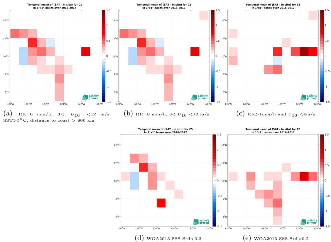
Figure 14: Temporal mean gridded over spatial boxes of size 1^\circ \times 1^\circ of \Delta\text{SSS} (SMOS SSS L4 OI v346 - Weekly (CMEMS-CATDS-LOPS) - Salinity Snake (SPURS 2)) for 5 different subdatasets corresponding to: RR=0 mm/h, 3 < U_{10} < 12 m/s, SST > 5^\circ\text{C} , distance to coast > 800 km (a), RR=0 mm/h, 3 < U_{10} < 12 m/s (b), RR > 1 mm/h and U_{10} < 4 m/s (c), WOA2013 SSS Std < 0.2 (d), WOA2013 SSS Std > 0.2 (e).
