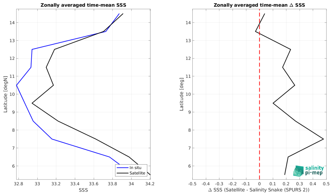
Figure 9: Left panel: Zonal mean SSS from SMOS SSS L4 OI v346 - Weekly (CMEMS-CATDS-LOPS) satellite product (black) and from Salinity Snake (SPURS 2) (blue). Right panel: Zonal mean of \Delta SSS (Satellite - Salinity Snake (SPURS 2)) for all the collected Pi-MEP match-up pairs estimated over the full satellite product period.
