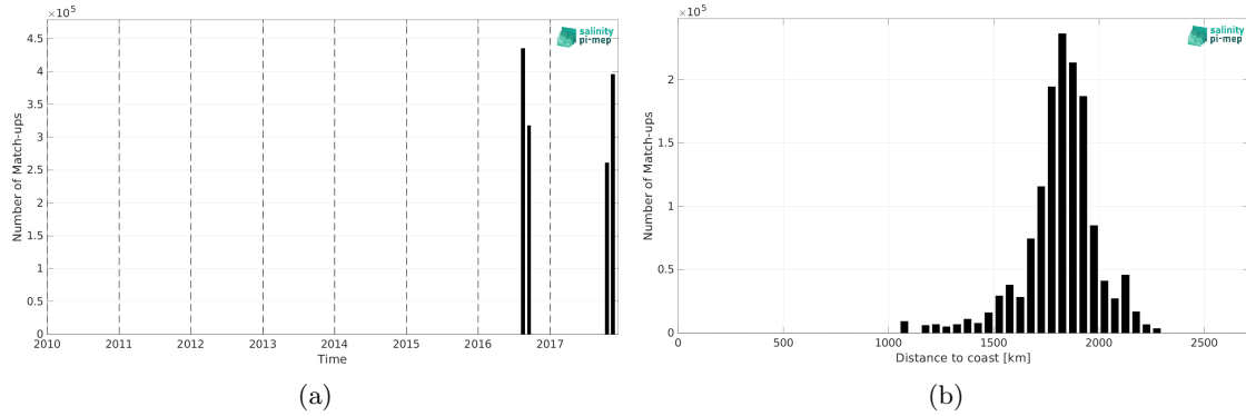
Figure 2: Number of match-ups between Salinity Snake (SPURS 2) and SMOS SSS L4 OI v346 - Weekly (CMEMS-CATDS-LOPS) SSS as a function of time (a) and as function of the distance to coast (b) over the SPURS 2 Pi-MEP region and for the full satellite product period.
