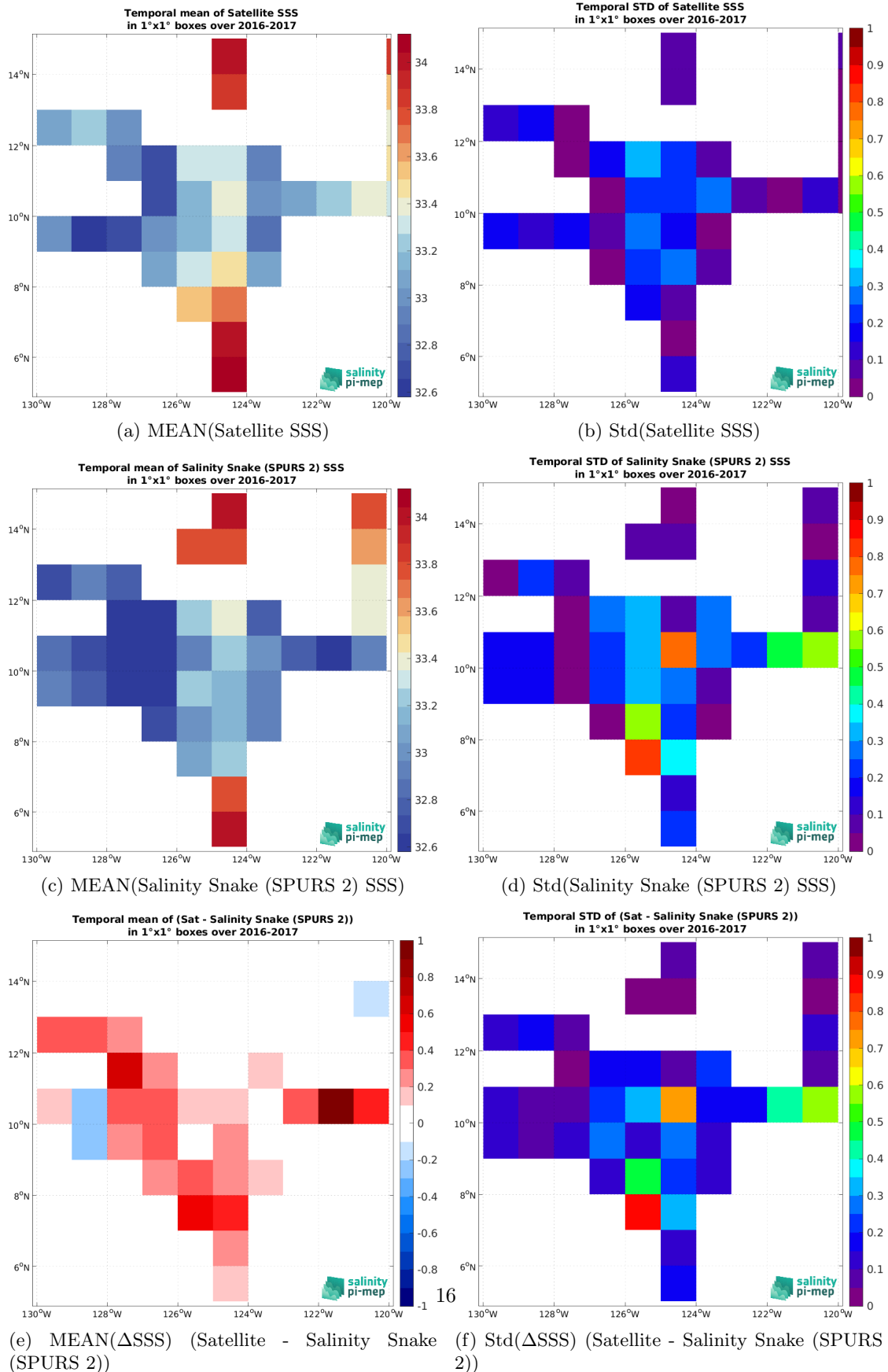
Figure 7: Temporal mean (left) and Std (right) of SSS from SMOS SSS L4 OI v346 - Weekly (CMEMS-CATDS-LOPS) (top), Salinity Snake (SPURS 2) (middle), and of \Delta SSS (Satellite - Salinity Snake (SPURS 2)). Only match-up pairs are used to generate these maps.
