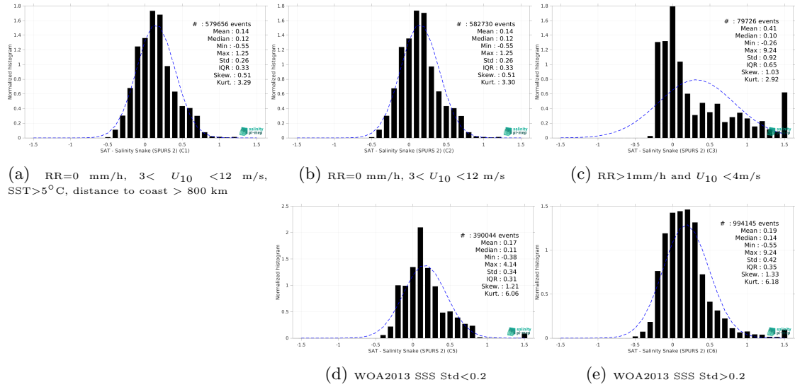
Figure 15: Normalized histogram of \Delta SSS (SMOS SSS L4 OI v346 - Weekly (CMEMS-CATDS-LOPS) - Salinity Snake (SPURS 2)) for 5 different subdatasets corresponding to: RR=0 mm/h, 3 < U_{10} < 12 m/s, SST>5°C, distance to coast > 800 km (a), RR=0 mm/h, 3 < U_{10} < 12 m/s (b), RR>1mm/h and U_{10} < 4 m/s (c), WOA2013 SSS Std<0.2 (d), WOA2013 SSS Std>0.2 (e).
