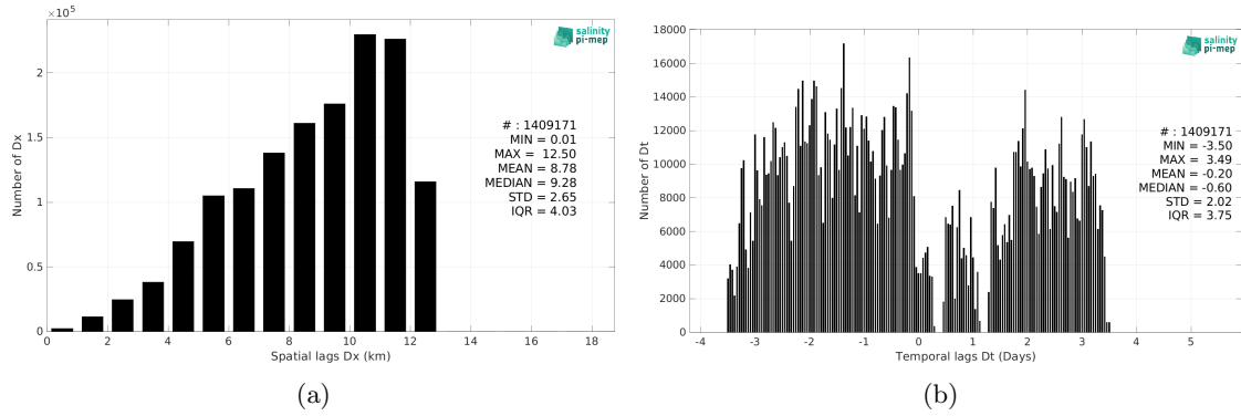
Figure 6: Histograms of the spatial (a) and temporal (b) lags between the location/time of the Salinity Snake (SPURS 2) measurement and the date of the corresponding SMOS SSS L4 OI v346 - Weekly (CMEMS-CATDS-LOPS) SSS pixel.
