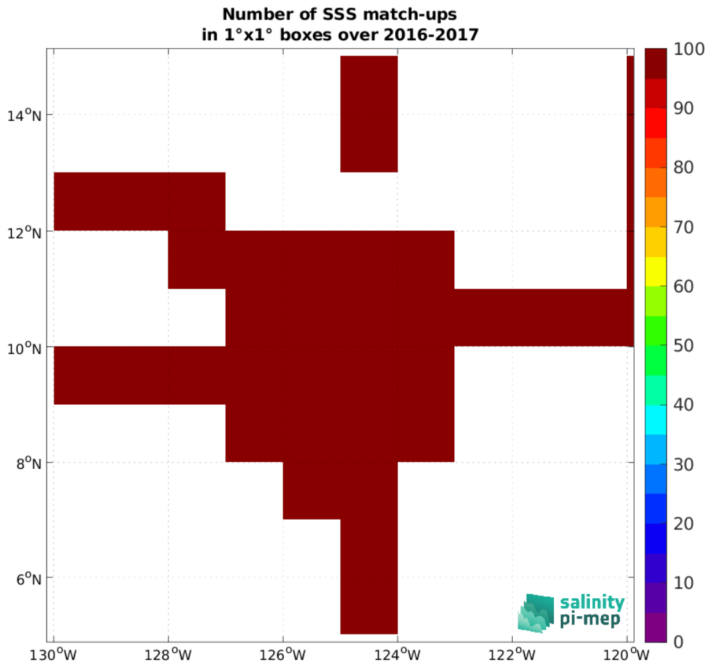
Figure 5: Number of SSS match-ups between Salinity Snake (SPURS 2) SSS and the SMOS SSS L4 OI v346 - Weekly (CMEMS-CATDS-LOPS) SSS product for the SPURS 2 Pi-MEP region over 1^\circ \times 1^\circ boxes and for the full satellite product period.
