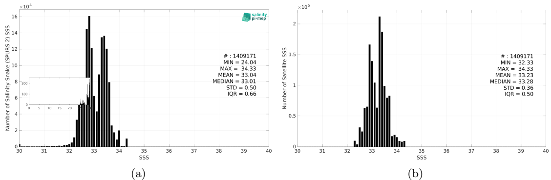
Figure 3: Histograms of SSS from Salinity Snake (SPURS 2) (a) and SMOS SSS L4 OI v346 - Weekly (CMEMS-CATDS-LOPS) (b) considering all match-up pairs per bins of 0.1 over the SPURS 2 Pi-MEP region and for the full satellite product period.
