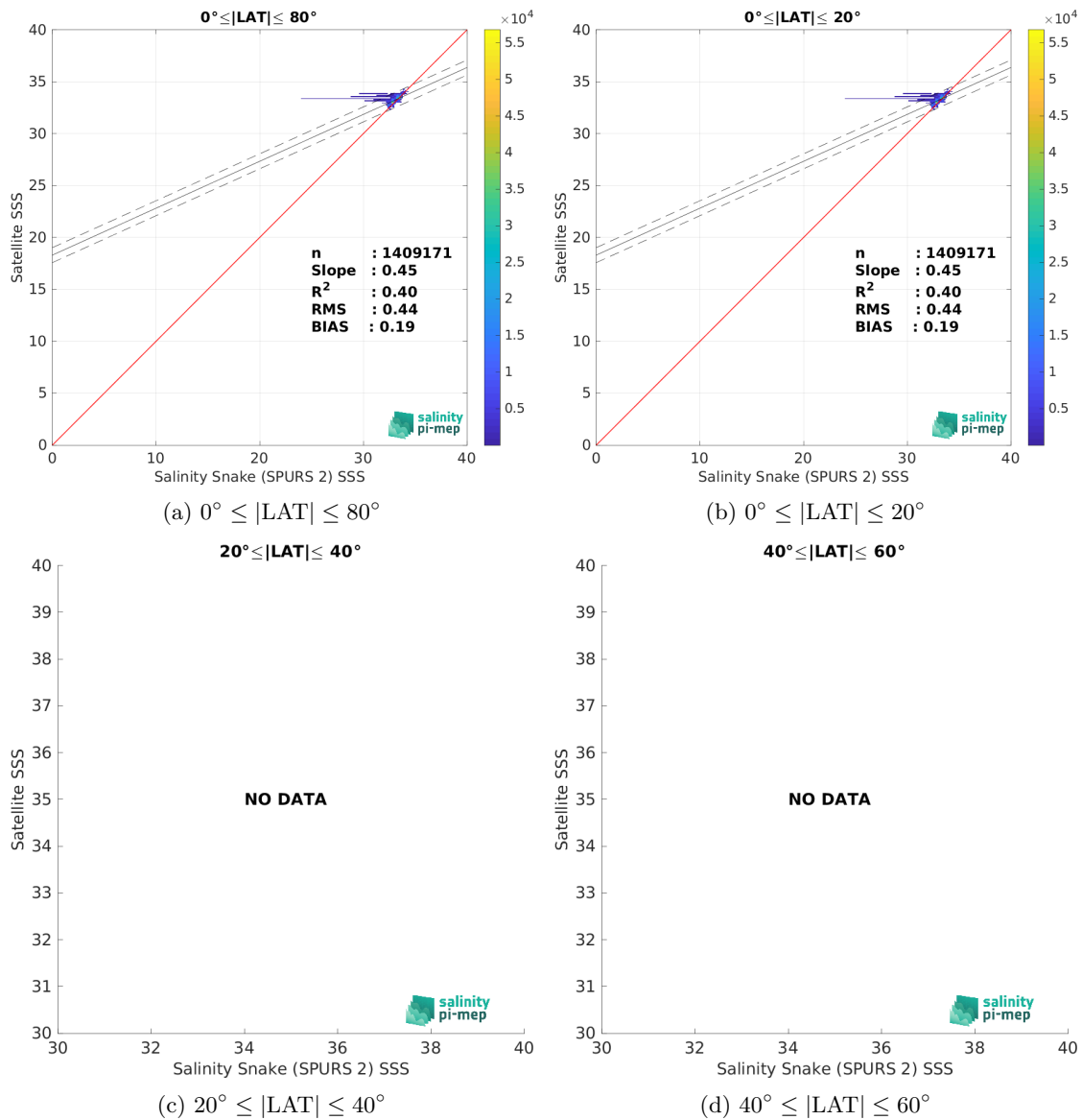
Figure 10: Contour maps of the concentration of SMOS SSS L4 OI v346 - Weekly (CMEMS-CATDS-LOPS) SSS (y-axis) versus Salinity Snake (SPURS 2) SSS (x-axis) at match-up pairs for different latitude bands. For each plot, the red line shows x=y . The black thin and dashed lines indicate a linear fit through the data cloud and the \pm 95\% confidence levels, respectively. The number match-up pairs n , the slope and R^2 coefficient of the linear fit, the root mean square (RMS) and the mean bias between satellite and in situ data are indicated for each latitude band in each plots.
