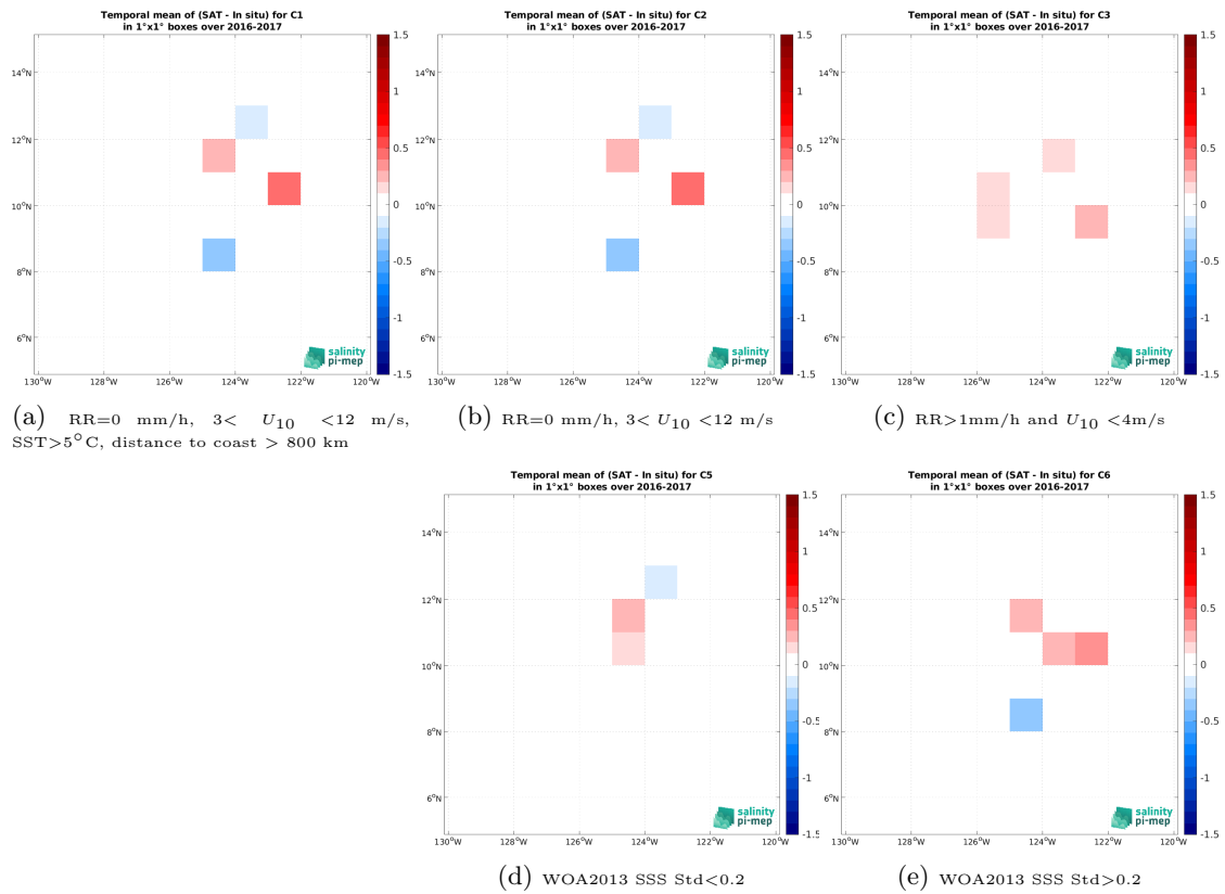
Figure 14: Temporal mean gridded over spatial boxes of size 1^\circ \times 1^\circ of \Delta SSS (SMOS SSS L4 OI v346 - Weekly (CMEMS-CATDS-LOPS) - Seaglider (SPURS 2)) for 5 different subdatasets corresponding to:RR=0 mm/h, 3 < U_{10} < 12 m/s, SST >5^\circ C, distance to coast > 800 km (a), RR=0 mm/h, 3 < U_{10} < 12 m/s (b), RR >1 mm/h and U_{10} < 4 m/s (c), WOA2013 SSS Std <0.2 (d), WOA2013 SSS Std >0.2 (e).
