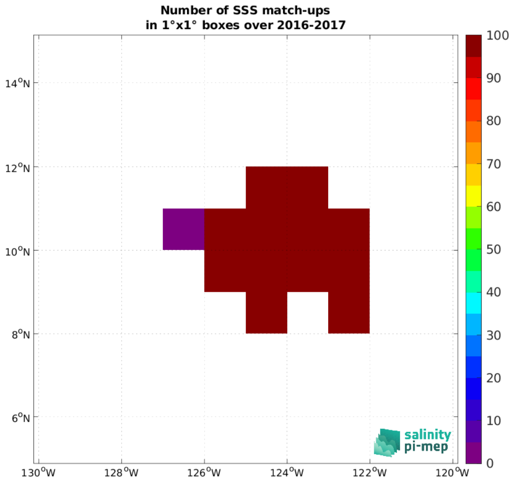
Figure 5: Number of SSS match-ups between Seaglider (SPURS 2) SSS and the SMOS SSS L4 OI v346 - Weekly (CMEMS-CATDS-LOPS) SSS product for the SPURS 2 Pi-MEP region over 1^\circ \times 1^\circ boxes and for the full satellite product period.
