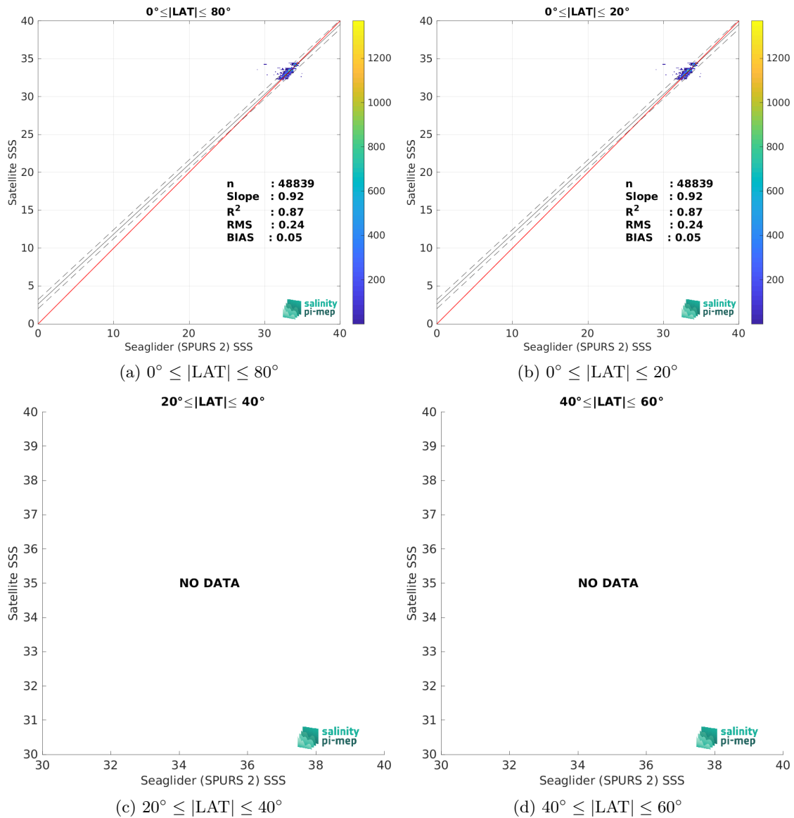
Figure 10: Contour maps of the concentration of SMOS SSS L4 OI v346 - Weekly (CMEMS-CATDS-LOPS) SSS (y-axis) versus Seaglider (SPURS 2) SSS (x-axis) at match-up pairs for different latitude bands. For each plot, the red line shows x=y . The black thin and dashed lines indicate a linear fit through the data cloud and the \pm 95\% confidence levels, respectively. The number match-up pairs n , the slope and R^2 coefficient of the linear fit, the root mean square (RMS) and the mean bias between satellite and in situ data are indicated for each latitude band in each plots.
