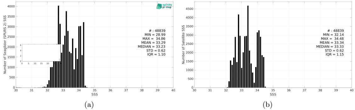
Figure 3: Histograms of SSS from Seaglider (SPURS 2) (a) and SMOS SSS L4 OI v346 - Weekly (CMEMS-CATDS-LOPS) (b) considering all match-up pairs per bins of 0.1 over the SPURS 2 Pi-MEP region and for the full satellite product period.
