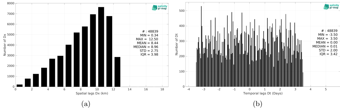
Figure 6: Histograms of the spatial (a) and temporal (b) lags between the location/time of the Seaglider (SPURS 2) measurement and the date of the corresponding SMOS SSS L4 OI v346 - Weekly (CMEMS-CATDS-LOPS) SSS pixel.
