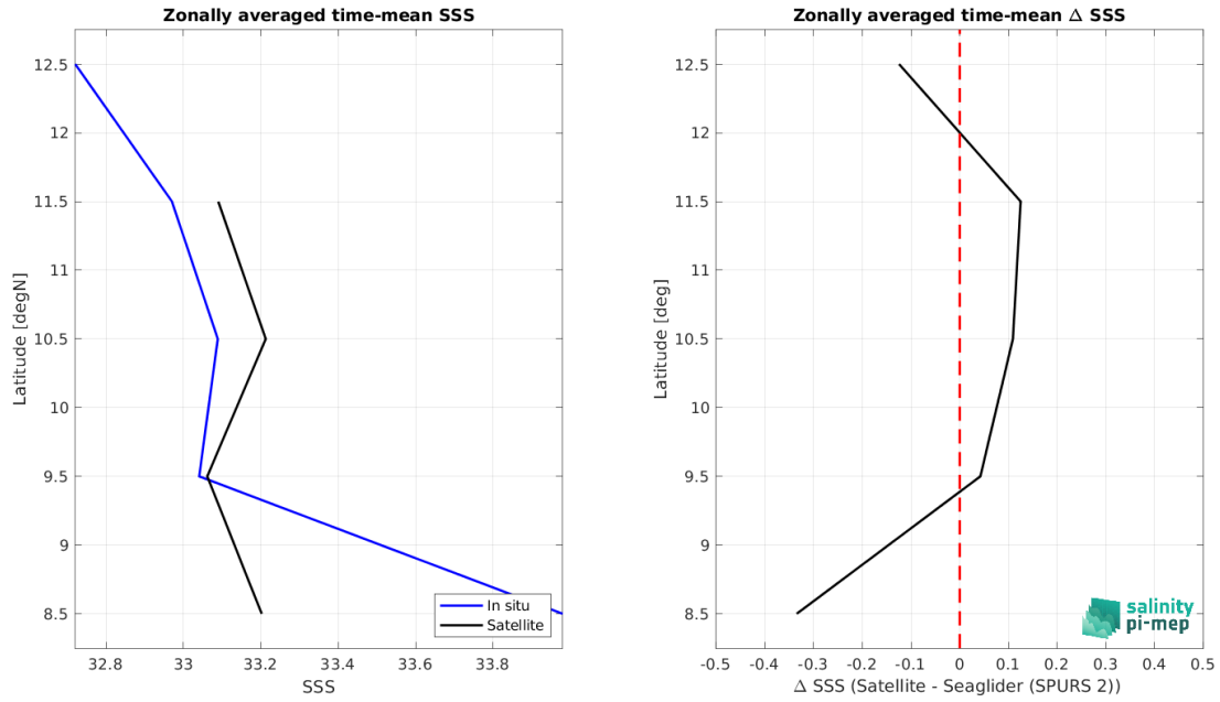
Figure 9: Left panel: Zonal mean SSS from SMOS SSS L4 OI v346 - Weekly (CMEMS-CATDS-LOPS) satellite product (black) and from Seaglider (SPURS 2) (blue). Right panel: Zonal mean of \Delta SSS (Satellite - Seaglider (SPURS 2)) for all the collected Pi-MEP match-up pairs estimated over the full satellite product period.
