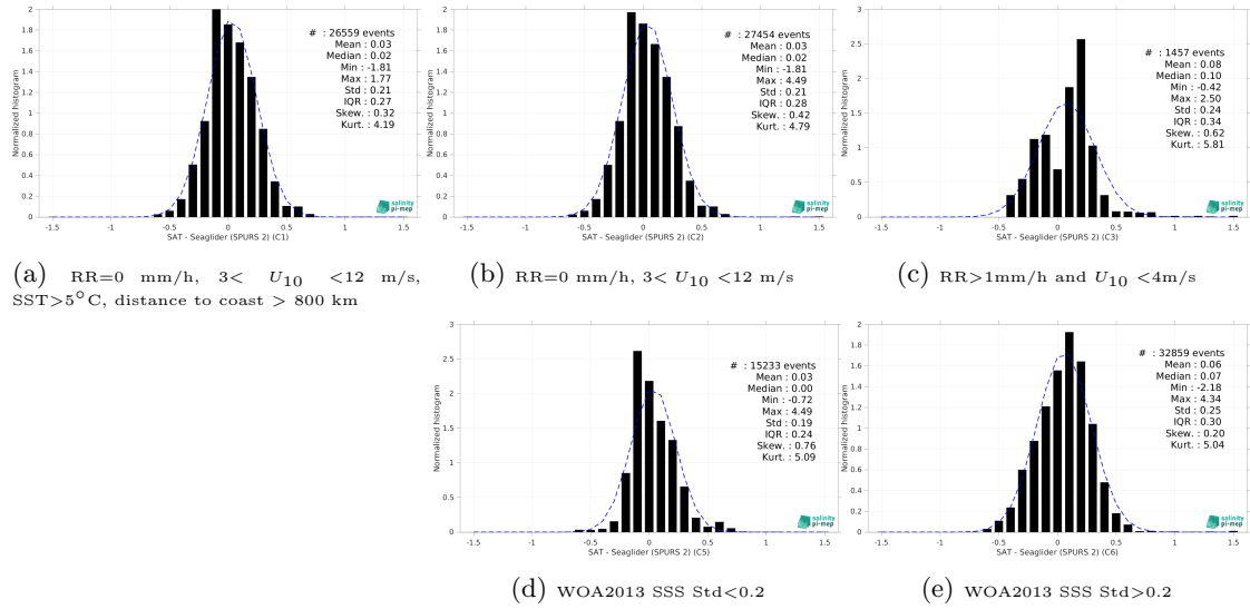
Figure 15: Normalized histogram of \Delta SSS (SMOS SSS L4 OI v346 - Weekly (CMEMS-CATDS-LOPS) - Seaglider (SPURS 2)) for 5 different subdatasets corresponding to: RR=0 mm/h, 3 < U_{10} < 12 m/s, SST>5°C, distance to coast > 800 km (a), RR=0 mm/h, 3 < U_{10} < 12 m/s (b), RR>1mm/h and U_{10} < 4 m/s (c), WOA2013 SSS Std<0.2 (d), WOA2013 SSS Std>0.2 (e).
