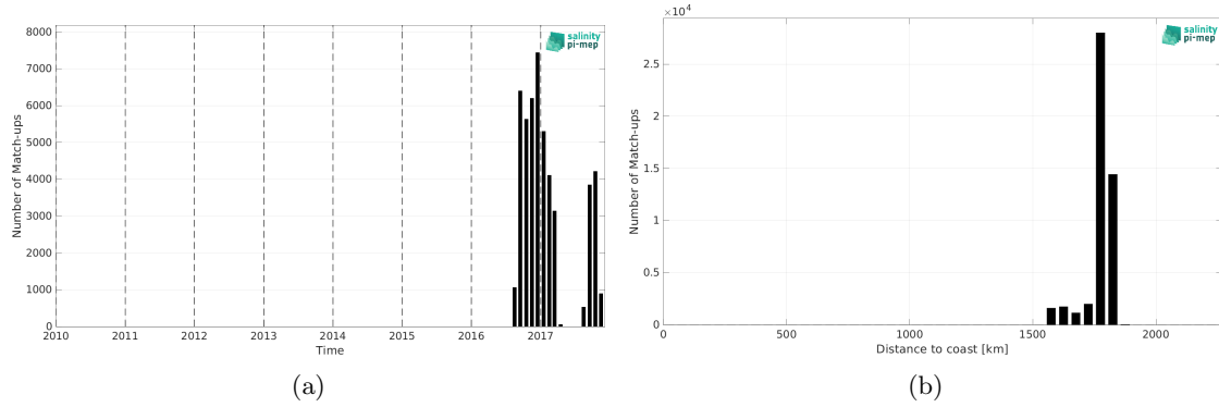
Figure 2: Number of match-ups between Seaglider (SPURS 2) and SMOS SSS L4 OI v346 - Weekly (CMEMS-CATDS-LOPS) SSS as a function of time (a) and as function of the distance to coast (b) over the SPURS 2 Pi-MEP region and for the full satellite product period.
