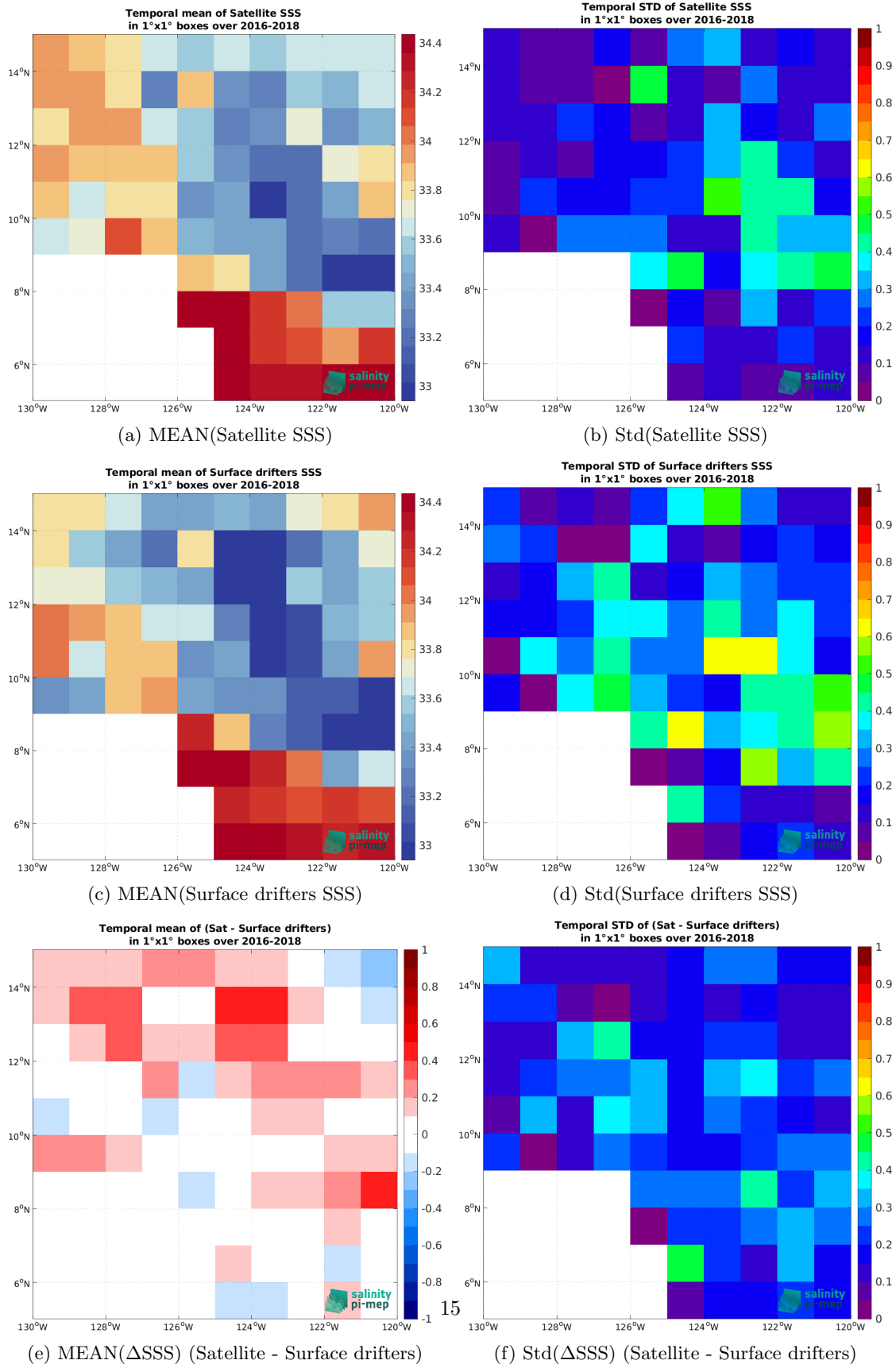
Figure 6: Temporal mean (left) and Std (right) of SSS from SMOS SSS L4 OI v346 - Weekly (CMEMS-CATDS-LOPS) (top), Surface drifters (middle), and of \Delta SSS (Satellite - Surface drifters). Only match-up pairs are used to generate these maps.
