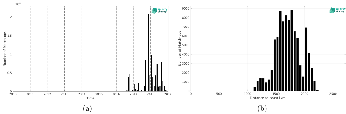
Figure 2: Number of match-ups between Surface drifters and SMOS SSS L4 OI v346 - Weekly (CMEMS-CATDS-LOPS) SSS as a function of time (a) and as function of the distance to coast (b) over the SPURS 2 Pi-MEP region and for the full satellite product period.
