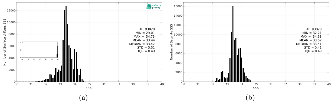
Figure 3: Histograms of SSS from Surface drifters (a) and SMOS SSS L4 OI v346 - Weekly (CMEMS-CATDS-LOPS) (b) considering all match-up pairs per bins of 0.1 over the SPURS 2 Pi-MEP region and for the full satellite product period.
