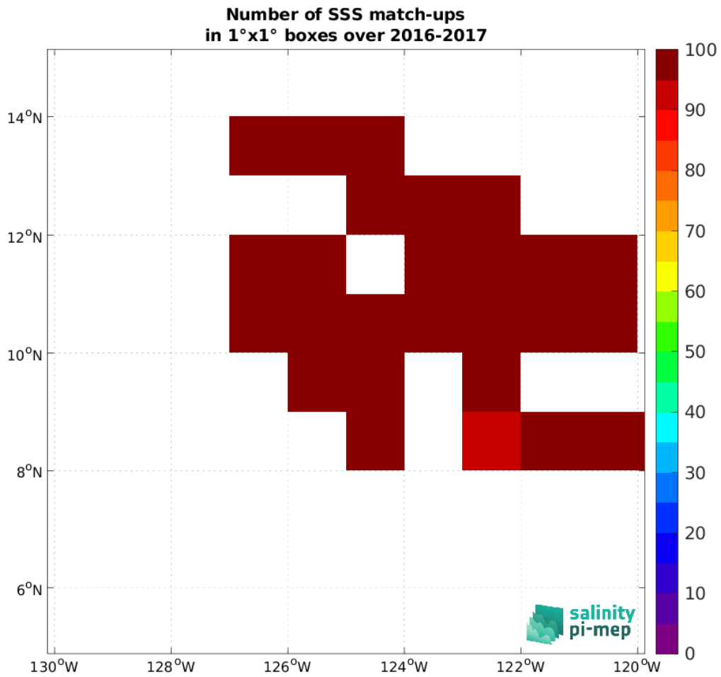
Figure 4: Number of SSS match-ups between Waveglider (SPURS 2) SSS and the SMOS SSS L4 OI v342 - Weekly (CMEMS-CATDS-LOPS) SSS product for the SPURS 2 Pi-MEP region over 1^\circ \times 1^\circ boxes and for the full satellite product period.
