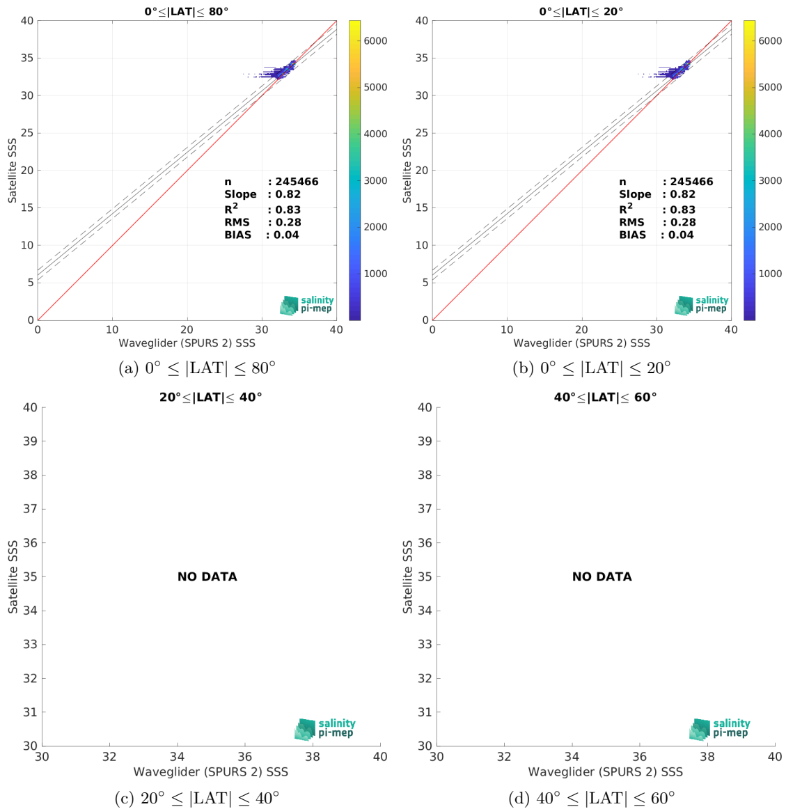
Figure 9: Contour maps of the concentration of SMOS SSS L4 OI v342 - Weekly (CMEMS-CATDS-LOPS) SSS (y-axis) versus Waveglider (SPURS 2) SSS (x-axis) at match-up pairs for different latitude bands. For each plot, the red line shows x=y . The black thin and dashed lines indicate a linear fit through the data cloud and the \pm 95\% confidence levels, respectively. The number match-up pairs n , the slope and R^2 coefficient of the linear fit, the root mean square (RMS) and the mean bias between satellite and in situ data are indicated for each latitude band in each plots.
