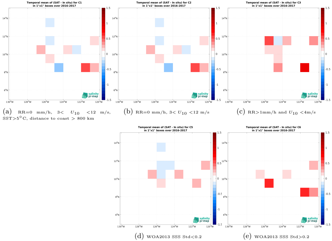
Figure 12: Temporal mean gridded over spatial boxes of size 1^{\circ}\times 1^{\circ} of \Delta\text{SSS} (SMOS SSS L4 OI v342 - Weekly (CMEMS-CATDS-LOPS) - Waveglider (SPURS 2)) for 5 different subdatasets corresponding to:RR=0 mm/h, 3 < U_{10} < 12 m/s, SST >5^{\circ}\text{C} , distance to coast > 800 km (a), RR=0 mm/h, 3 < U_{10} < 12 m/s (b), RR >1 mm/h and U_{10} < 4 m/s (c), WOA2013 SSS Std <0.2 (d), WOA2013 SSS Std >0.2 (e).
