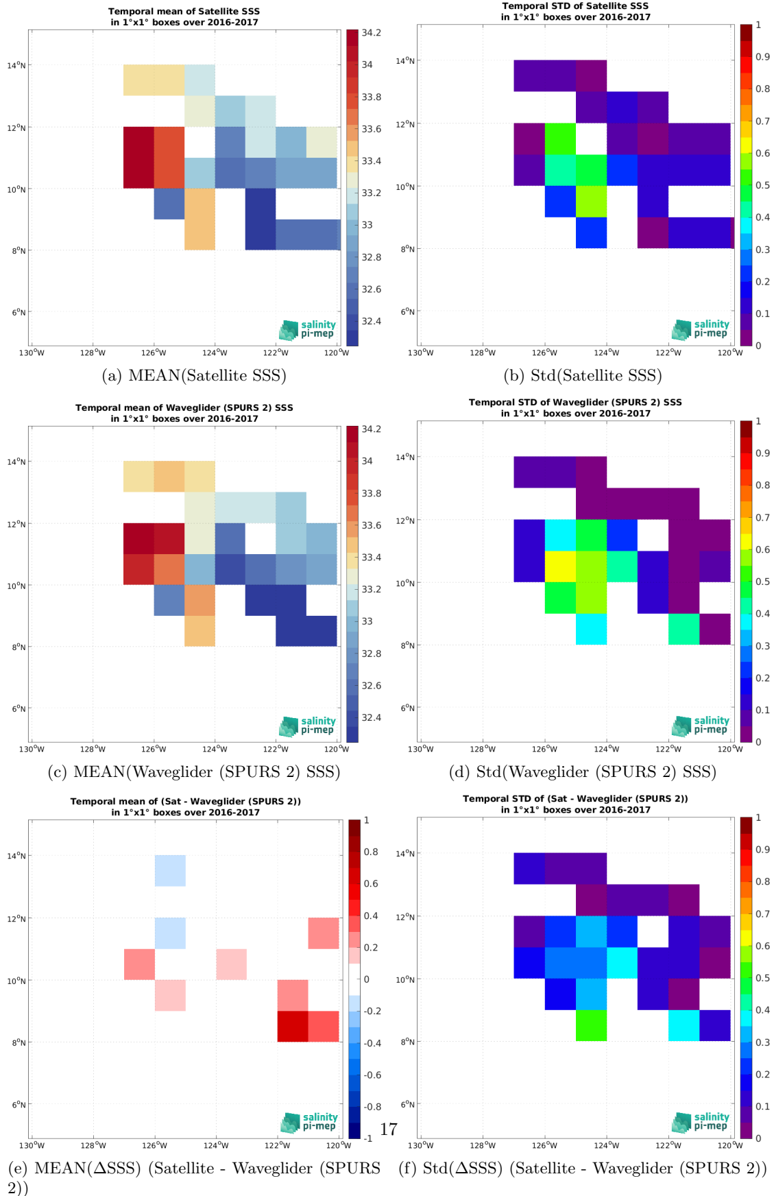
Figure 6: Temporal mean (left) and Std (right) of SSS from SMOS SSS L4 OI v342 - Weekly (CMEMS-CATDS-LOPS) (top), Waveglider (SPURS 2) (middle), and of \Delta SSS (Satellite - Waveglider (SPURS 2)). Only match-up pairs are used to generate these maps.
