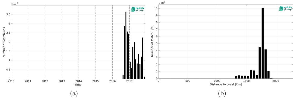
Figure 1: Number of match-ups between Waveglider (SPURS 2) and SMOS SSS L4 OI v342 - Weekly (CMEMS-CATDS-LOPS) SSS as a function of time (a) and as function of the distance to coast (b) over the SPURS 2 Pi-MEP region and for the full satellite product period.
