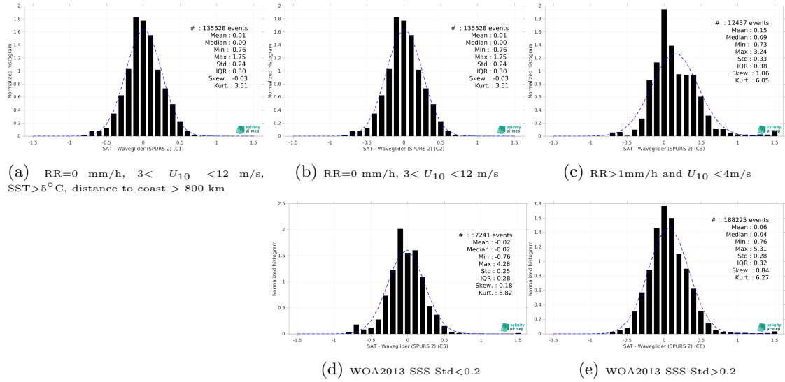
Figure 13: Normalized histogram of \Delta SSS (SMOS SSS L4 OI v342 - Weekly (CMEMS-CATDS-LOPS) - Waveglider (SPURS 2)) for 5 different subdatasets corresponding to: RR=0 mm/h, 3 < U_{10} < 12 m/s, SST>5°C, distance to coast > 800 km (a), RR=0 mm/h, 3 < U_{10} < 12 m/s (b), RR>1mm/h and U_{10} < 4 m/s (c), WOA2013 SSS Std<0.2 (d), WOA2013 SSS Std>0.2 (e).
