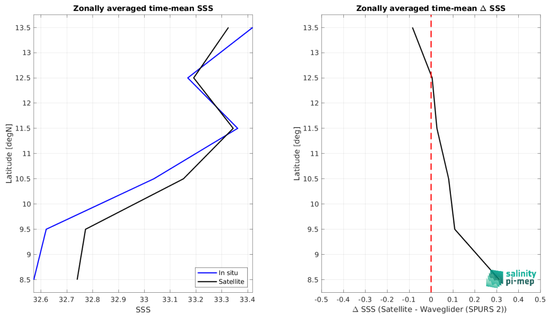
Figure 8: Left panel: Zonal mean SSS from SMOS SSS L4 OI v342 - Weekly (CMEMS-CATDS-LOPS) satellite product (black) and from Waveglider (SPURS 2) (blue). Right panel: Zonal mean of \Delta SSS (Satellite - Waveglider (SPURS 2)) for all the collected Pi-MEP match-up pairs estimated over the full satellite product period.
