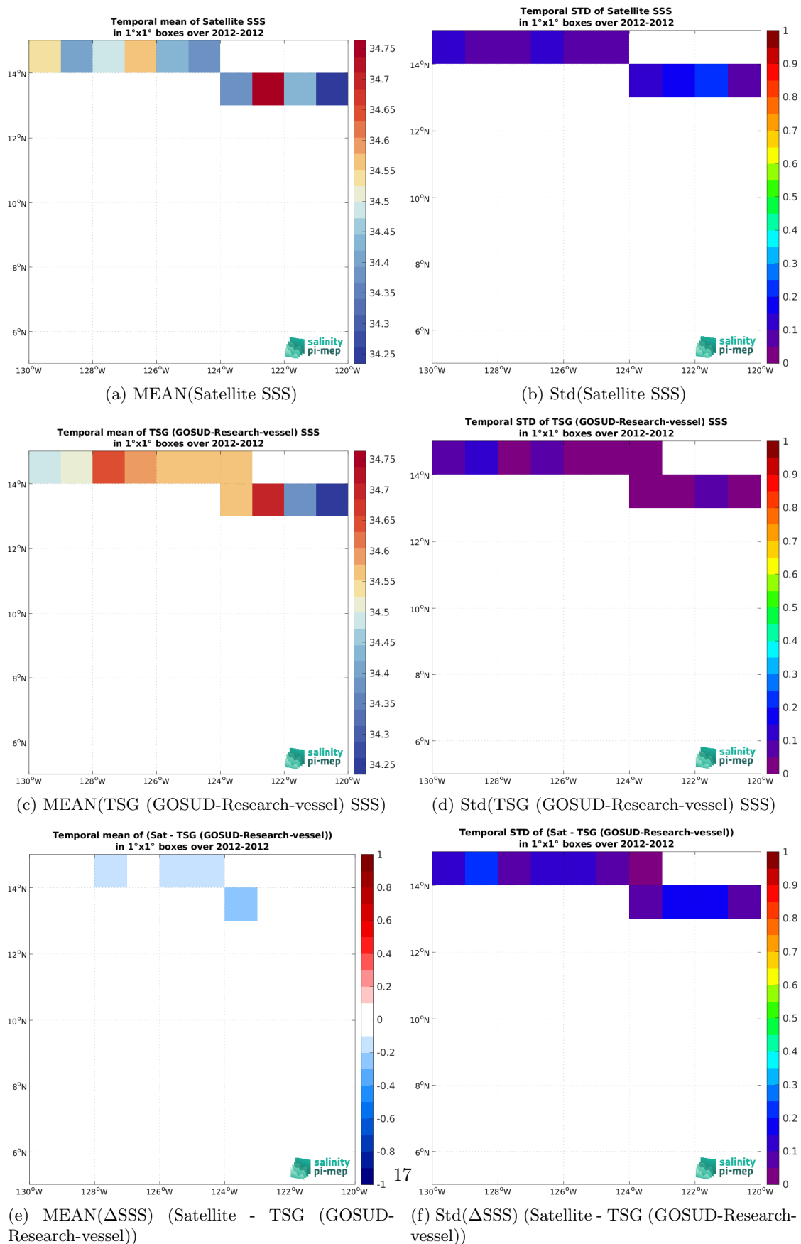
Figure 6: Temporal mean (left) and Std (right) of SSS from SMOS SSS L4 OI v342 - Weekly (CMEMS-CATDS-LOPS) (top), TSG (GOSUD-Research-vessel) (middle), and of \Delta SSS (Satellite - TSG (GOSUD-Research-vessel)). Only match-up pairs are used to generate these maps.
