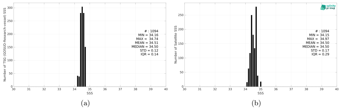
Figure 2: Histograms of SSS from TSG (GOSUD-Research-vessel) (a) and SMOS SSS L4 OI v342 - Weekly (CMEMS-CATDS-LOPS) (b) considering all match-up pairs per bins of 0.1 over the SPURS 2 Pi-MEP region and for the full satellite product period.
