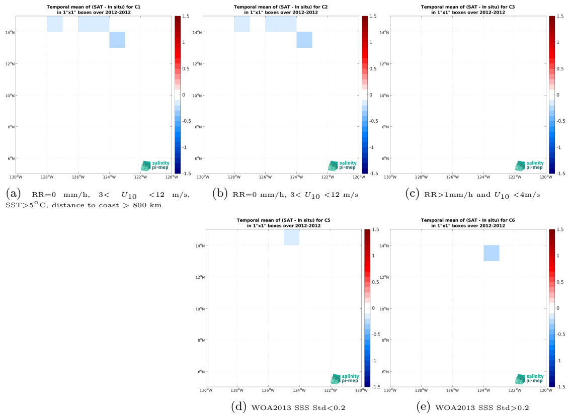
Figure 12: Temporal mean gridded over spatial boxes of size 1^\circ \times 1^\circ of \Delta SSS (SMOS SSS L4 OI v342 - Weekly (CMEMS-CATDS-LOPS) - TSG (GOSUD-Research-vessel)) for 5 different subdatasets corresponding to:RR=0 mm/h, 3 < U_{10} < 12 m/s, SST>5°C, distance to coast > 800 km (a), RR=0 mm/h, 3 < U_{10} < 12 m/s (b), RR>1mm/h and U_{10} < 4 m/s (c), WOA2013 SSS Std<0.2 (d), WOA2013 SSS Std>0.2 (e).
