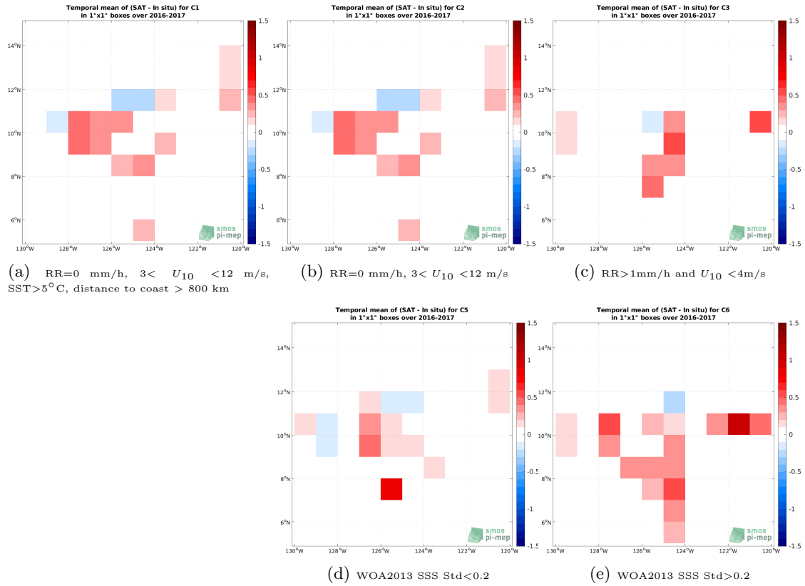
Figure 12: Temporal mean gridded over spatial boxes of size 1^{\circ} \times 1^{\circ} of \Delta\text{SSS} (SMOS SSS L4 OI v342 - Weekly (CMEMS-CATDS-LOPS) - Salinity Snake (SPURS 2)) for 5 different subdatasets corresponding to: RR=0 mm/h, 3 < U_{10} < 12 m/s, SST > 5^{\circ}\text{C} , distance to coast > 800 km (a), RR=0 mm/h, 3 < U_{10} < 12 m/s (b), RR > 1\text{mm/h} and U_{10} < 4\text{m/s} (c), WOA2013 SSS Std < 0.2 (d), WOA2013 SSS Std > 0.2 (e).
