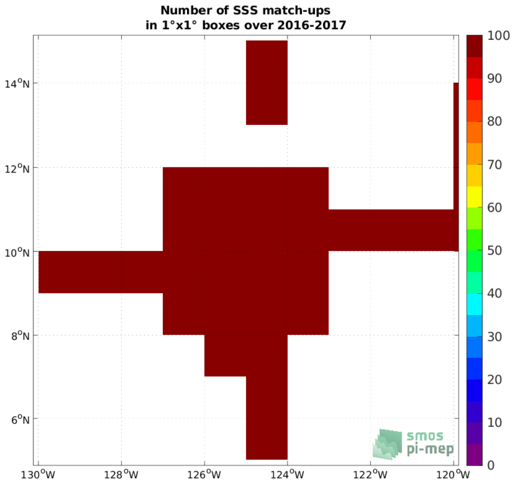
Figure 4: Number of SSS match-ups between Salinity Snake (SPURS 2) SSS and the SMOS SSS L4 OI v342 - Weekly (CMEMS-CATDS-LOPS) SSS product for the SPURS 2 Pi-MEP region over 1°x1° boxes and for the full satellite product period.
