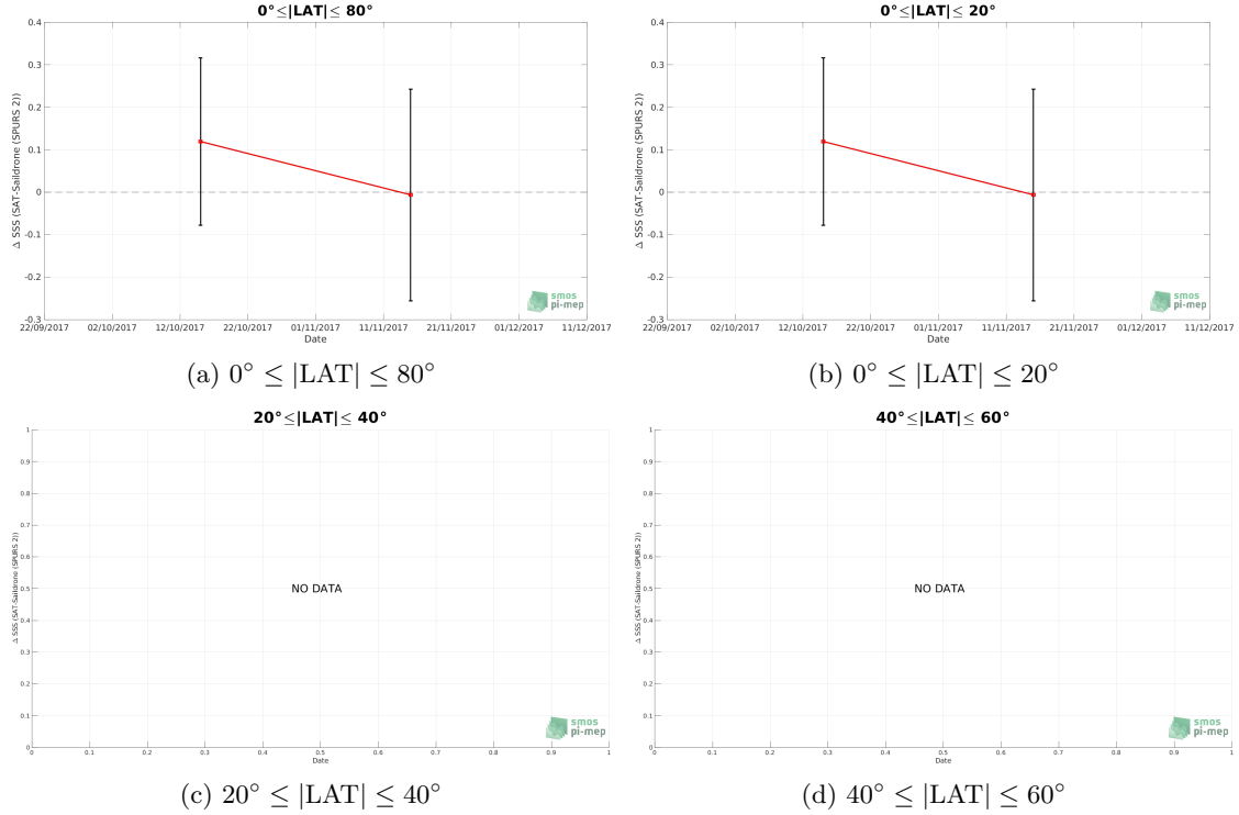
Figure 10: Monthly median (red curves) of \Delta SSS (Satellite - Sailerone (SPURS 2)) and \pm 1 Std (black vertical thick bars) as function of time for all the collected Pi-MEP match-up pairs estimated over the SPURS 2 Pi-MEP region and for the full satellite product period are shown for different latitude bands: (a) 80^\circ\text{S}-80^\circ\text{N} , (b) 20^\circ\text{S}-20^\circ\text{N} , (c) 40^\circ\text{S}-20^\circ\text{S} and 20^\circ\text{N}-40^\circ\text{N} and (d) 60^\circ\text{S}-40^\circ\text{S} and 40^\circ\text{N}-60^\circ\text{N} .
