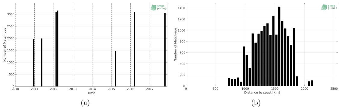
Figure 1: Number of match-ups between TSG-SAMOS and SMOS-L4-CATDS-CECOS-IFREMER-V2-WEEKLY-0.5DEG SSS as a function of time (a) and as function of the distance to coast (b) over the SPURS 2 Pi-MEP region and for the full satellite product period.
