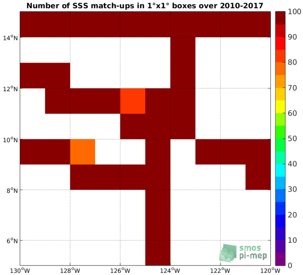
Figure 4: Number of SSS match-ups between TSG-SAMOS SSS and the SMOS-L4-CATDS-CECOS-IFREMER-V2-WEEKLY-0.5DEG SSS product for the SPURS 2 Pi-MEP region over 1°x1° boxes and for the full satellite product period.
