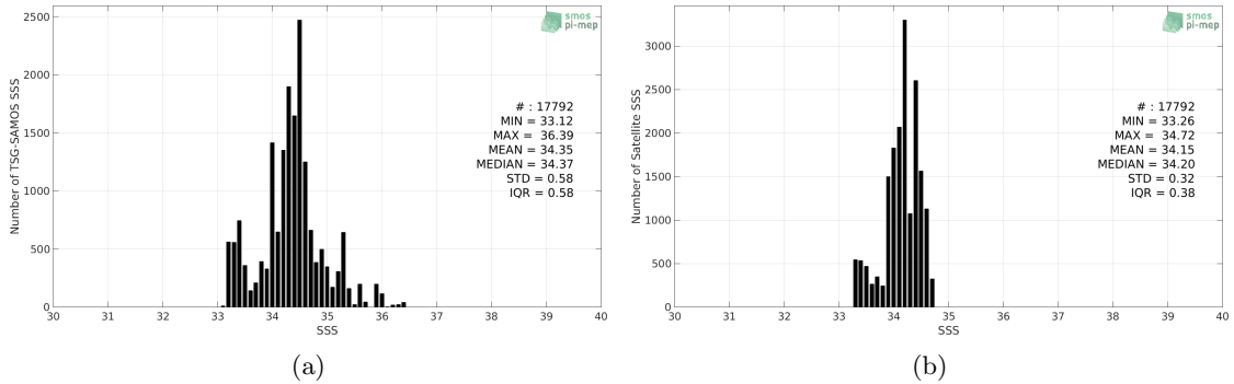
Figure 2: Histograms of SSS from TSG-SAMOS (a) and SMOS-L4-CATDS-CECOS-IFREMER-V2-WEEKLY-0.5DEG (b) considering all match-up pairs per bins of 0.1 over the SPURS 2 Pi-MEP region and for the full satellite product period.
