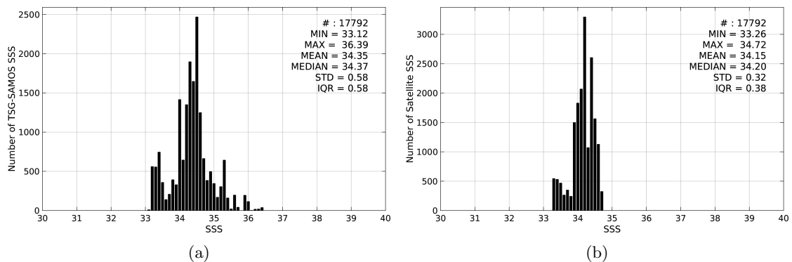
Figure 2: Histograms of SSS from TSG-SAMOS (a) and SMOS-L4-CATDS-CECOS-IFREMER-V2-WEEKLY-0.5DEG (b) considering all match-up pairs per bins of 0.1 over the SPURS 2 Pi-MEP region and for the full satellite product period.
