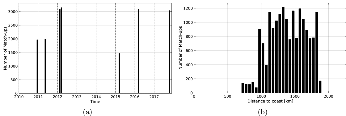
Figure 1: Number of match-ups between TSG-SAMOS and SMOS-L4-CATDS-CECOS-IFREMER-V2-WEEKLY-0.5DEG SSS as a function of time (a) and as function of the distance to coast (b) over the SPURS 2 Pi-MEP region and for the full satellite product period.
