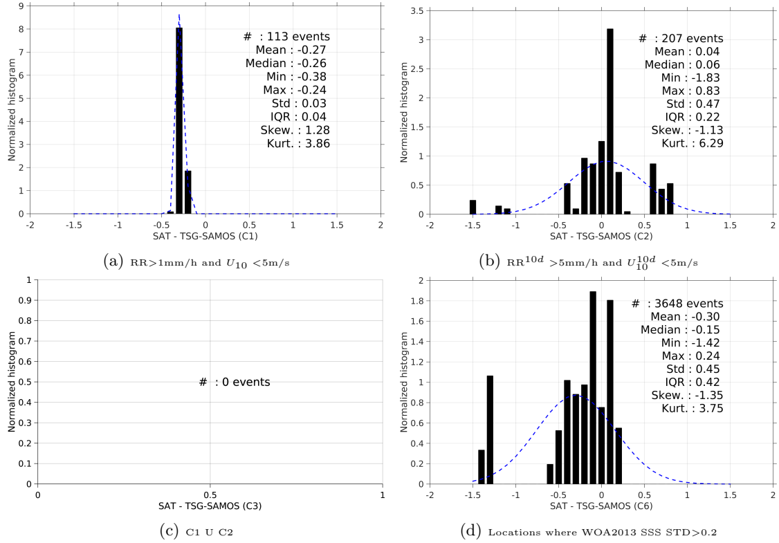
Figure 13: Normalized histogram of \Delta SSS (SMOS-L4-CATDS-CECOS-IFREMER-V2-WEEKLY-0.5DEG - TSG-SAMOS) for 6 different subdatasets corresponding to: RR > 1mm/h and U_{10} < 5 m/s (a), RR^{10d} > 5 mm/h and U_{10}^{10d} < 5 m/s (b), C1 U C2 (c), Locations where WOA2013 SSS STD > 0.2 (d).
