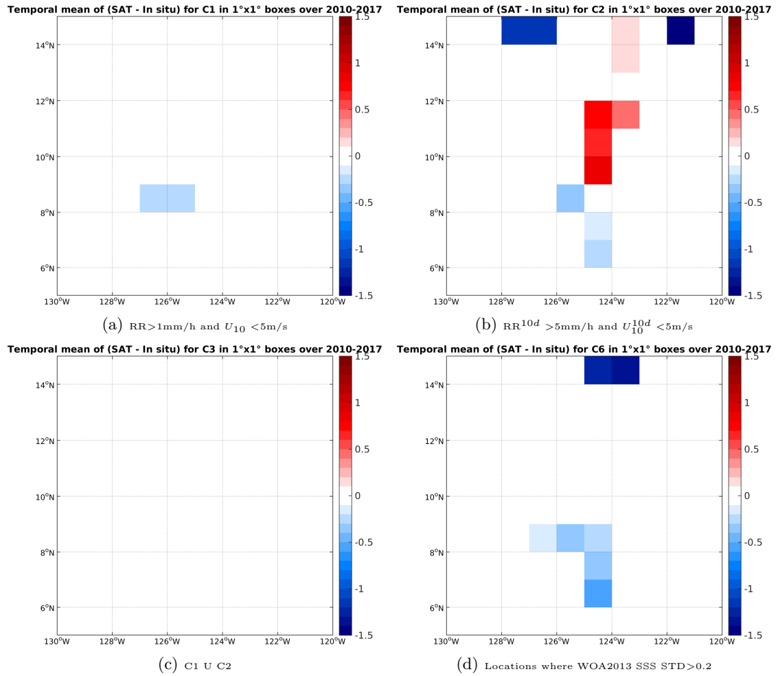
Figure 12: Temporal mean gridded over spatial boxes of size 1°x1° of \Delta SSS (SMOS-L4-CATDS-CECOS-IFREMER-V2-WEEKLY-0.5DEG - TSG-SAMOS) for 4 different subdatasets corresponding to: RR > 1mm/h and U_{10} < 5\text{m/s} (a), RR^{10d} > 5\text{mm/h} and U_{10}^{10d} < 5\text{m/s} (b), C1 U C2 (c), Locations where WOA2013 SSS STD > 0.2 (d).
