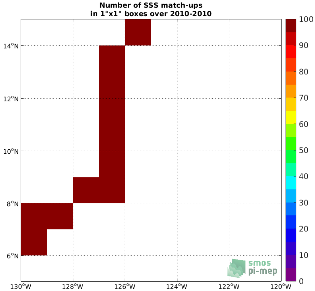
Figure 4: Number of SSS match-ups between TSG (GOSUD-Sailing-ship) SSS and the SMOS L4 v2 Weekly (CATDS-CECOS-IFREMER) SSS product for the SPURS 2 Pi-MEP region over 1°x1° boxes and for the full satellite product period.
