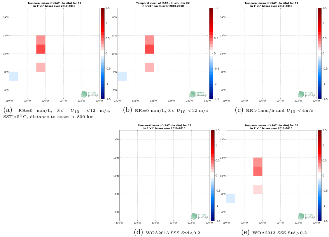
Figure 12: Temporal mean gridded over spatial boxes of size 1^\circ \times 1^\circ of \Delta SSS (SMOS L4 v2 Weekly (CATDS-CECOS-IFREMER) - TSG (GOSUD-Sailing-ship)) for 5 different subdatasets corresponding to: RR=0 mm/h, 3 < U_{10} < 12 m/s, SST>5°C, distance to coast > 800 km (a), RR=0 mm/h, 3 < U_{10} < 12 m/s (b), RR>1mm/h and U_{10} < 4 m/s (c), WOA2013 SSS Std<0.2 (d), WOA2013 SSS Std>0.2 (e).
