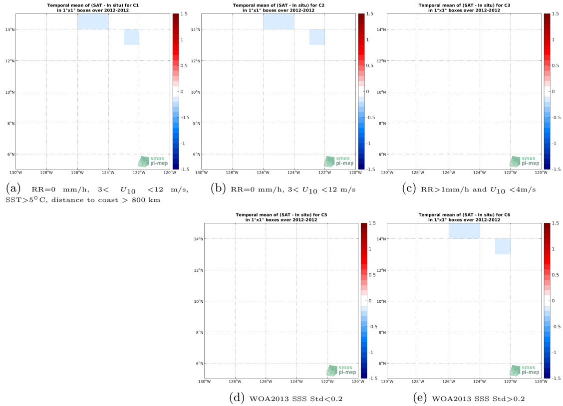
Figure 12: Temporal mean gridded over spatial boxes of size 1^\circ \times 1^\circ of \Delta SSS (SMOS L4 v2 Weekly (CATDS-CECOS-IFREMER) - TSG (GOSUD-Research-vessel)) for 5 different subdatasets corresponding to: RR=0 mm/h, 3 < U_{10} < 12 m/s, SST > 5°C, distance to coast > 800 km (a), RR=0 mm/h, 3 < U_{10} < 12 m/s (b), RR > 1mm/h and U_{10} < 4 m/s (c), WOA2013 SSS Std < 0.2 (d), WOA2013 SSS Std > 0.2 (e).
