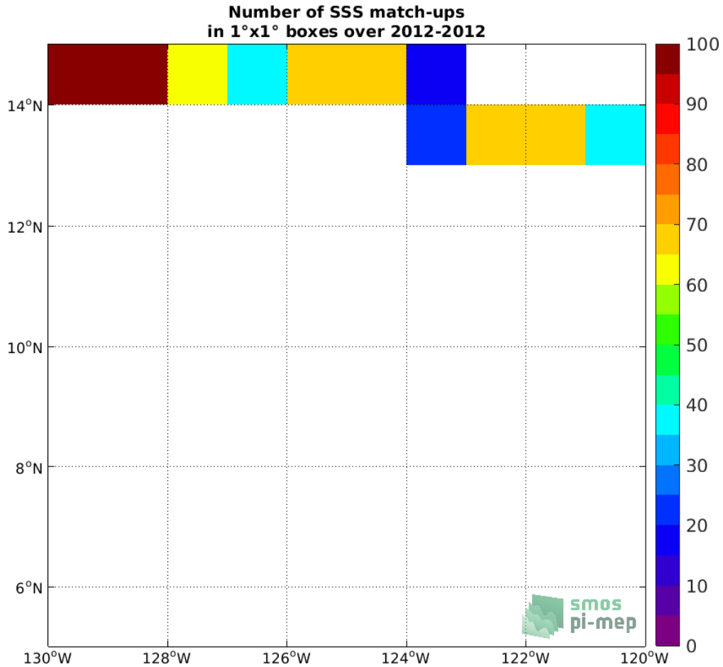
Figure 4: Number of SSS match-ups between TSG (GOSUD-Research-vessel) SSS and the SMOS L4 v2 Weekly (CATDS-CECOS-IFREMER) SSS product for the SPURS 2 Pi-MEP region over 1°x1° boxes and for the full satellite product period.
