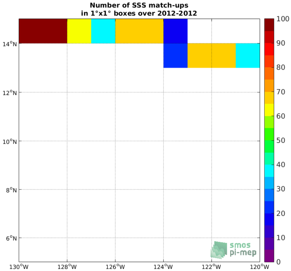
Figure 4: Number of SSS match-ups between TSG-GOSUD-Research-vessel SSS and the SMOS-L4-CATDS-CECOS-IFREMER-V2-WEEKLY-0.5DEG SSS product for the SPURS 2 Pi-MEP region over 1°x1° boxes and for the full satellite product period.
